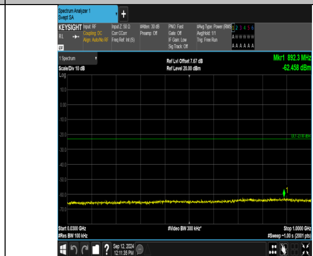
Band2_3MHz_16QAM_18615_1RB#14_30~1000_30~1000
