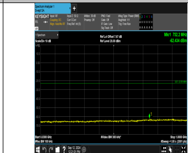
Band2_3MHz_16QAM_19185_1RB#14_30~1000_30~1000
