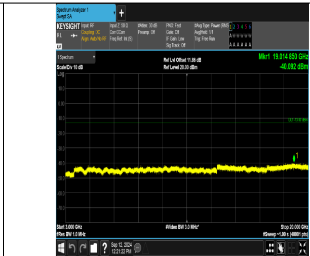
Band2_3MHz_16QAM_19185_1RB#14_3000~20000_3000~20000
