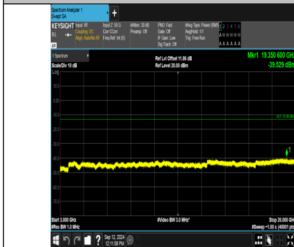
Band2_3MHz_QPSK_18615_1RB#14_3000~20000_3000~20000
