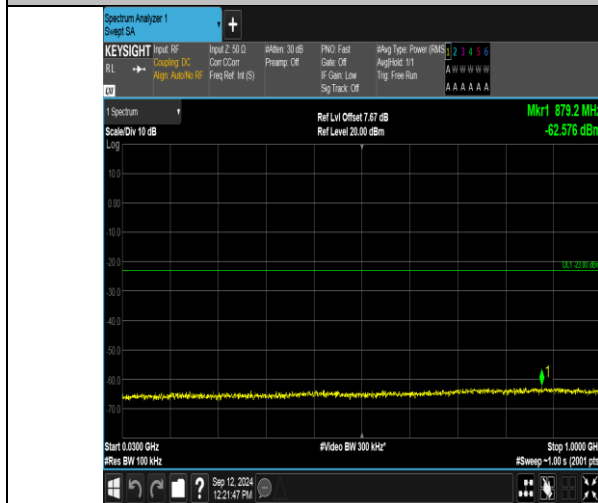
Band2_3MHz_QPSK_19185_15RB#0_30~1000_30~1000
