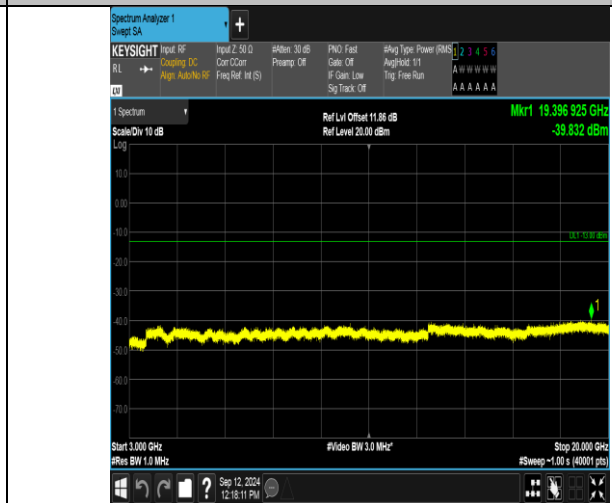
Band2_3MHz_16QAM_18900_15RB#0_3000~20000_3000~20000
