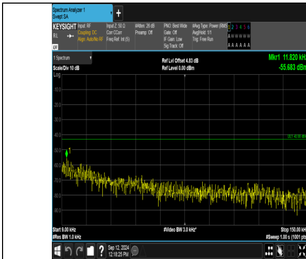
Band2_3MHz_QPSK_19185_1RB#0_0.009~0.15_0.009~0.15
