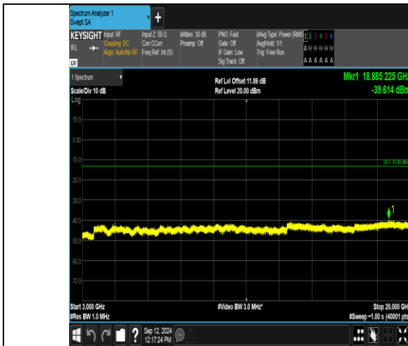
Band2_3MHz_QPSK_18900_15RB#0_3000~20000_3000~20000
