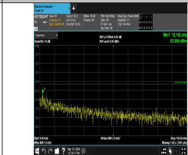
Band2_3MHz_16QAM_19185_1RB#0_0.009~0.15_0.009~0.15
