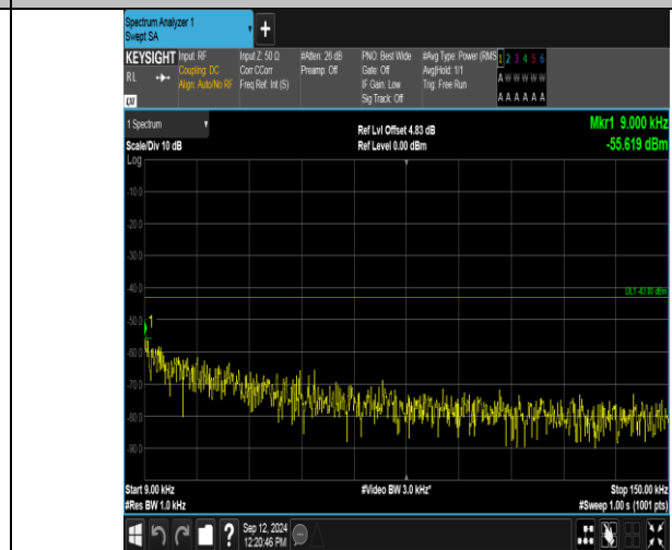
Band2_3MHz_16QAM_19185_1RB#14_0.009~0.15_0.009~0.15
