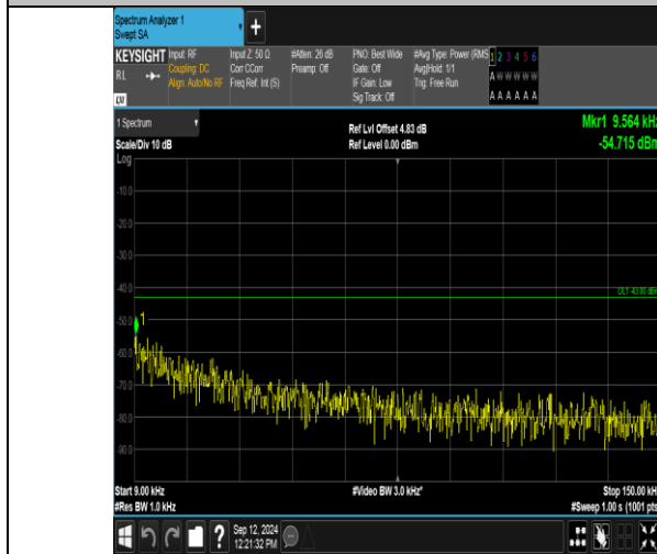
Band2_3MHz_QPSK_19185_15RB#0_0.009~0.15_0.009~0.15
