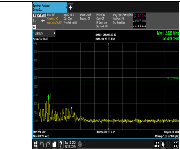
Band2_3MHz_QPSK_19185_1RB#0_0.15~30_0.15~30
