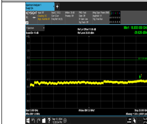
Band2_3MHz_QPSK_19185_1RB#14_3000~20000_3000~20000
