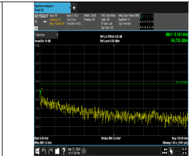
Band2_3MHz_16QAM_18900_15RB#0_0.009~0.15_0.009~0.15
