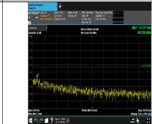
Band2_3MHz_16QAM_18615_1RB#14_0.009~0.15_0.009~0.15
