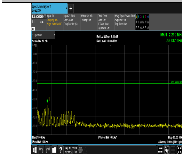
Band2_3MHz_16QAM_18615_1RB#14_0.15~30_0.15~30
