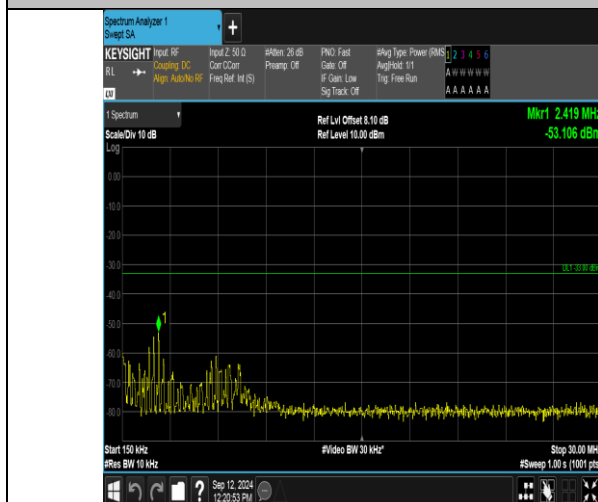
Band2_3MHz_16QAM_19185_1RB#14_0.15~30_0.15~30
