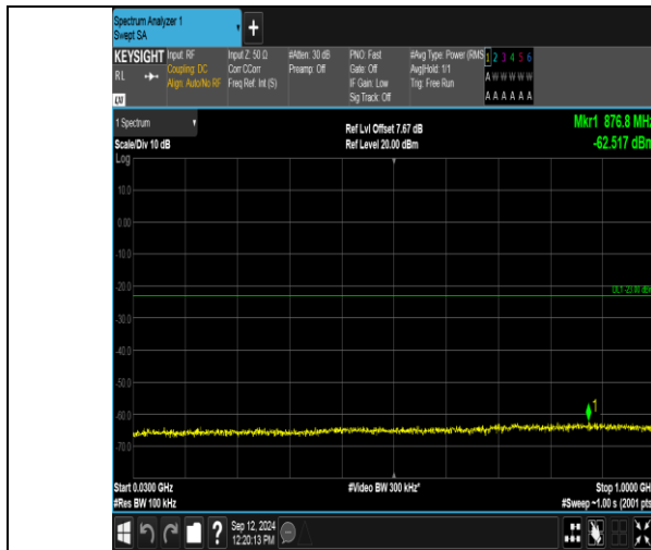
Band2_3MHz_QPSK_19185_1RB#14_30~1000_30~1000
