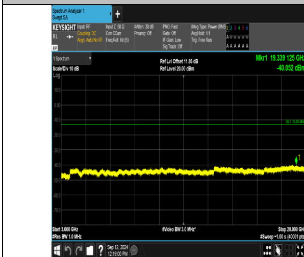
Band2_3MHz_QPSK_19185_1RB#0_3000~20000_3000~20000
