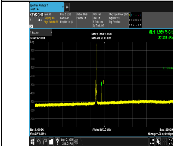
Band2_3MHz_16QAM_18900_15RB#0_1000~3000_1000~3000
