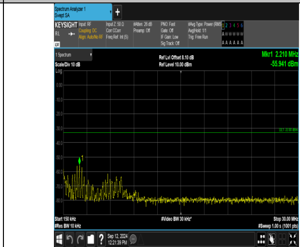
Band2_3MHz_QPSK_19185_15RB#0_0.15~30_0.15~30
