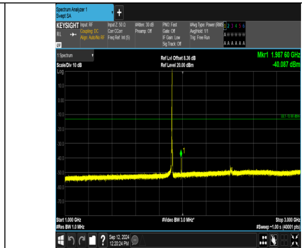
Band2_3MHz_QPSK_19185_1RB#14_1000~3000_1000~3000
