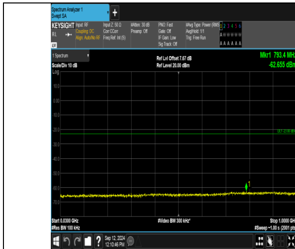
Band2_3MHz_QPSK_18615_1RB#14_30~1000_30~1000
