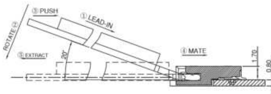
Figure 30. Angle of insertion for APCI0026-P001A
