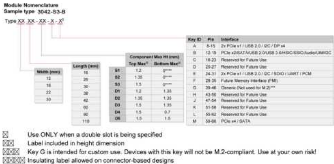
Figure 26. M.2 interface model
