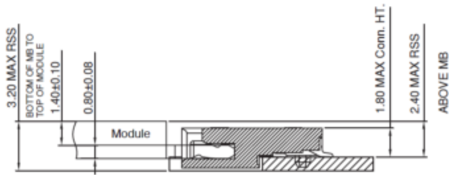
Figure 31. Stack-up mid-mount single-sided module
