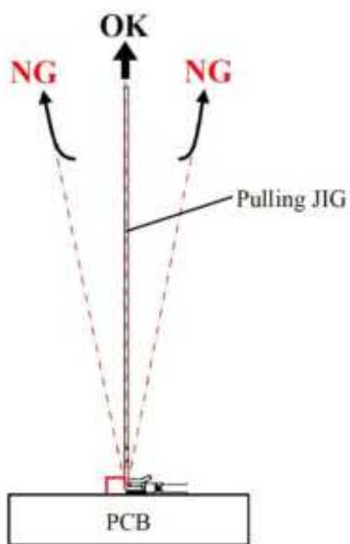
Figure 23. Pulling direction
