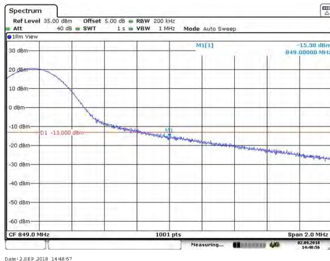
BAND 26_15MHz_64QAM_26965_75RB#0
