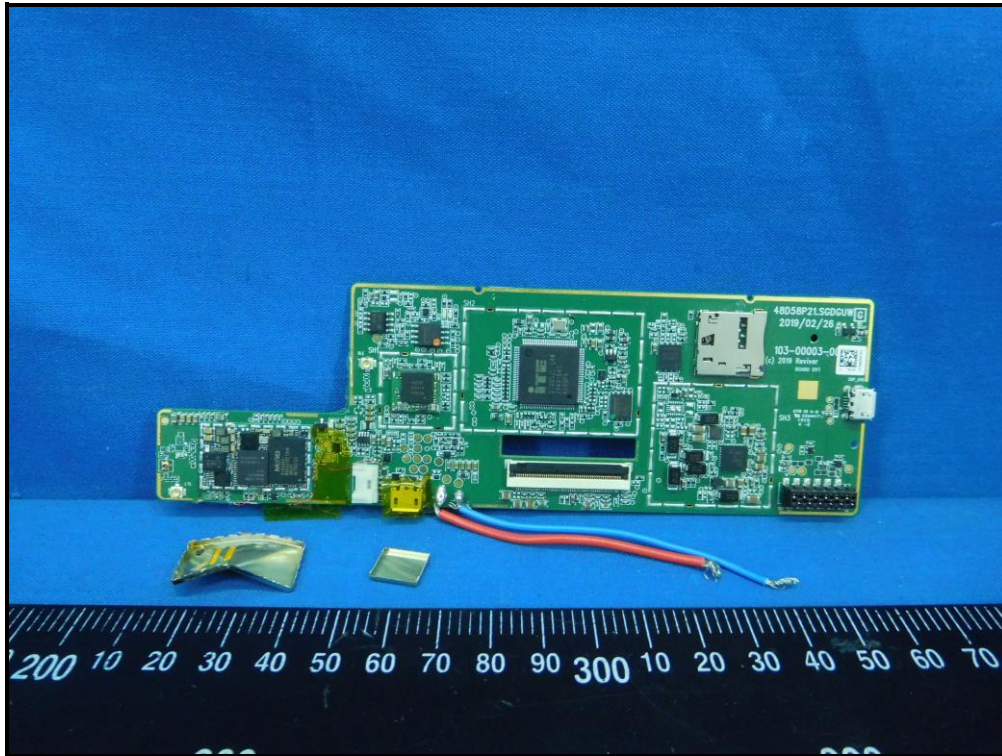
EUT with Test tools
