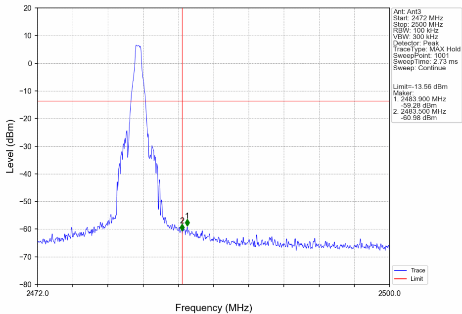
GFSK_DH5_HCH_2480MHz_Ant3_NTNV
