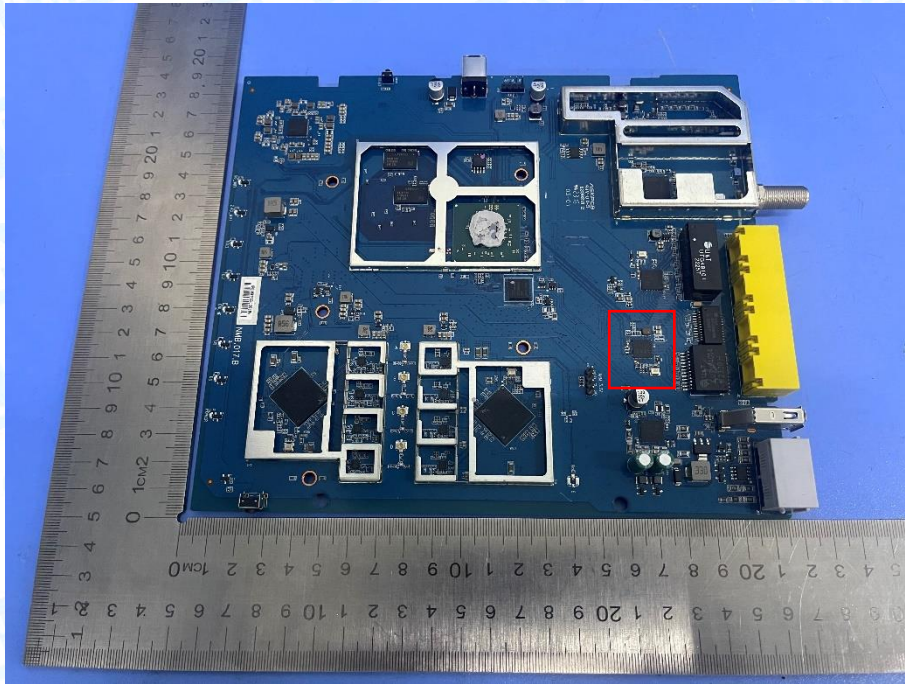
Photo 17 Appearance of PCB(1Gbps)
