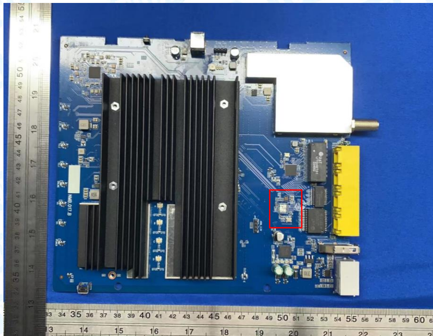
Photo 17 Appearance of PCB(1Gbps)
