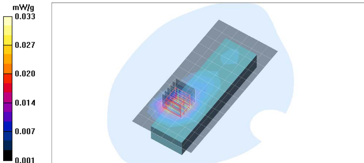
Plot. 2: SAR distribution plot for DECT, channel 4, body-worn configuration, front side, 0mm gap.
