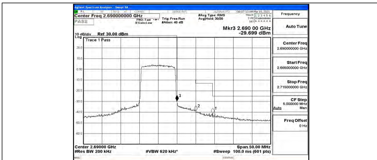
Band41-15MHz-QPSK-39725-75RB#0
