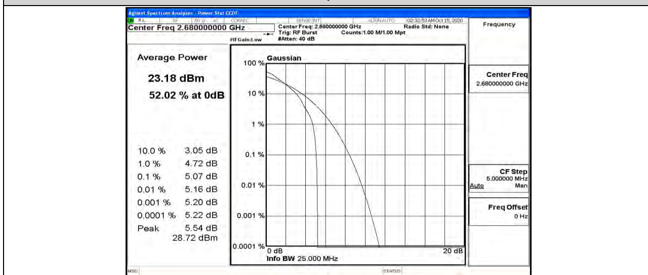
Band41-20MHz-QPSK-41490-100RB#0
