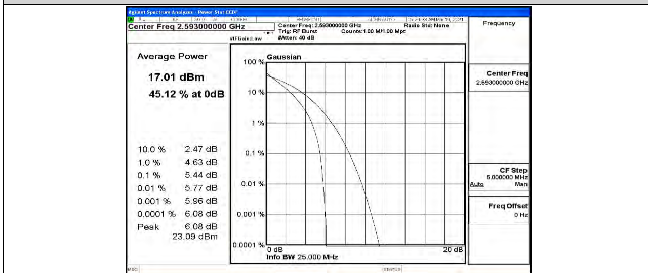
Band41-15MHz-QPSK-41515-1RB#0
