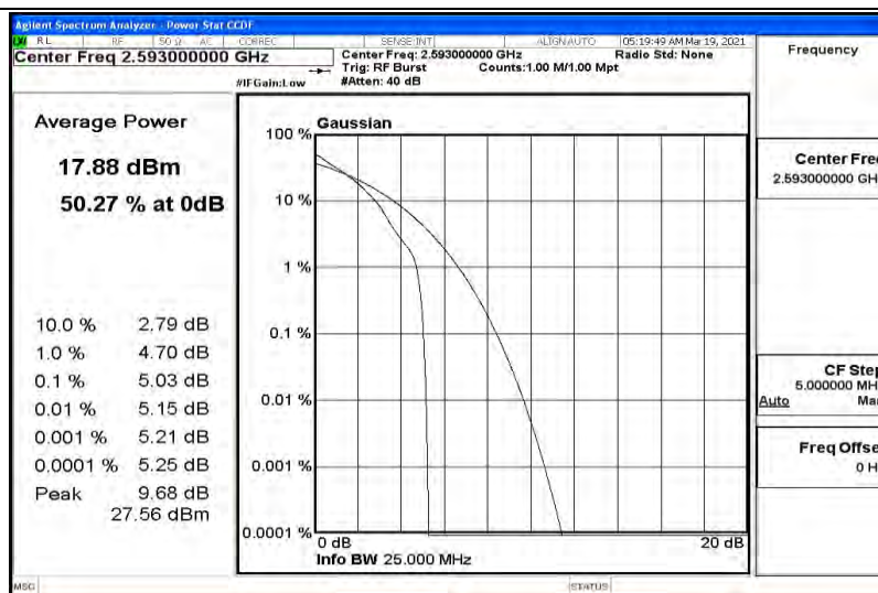
Band41-10MHz-QPSK-40620-50RB#0
