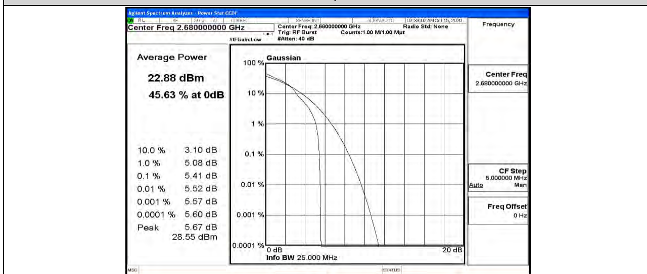
Band41-20MHz-16QAM-41490-100RB#0
