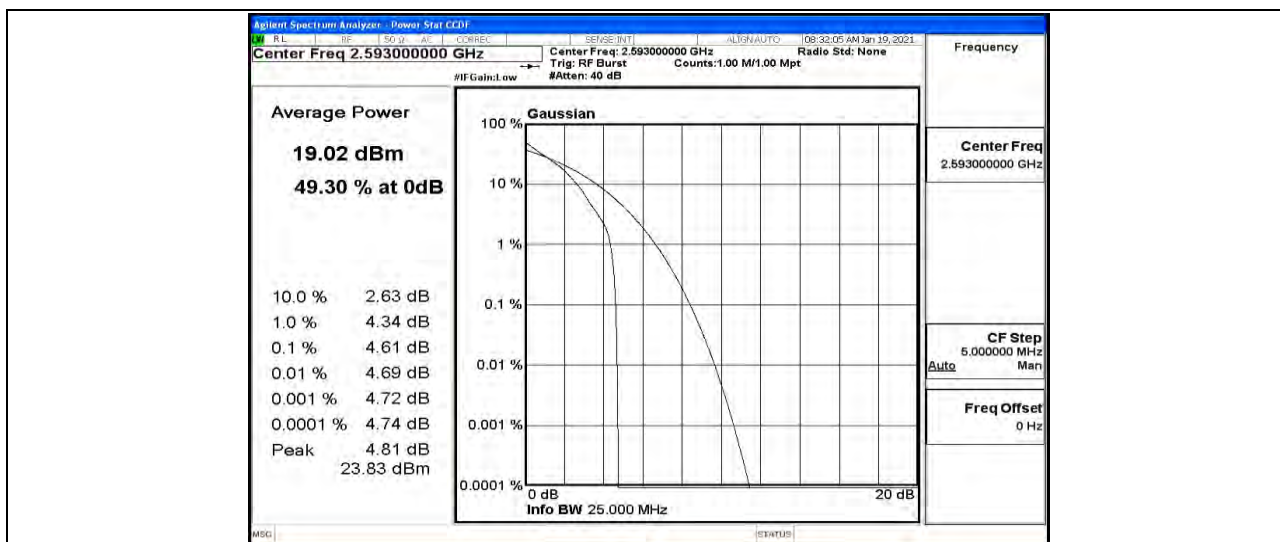
Band41-20MHz-QPSK-40620-100RB#0
