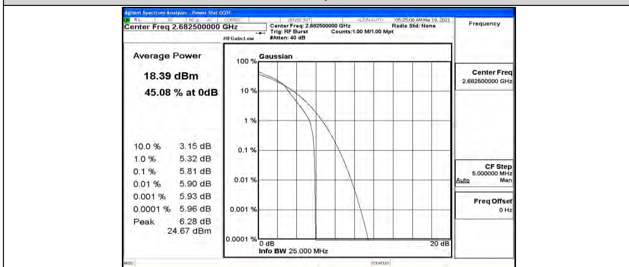
Band41-15MHz-16QAM-41515-75RB#0
