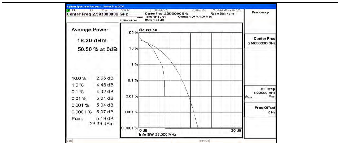
Band41-15MHz-QPSK-40620-75RB#0
