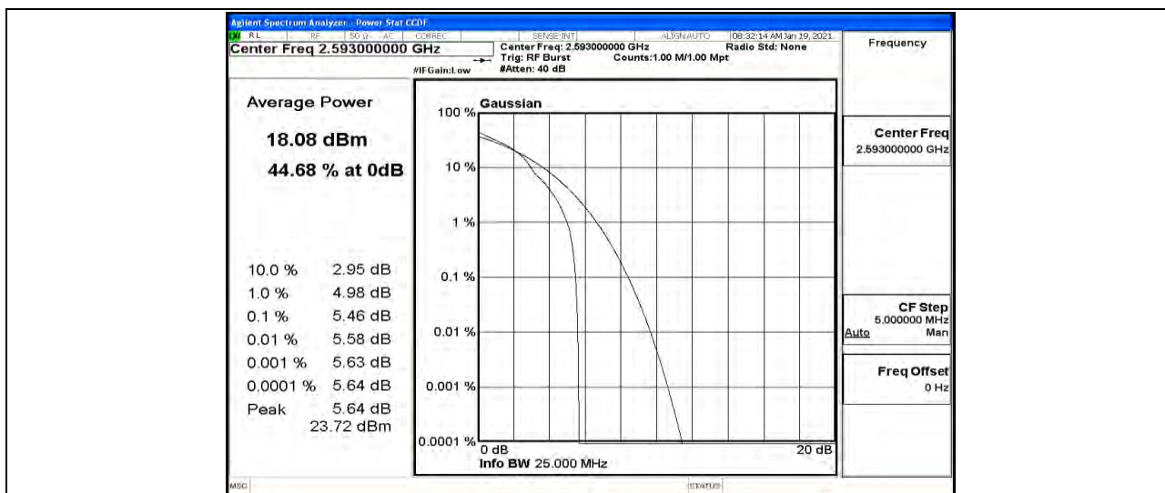
Band41-20MHz-16QAM-40620-100RB#0
