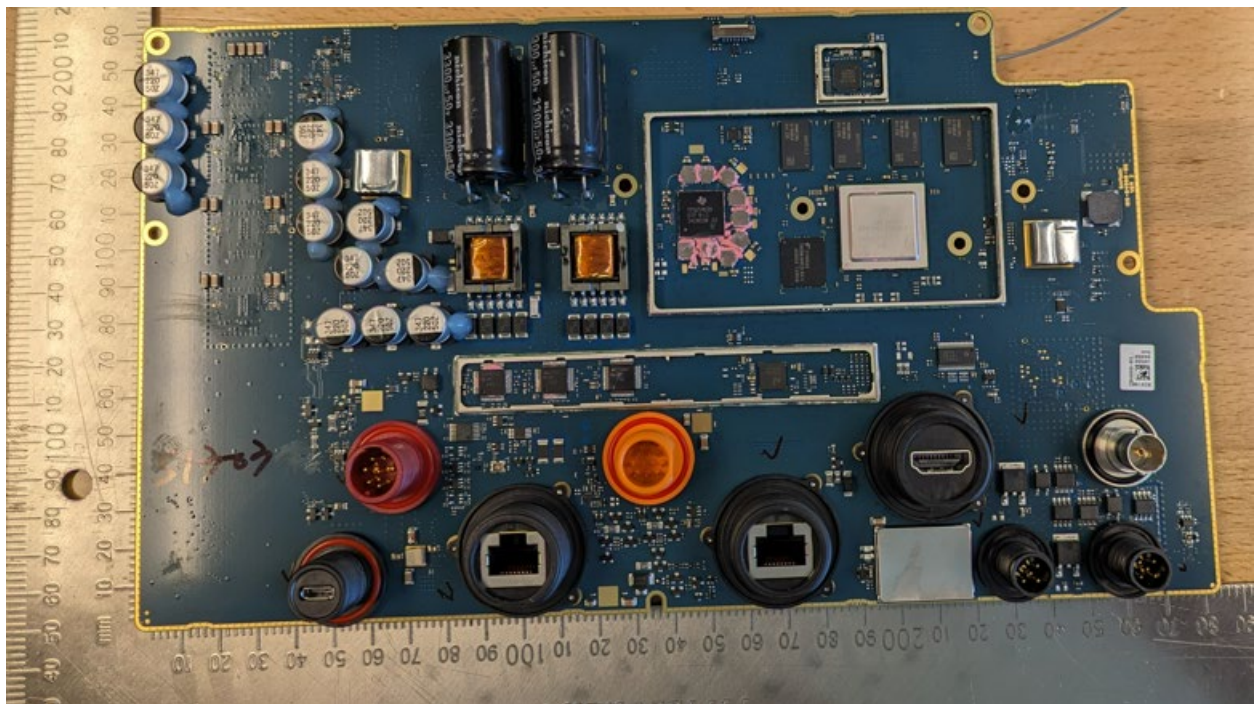
PCBA: (Back)
