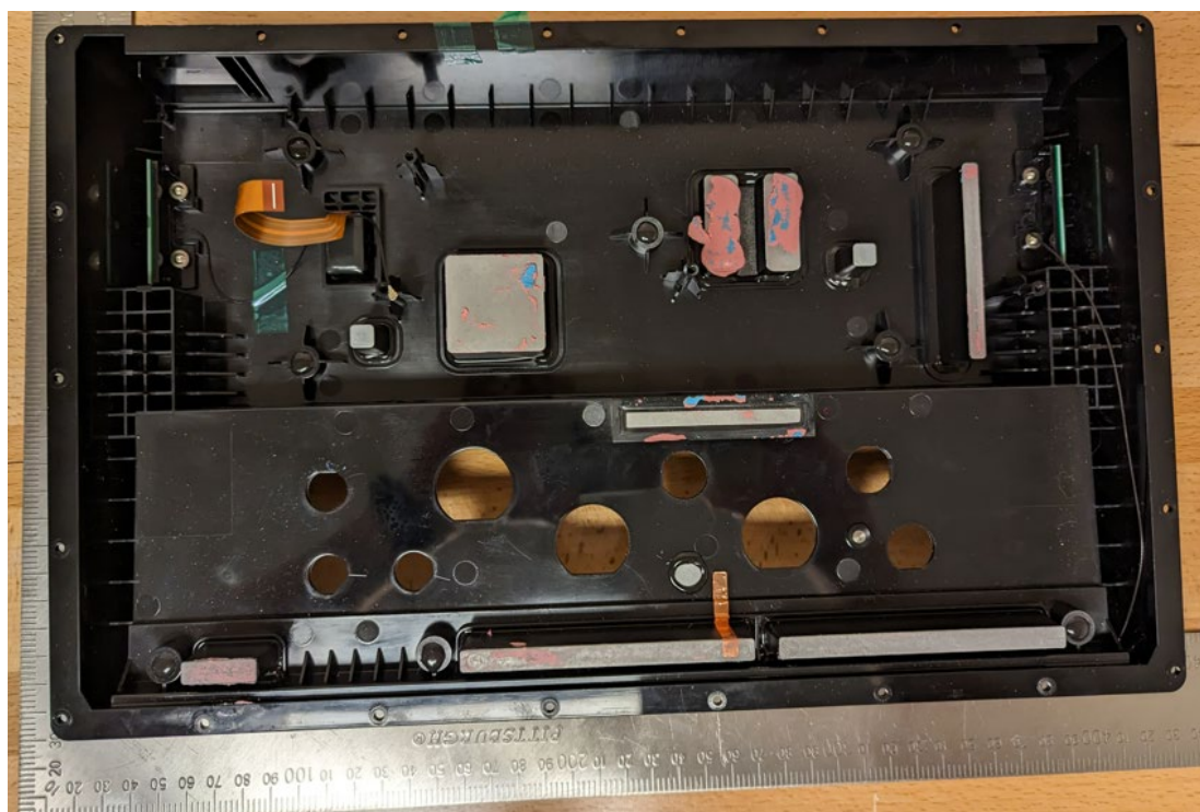
Rear: (Empty)
