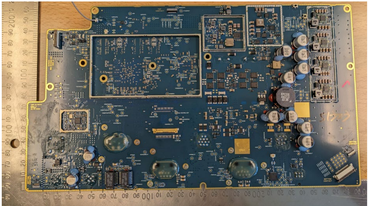
PCBA: (Front)
