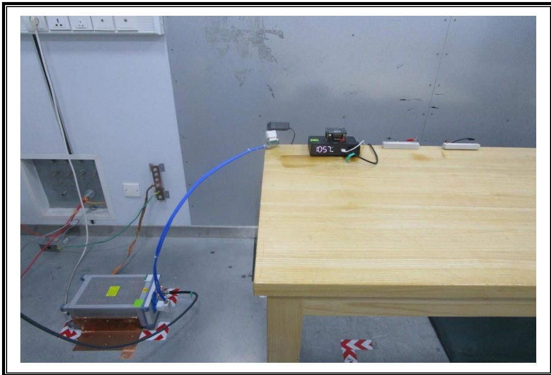
AC Power Line Conducted Emission
