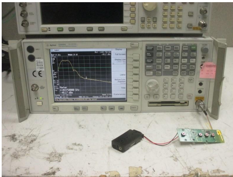
Conducted Average Power Measurements at Antenna Port ( reference only)
