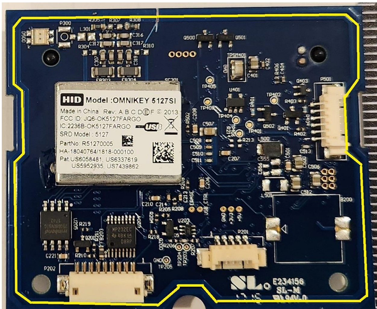
OMNIKEY 5127SI_LF Antenna Location (PCB Trace_yellow)
