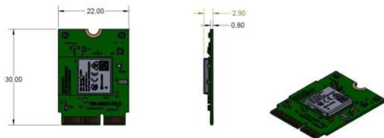
Figure 11: Module dimension of LWB5+ M.2 module – Top View
