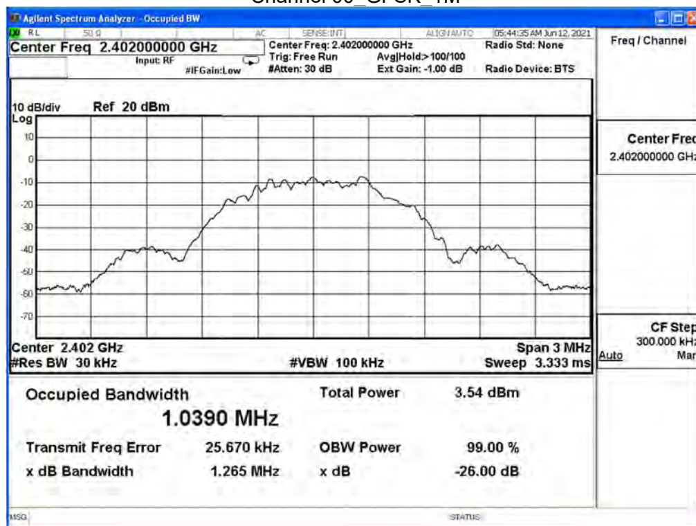
Channel 00_GFSK_1M
