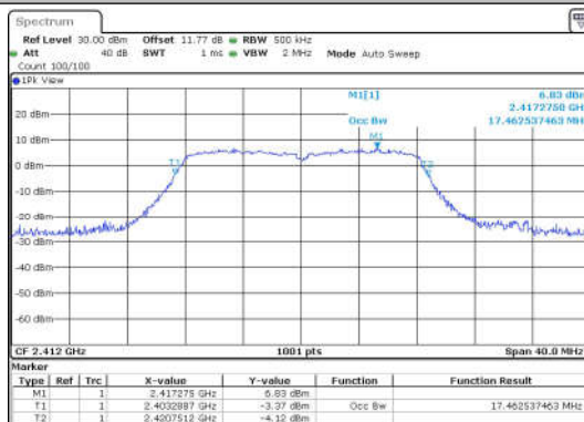
11G-Ant1-2412
