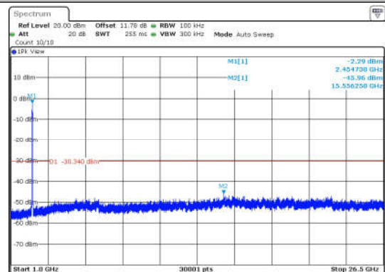
11N40SISO-Ant1-2452-1000~26500-PASS
