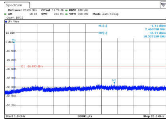
11G-Ant1-2462-1000~26500-PASS
