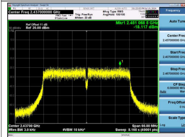
11N40SISO-Ant1-2437-PASS
