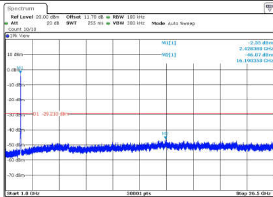
11N40SISO-Ant1-2437-1000~26500-PASS
