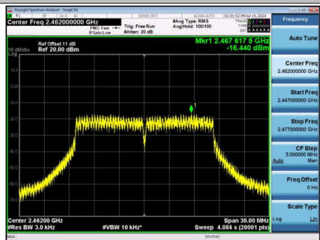
11G-Ant1-2462-PASS
