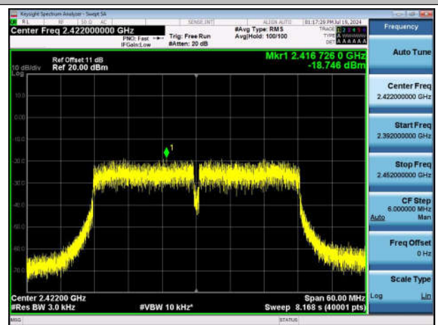
11N40SISO-Ant1-2422-PASS
