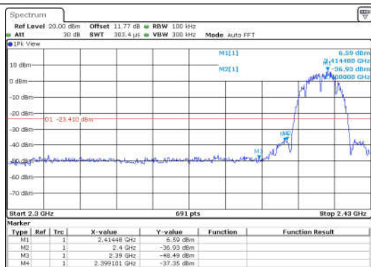
11B-Ant1-2412-PASS
