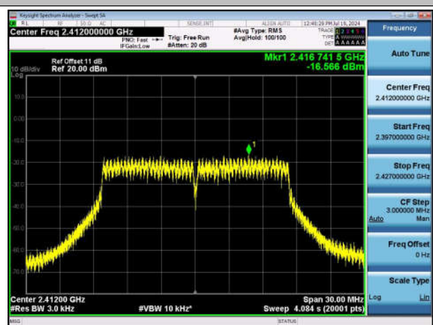
11G-Ant1-2412-PASS
