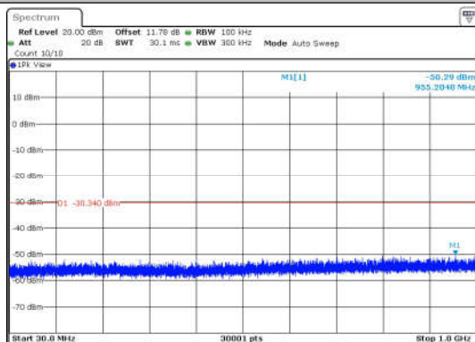
11N40SISO-Ant1-2452-30~1000-PASS
