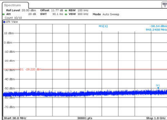
11N40SISO-Ant1-2422-30~1000-PASS
