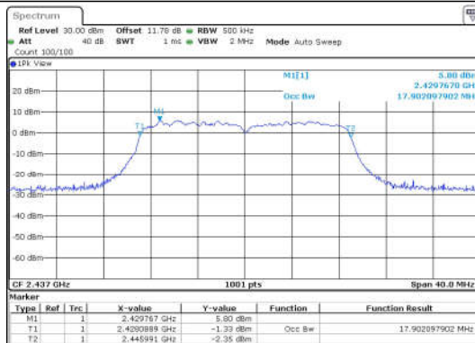
11N20SISO-Ant1-2437
