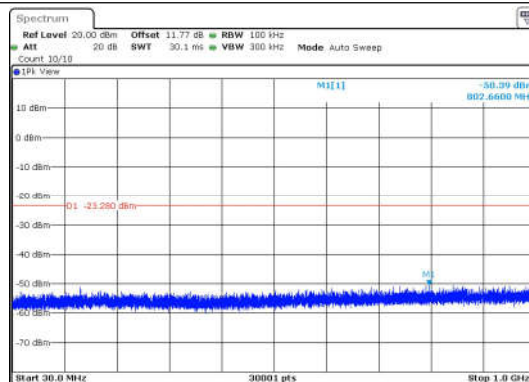
11B-Ant1-2412-30~1000-PASS
