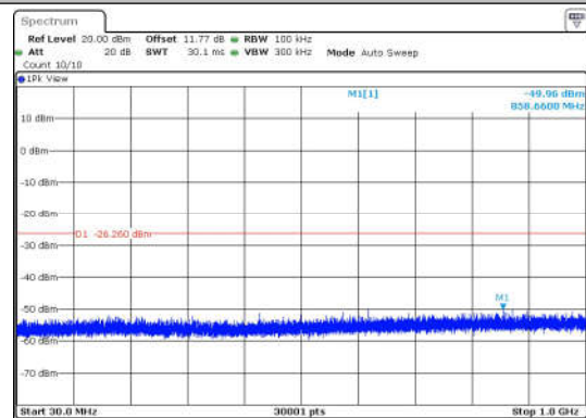
11N20SISO-Ant1-2412-30~1000-PASS
