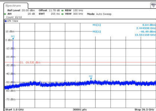
11N20SISO-Ant1-2437-1000~26500-PASS
