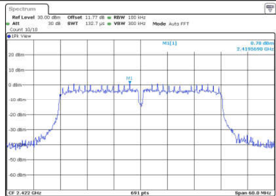
11N40SISO-Ant1-2422-0~Reference-PASS
