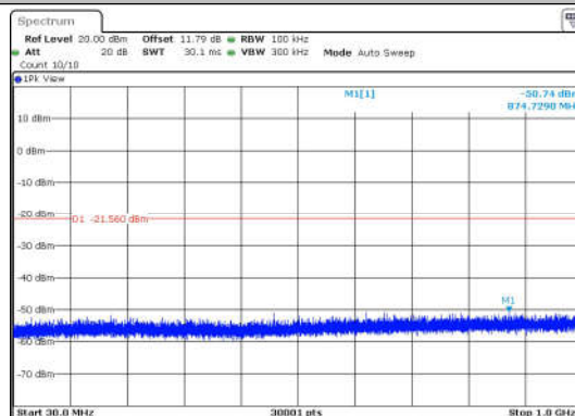
11B-Ant1-2462-30~1000-PASS
