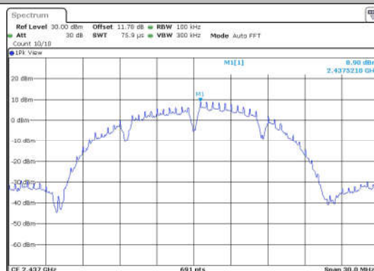
11B-Ant1-2437-0~Reference-PASS
