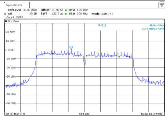
11N40SISO-Ant1-2452-0~Reference-PASS
