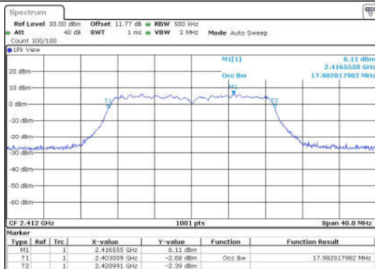
11N20SISO-Ant1-2412
