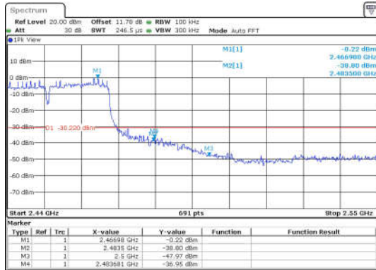
11N40SISO-Ant1-2452-PASS
