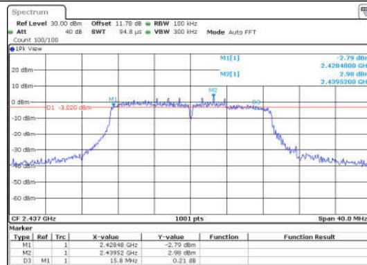
11N20SISO-Ant1-2437-PASS
