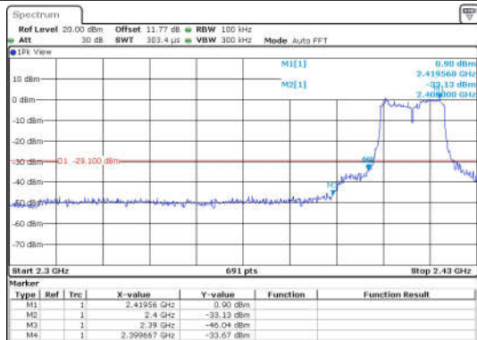
11N20SISO-Ant1-2412-PASS
