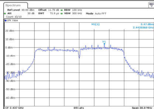
11N20SISO-Ant1-2437-0~Reference-PASS
