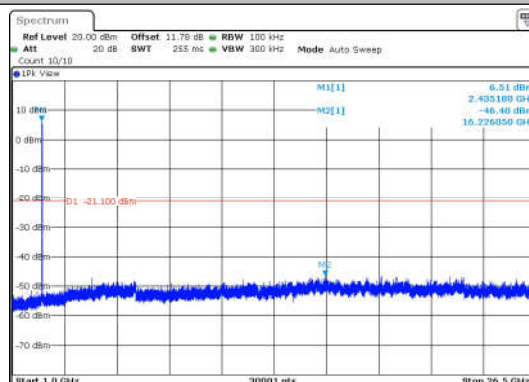
11B-Ant1-2437-1000~26500-PASS
