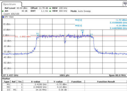
11N40SISO-Ant1-2437-PASS
