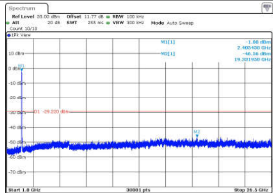
11N40SISO-Ant1-2422-1000~26500-PASS
