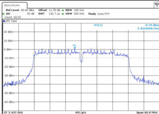
11N40SISO-Ant1-2437-0~Reference-PASS
