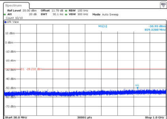
11N40SISO-Ant1-2437-30~1000-PASS
