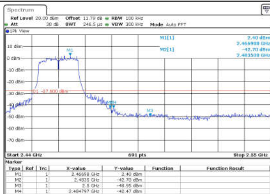
11G-Ant1-2462-PASS
