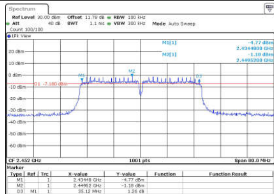
11N40SISO-Ant1-2452-PASS
