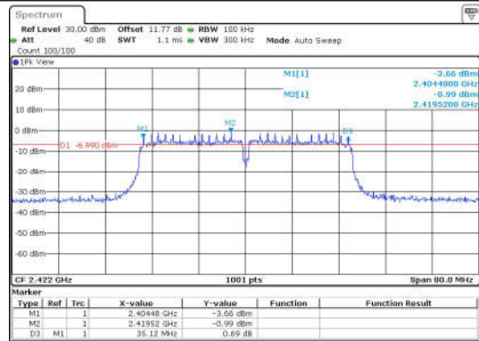
11N40SISO-Ant1-2422-PASS
