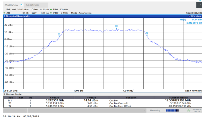
11A-CDD_Ant3_5240
