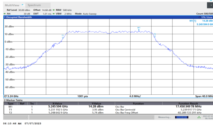
11A-CDD_Ant4_5240
