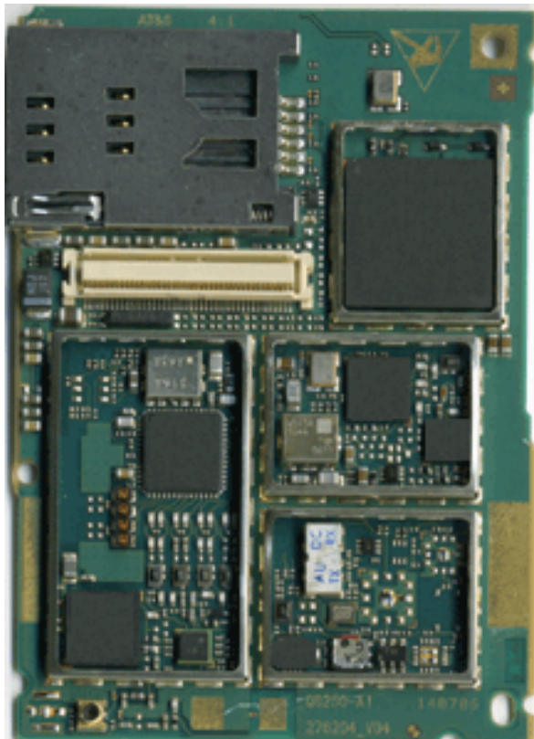
Siemens Cellular Engine HMS1 Top side without shielding
