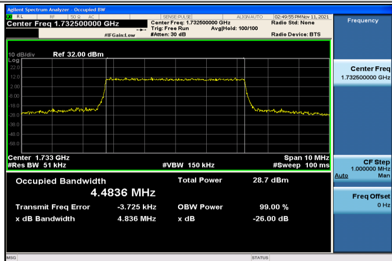
Band4-5MHz-QPSK-20175-25RB#0-4.4836
