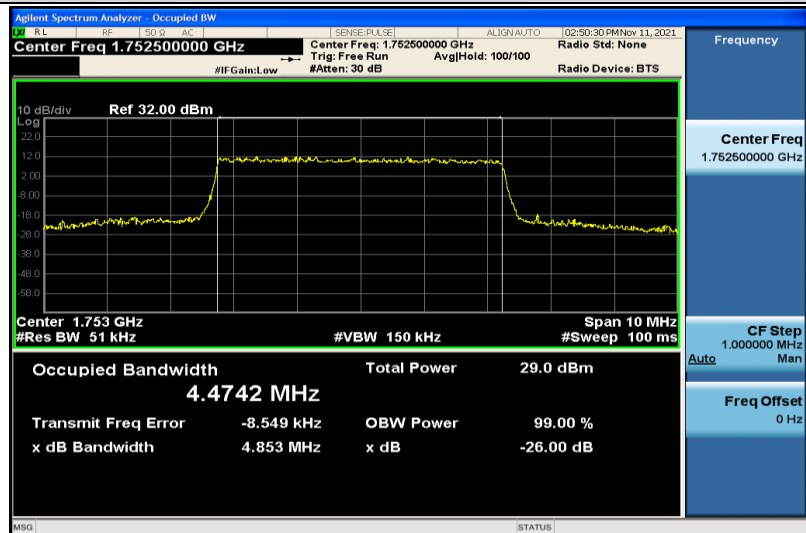
Band4-5MHz-QPSK-20375-25RB#0-4.4742
