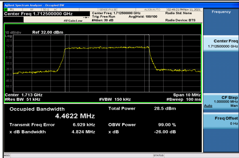
Band4-5MHz-QPSK-19975-25RB#0-4.4622
