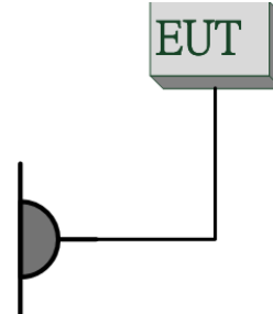
Fig 2-3 Conduction (AC Power Line) Emission
