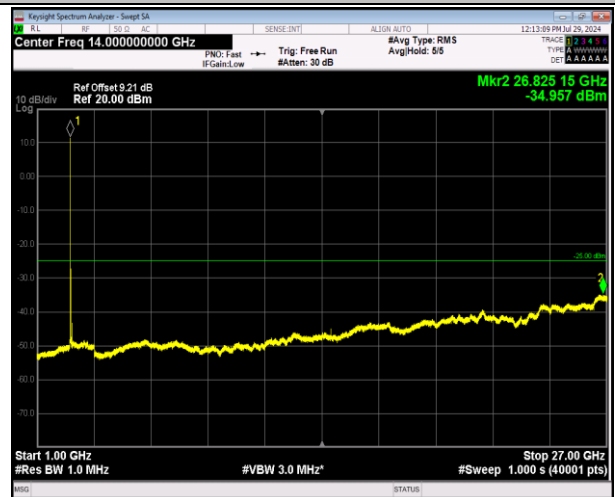
7-7-20MHz-20MHz-64QAM-64QAM-21001-21199-1RB#0-1-1000~27000MHz-PASS
