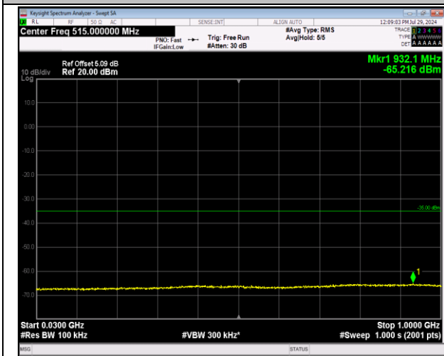
7-7-20MHz-20MHz-64QAM-64QAM-20850-21048-1RB#0 -0RB#0-30~1000MHz-PASS
