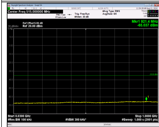
7-7-20MHz-20MHz-QPSK-QPSK-21001-21199-1RB#99-0 RB#0-30~1000MHz-PASS
