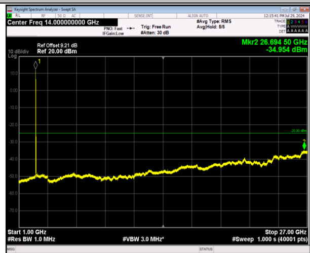
7-7-20MHz-20MHz-64QAM-64QAM-21152-21350-1RB#0-1-1000~27000MHz-PASS
