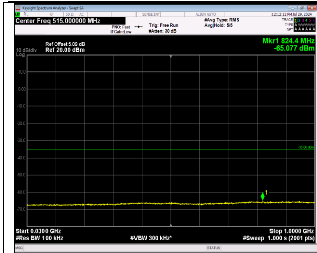
7-7-20MHz-20MHz-64QAM-64QAM-21001-21199-1RB#9 9-ORB#0-30~1000MHz-PASS
