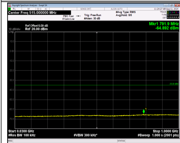
7-7-20MHz-10MHz-QPSK-QPSK-21251-21395-1RB#0-0 RB#0-30~1000MHz-PASS
