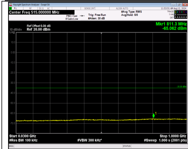
7-7-20MHz-20MHz-16QAM-16QAM-21001-21199-1RB#0 -ORB#0-30~1000MHz-PASS
