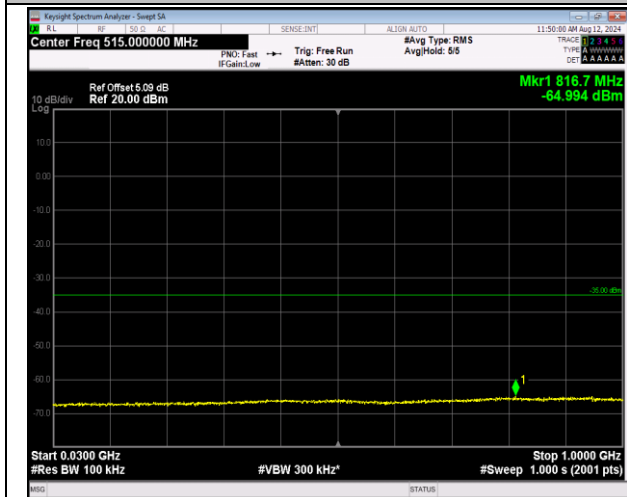
7-7-20MHz-20MHz-16QAM-16QAM-20850-21048-1RB#99 9-ORB#0-30~1000MHz-PASS
