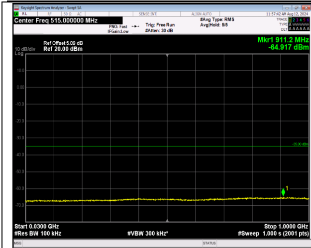
7-7-20MHz-20MHz-16QAM-16QAM-21001-21199-100RB#0-100RB#0-30~1000MHz-PASS
