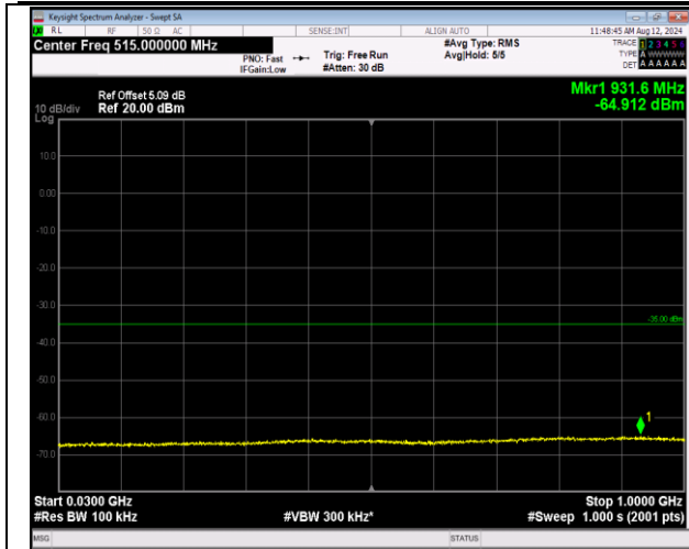
7-7-20MHz-20MHz-16QAM-16QAM-20850-21048-1RB#0 -ORB#0-30~1000MHz-PASS
