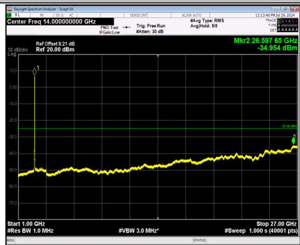
7-7-20MHz-20MHz-64QAM-64QAM-21001-21199-100RB#0 -100RB#0-1000~27000MHz-PASS
