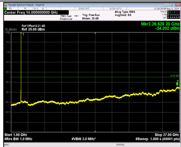
7-7-20MHz-10MHz-16QAM-16QAM-21251-21395-1RB#99- ORB#0-1000~27000MHz-PASS
