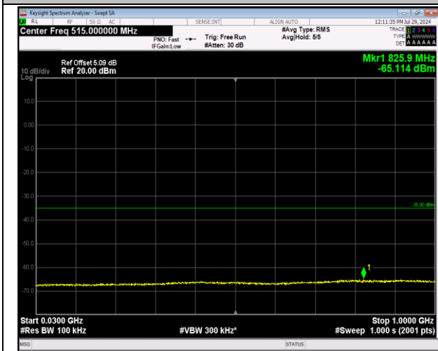
7-7-20MHz-20MHz-64QAM-64QAM-21001-21199-1RB#0-0-30~1000MHz-PASS
