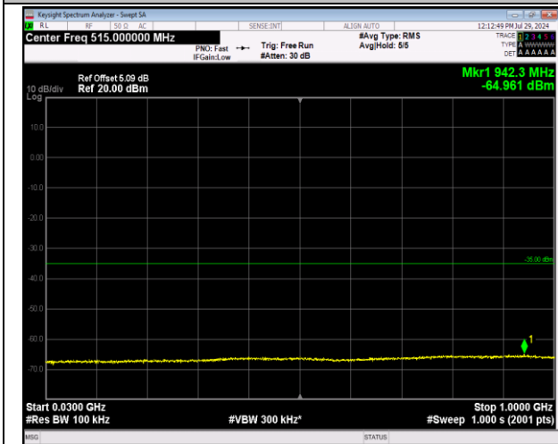
7-7-20MHz-20MHz-64QAM-64QAM-21001-21199-1RB#0-1-30~1000MHz-PASS
