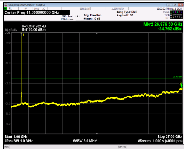
7-7-20MHz-20MHz-16QAM-16QAM-21152-21350-1RB#99- ORB#0-1000~27000MHz-PASS
