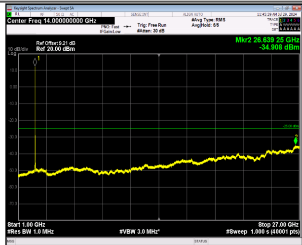
7-7-20MHz-10MHz-64QAM-64QAM-21251-21395-1RB#0-1 RB#49-1000~27000MHz-PASS
