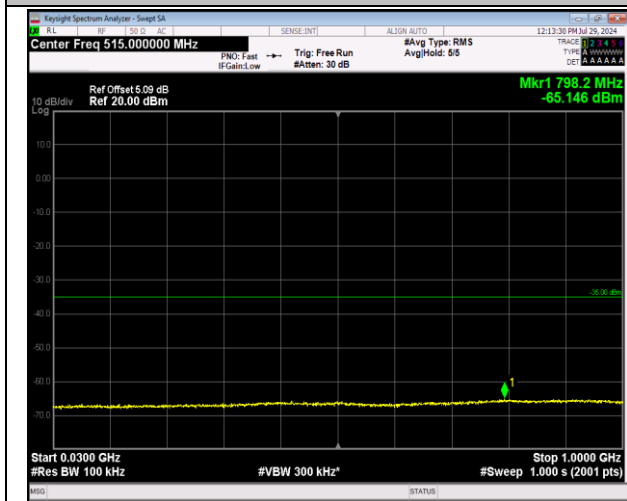
7-7-20MHz-20MHz-64QAM-64QAM-21001-21199-100RB #0-100RB#0-30~1000MHz-PASS
