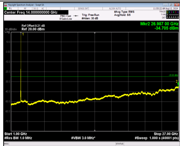
7-7-20MHz-20MHz-16QAM-16QAM-21001-21199-1RB#99- ORB#0-1000~27000MHz-PASS
