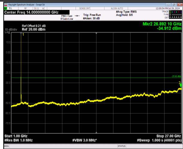
7-7-20MHz-20MHz-64QAM-64QAM-20850-21048-1RB#99- ORB#0-1000~27000MHz-PASS
