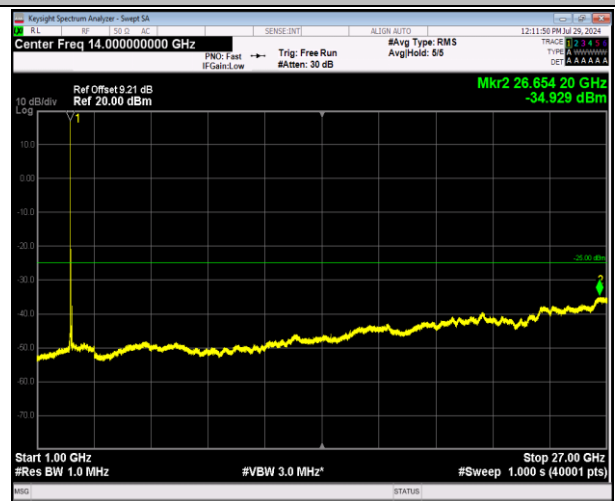
7-7-20MHz-20MHz-64QAM-64QAM-21001-21199-1RB#0-0-1000~27000MHz-PASS
