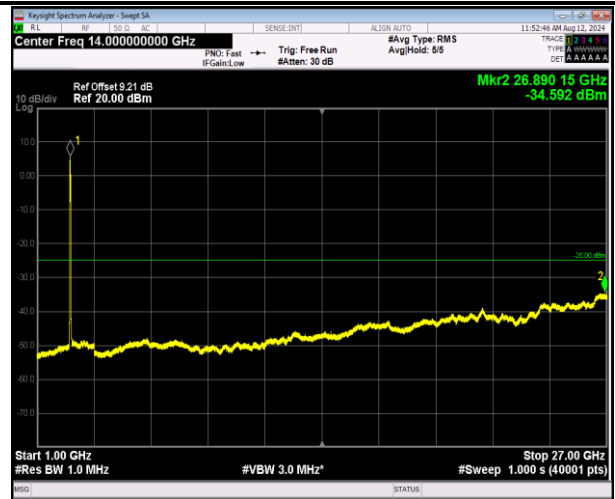
7-7-20MHz-20MHz-16QAM-16QAM-20850-21048-100RB#0 -100RB#0-1000~27000MHz-PASS
