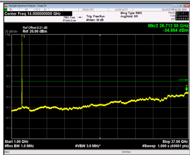
7-7-20MHz-20MHz-64QAM-64QAM-21152-21350-1RB#0-0-1000~27000MHz-PASS
