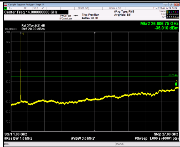
7-7-20MHz-10MHz-64QAM-64QAM-21051-21195-1RB#99- 0RB#0-1000~27000MHz-PASS
