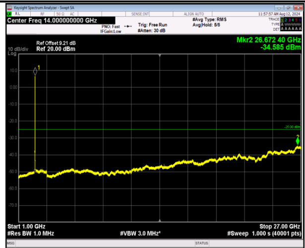
7-7-20MHz-20MHz-16QAM-16QAM-21001-21199-100RB#0-100RB#0-1000~27000MHz-PASS
