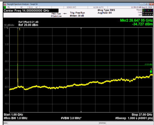
7-7-20MHz-20MHz-16QAM-16QAM-20850-21048-1RB#99- ORB#0-1000~27000MHz-PASS
