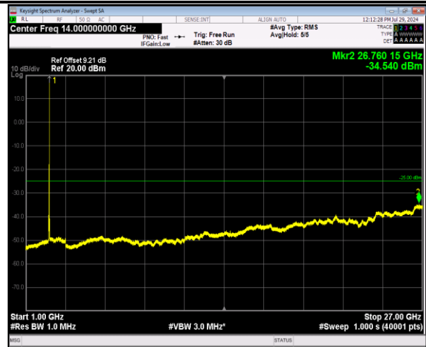
7-7-20MHz-20MHz-64QAM-64QAM-21001-21199-1RB#99- ORB#0-1000~27000MHz-PASS
