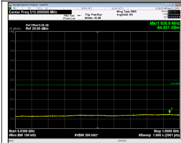
7-7-20MHz-10MHz-16QAM-16QAM-21251-21395-1RB#9 9-ORB#0-30~1000MHz-PASS
