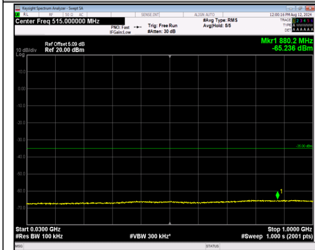
7-7-20MHz-20MHz-16QAM-16QAM-21152-21350-1RB#9 9-ORB#0-30~1000MHz-PASS
