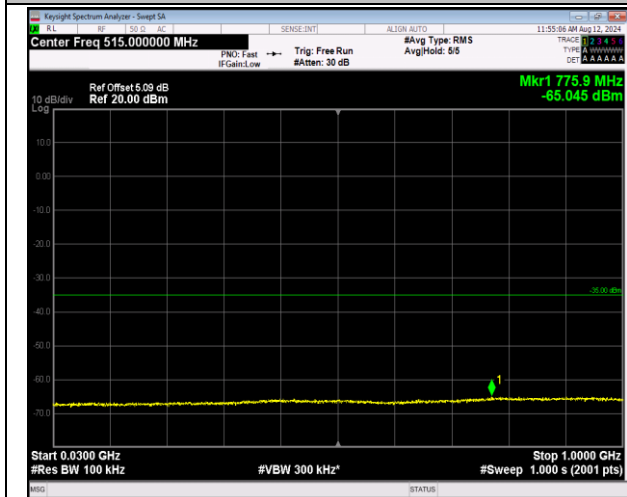
7-7-20MHz-20MHz-16QAM-16QAM-21001-21199-1RB#99 9-ORB#0-30~1000MHz-PASS
