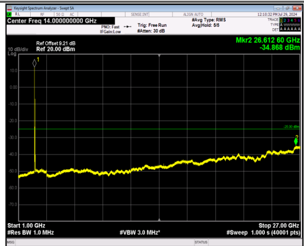
7-7-20MHz-20MHz-64QAM-64QAM-20850-21048-1RB#0-1 RB#99-1000~27000MHz-PASS
