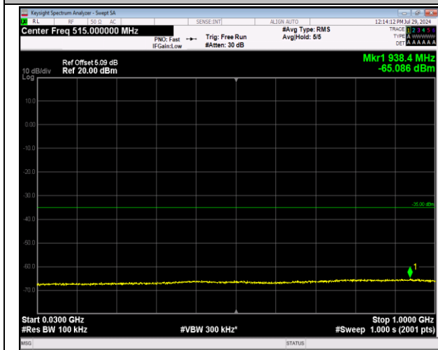
7-7-20MHz-20MHz-64QAM-64QAM-21152-21350-1RB#0-0-30~1000MHz-PASS
