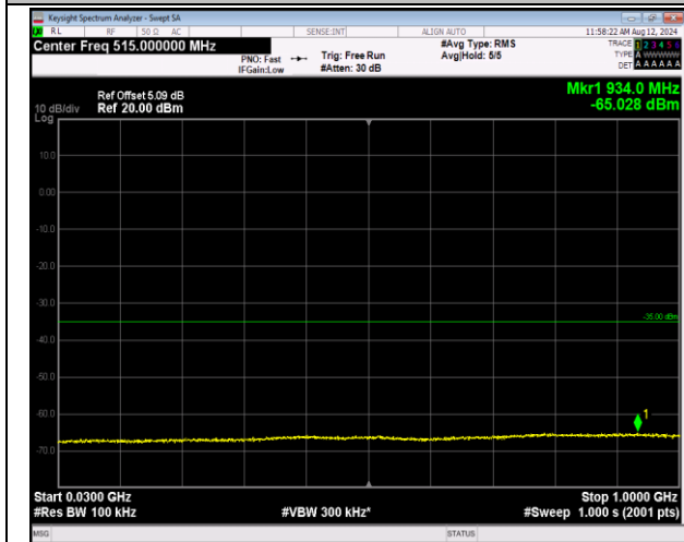
7-7-20MHz-20MHz-QPSK-QPSK-21152-21350-1RB#0-0 RB#0-30~1000MHz-PASS
