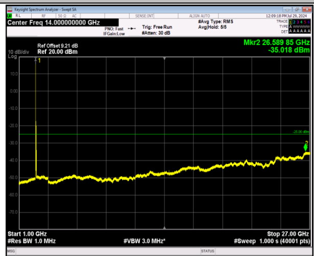
7-7-20MHz-20MHz-64QAM-64QAM-20850-21048-1RB#0-0 RB#0-1000~27000MHz-PASS
