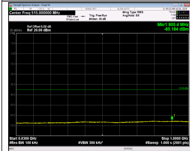
7-7-20MHz-10MHz-64QAM-64QAM-21251-21395-1RB#0 -1RB#49-30~1000MHz-PASS
