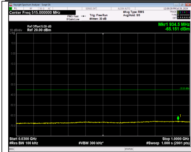
7-7-20MHz-20MHz-64QAM-64QAM-20850-21048-1RB#9 9-ORB#0-30~1000MHz-PASS
