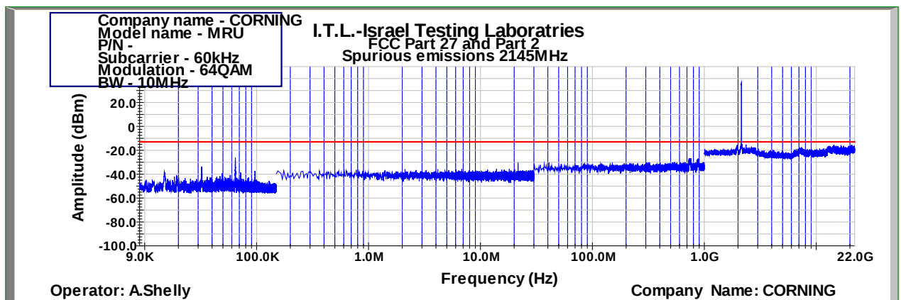
Figure 880: Spurious Emissions at Antenna Terminal 64QAM 10MHz B.W.; 2145.0MHz, 60kHz
