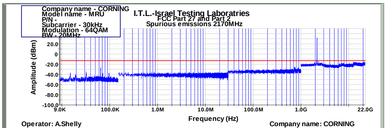
Figure 896: Spurious Emissions at Antenna Terminal 64QAM 20MHz B.W.; 2170.0MHz, 30kHz
