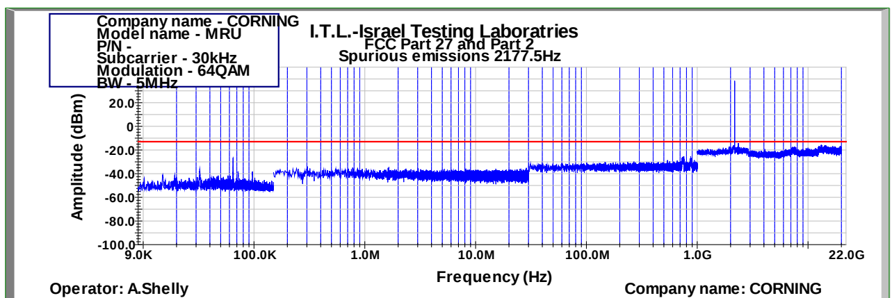
Figure 872: Spurious Emissions at Antenna Terminal 64QAM 5MHz B.W.; 2177.5MHz, 30kHz
