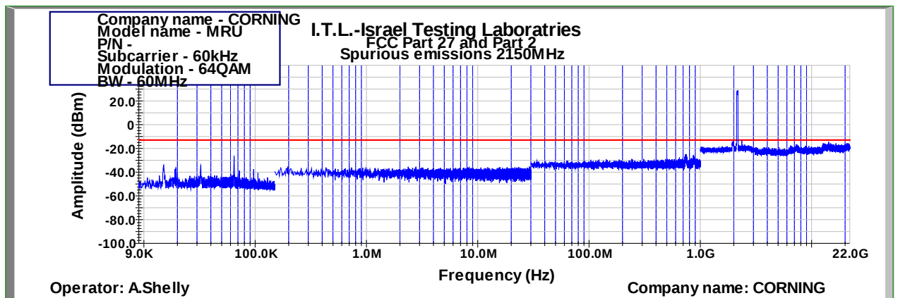
Figure 932: Spurious Emissions at Antenna Terminal 64QAM 60MHz B.W.; 2150.0MHz, 60kHz
