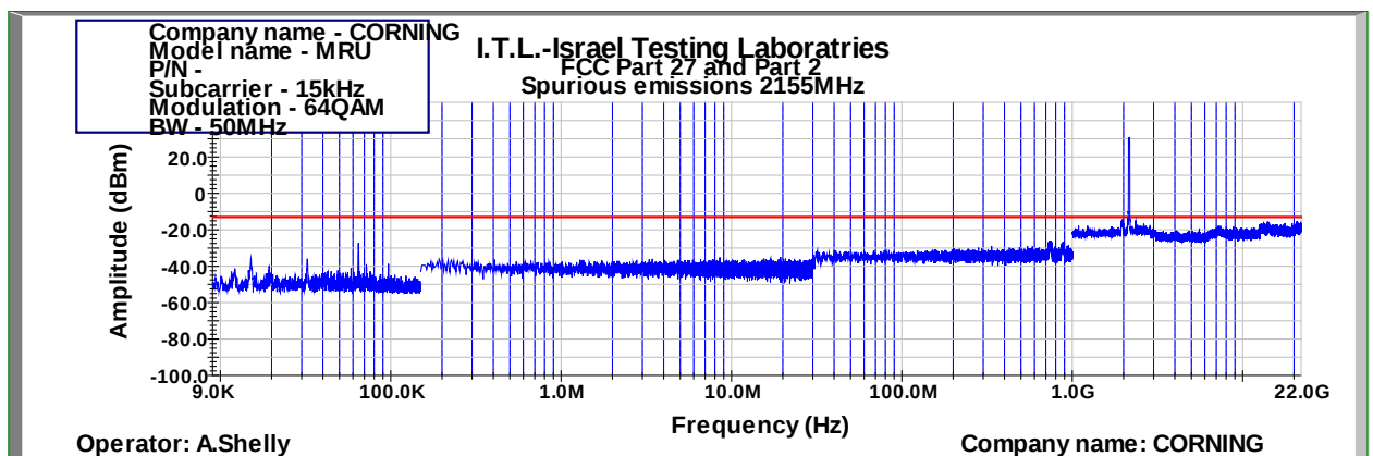
Figure 920: Spurious Emissions at Antenna Terminal 64QAM 50MHz B.W.; 2155.0MHz, 15kHz
