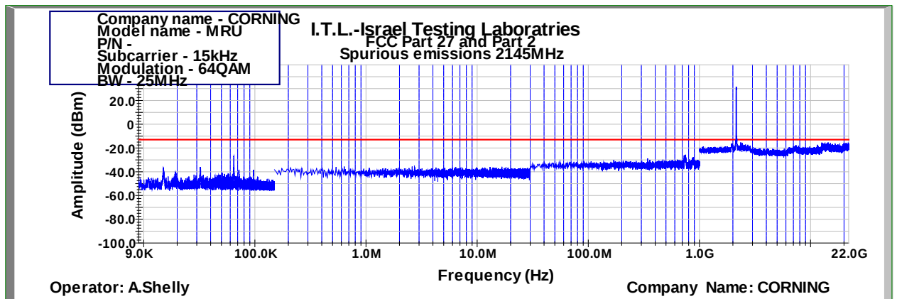
Figure 901: Spurious Emissions at Antenna Terminal 64QAM 25MHz B.W.; 2145.0MHz, 15kHz
