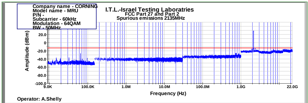
Figure 924: Spurious Emissions at Antenna Terminal 64QAM 50MHz B.W.; 2135.0MHz, 60kHz
