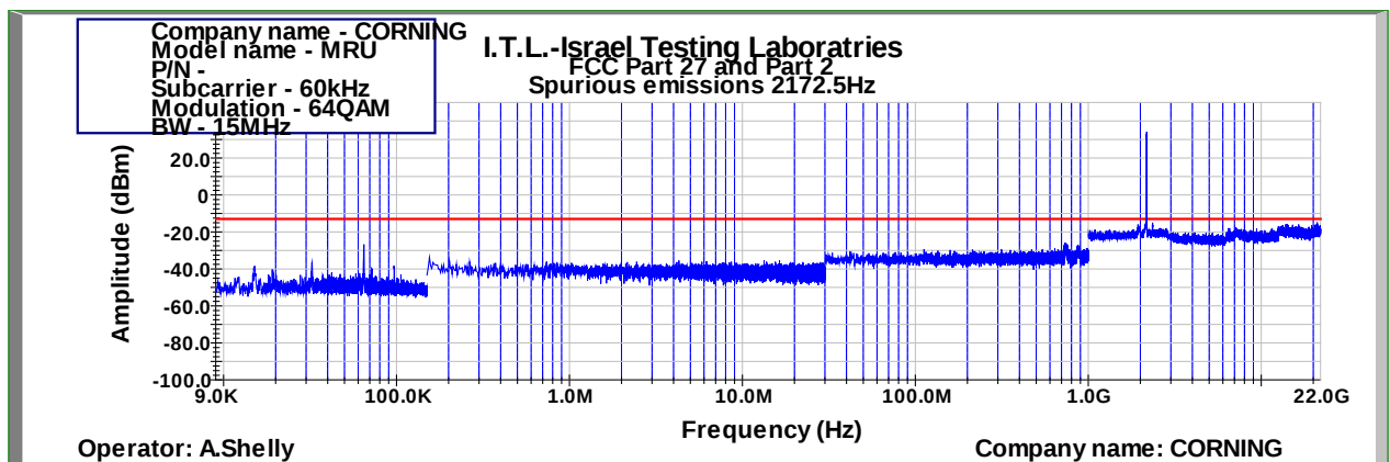
Figure 890: Spurious Emissions at Antenna Terminal 64QAM 15MHz B.W.; 2172.5MHz, 30kHz
