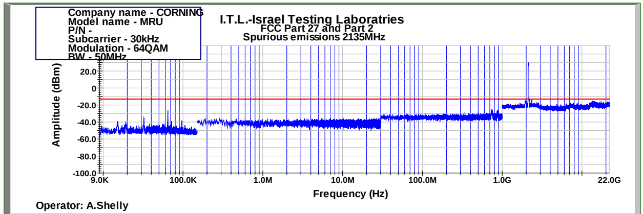
Figure 921: Spurious Emissions at Antenna Terminal 64QAM 50MHz B.W.; 2135.0MHz, 30kHz
