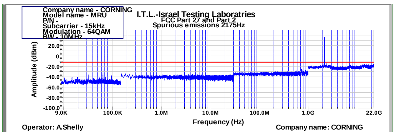
Figure 875: Spurious Emissions at Antenna Terminal 64QAM 10MHz B.W.; 2175.0MHz, 15kHz
