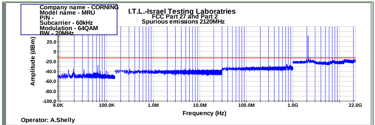
Figure 897: Spurious Emissions at Antenna Terminal 64QAM 20MHz B.W.; 2120.0MHz, 60kHz
