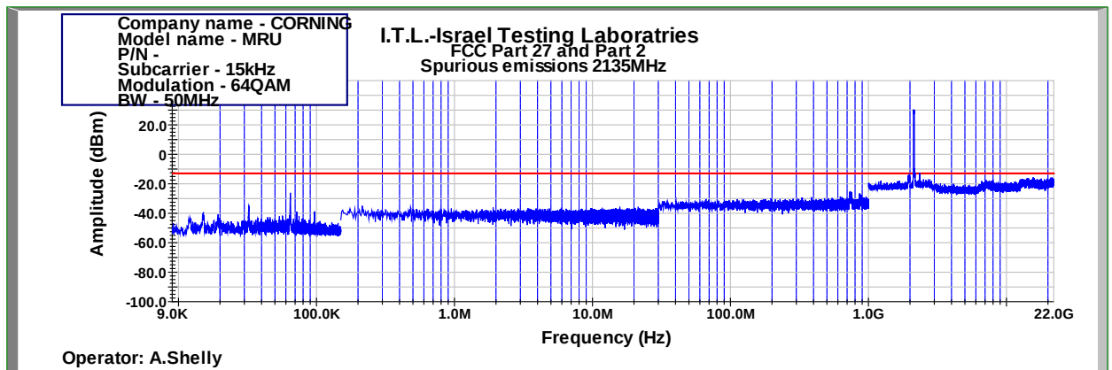
Figure 918: Spurious Emissions at Antenna Terminal 64QAM 50MHz B.W.; 2135.0MHz, 15kHz
