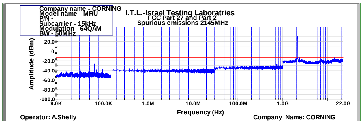
Figure 919: Spurious Emissions at Antenna Terminal 64QAM 50MHz B.W.; 2145.0MHz, 15kHz
