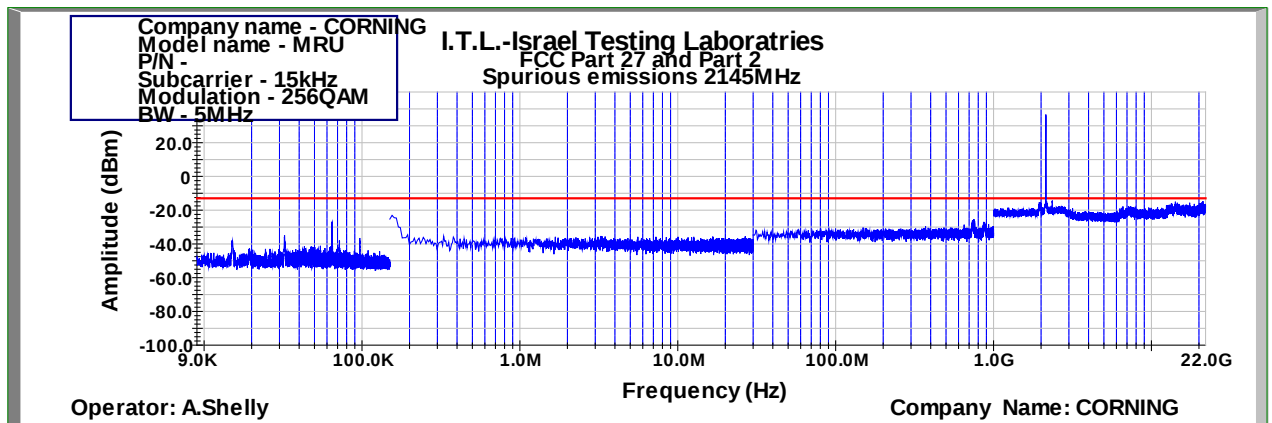
Figure 934: Spurious Emissions at Antenna Terminal 256QAM 5MHz B.W.; 2145.0MHz, 15kHz
