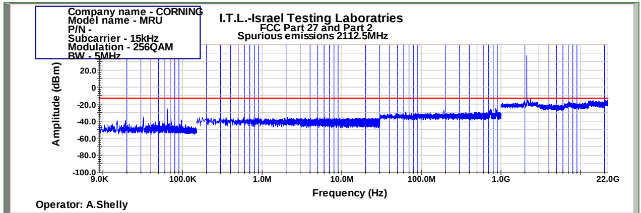
Figure 933: Spurious Emissions at Antenna Terminal 256QAM 5MHz B.W.; 2112.5MHz, 15kHz
