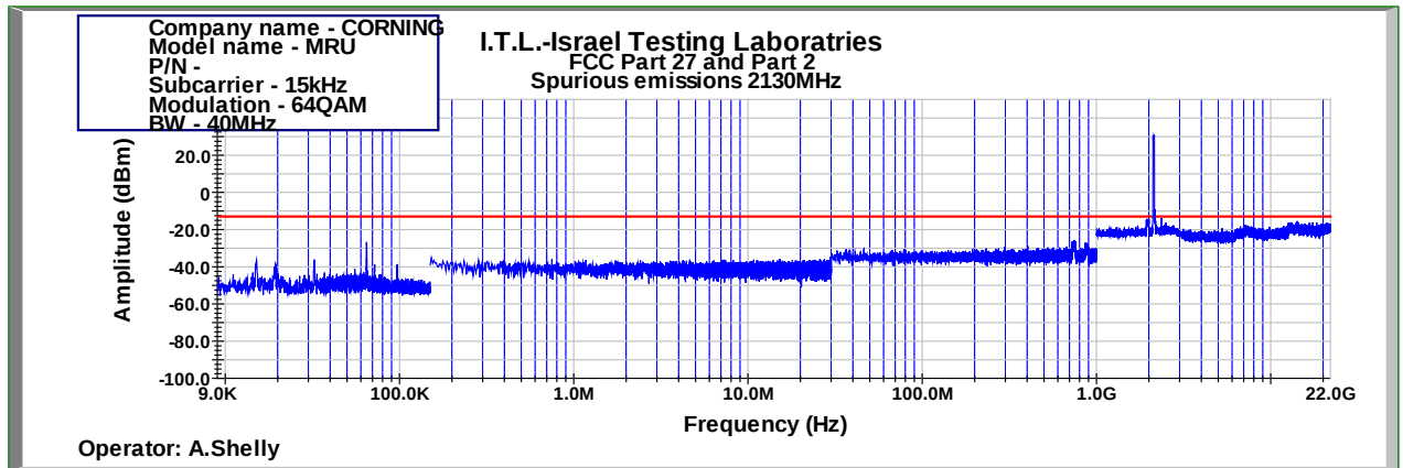
Figure 909: Spurious Emissions at Antenna Terminal 64QAM 40MHz B.W.; 2130.0MHz, 15kHz
