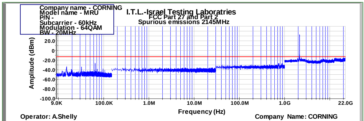
Figure 898: Spurious Emissions at Antenna Terminal 64QAM 20MHz B.W.; 2145.0MHz, 60kHz
