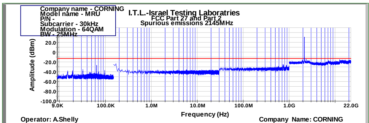
Figure 904: Spurious Emissions at Antenna Terminal 64QAM 25MHz B.W.; 2145.0MHz, 30kHz
