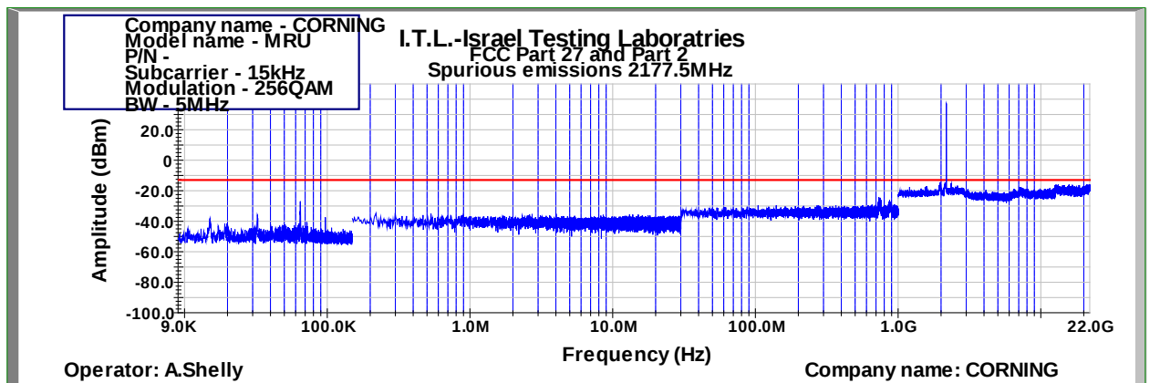
Figure 935: Spurious Emissions at Antenna Terminal 256QAM 5MHz B.W.; 2177.5MHz, 15kHz
