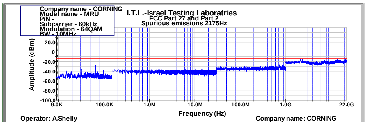
Figure 881: Spurious Emissions at Antenna Terminal 64QAM 10MHz B.W.; 2175.0MHz, 60kHz
