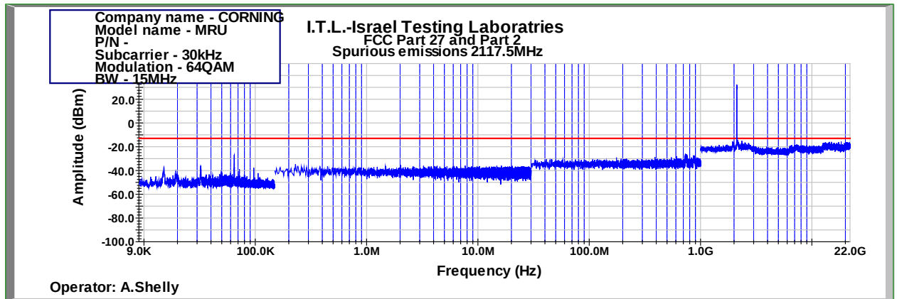
Figure 885: Spurious Emissions at Antenna Terminal 64QAM 15MHz B.W.; 2117.5MHz, 30kHz
