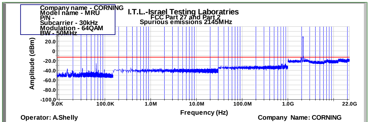
Figure 922: Spurious Emissions at Antenna Terminal 64QAM 50MHz B.W.; 2145.0MHz, 30kHz
