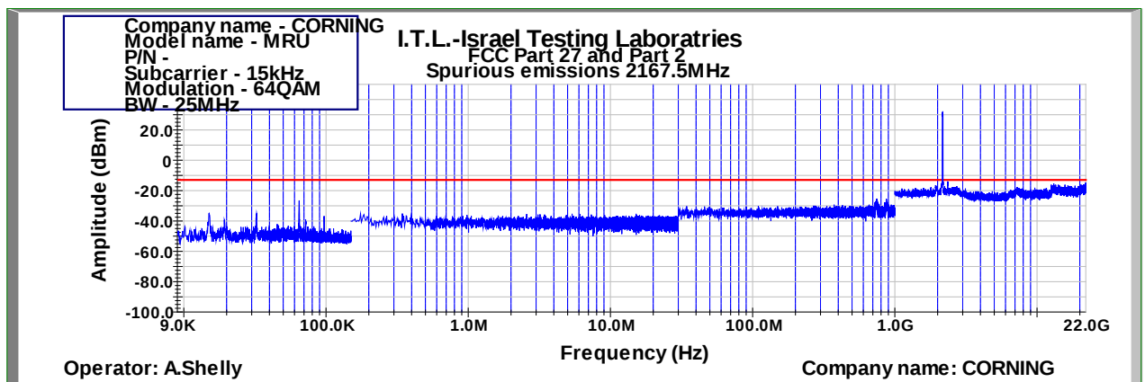
Figure 902: Spurious Emissions at Antenna Terminal 64QAM 25MHz B.W.; 2167.5MHz, 15kHz
