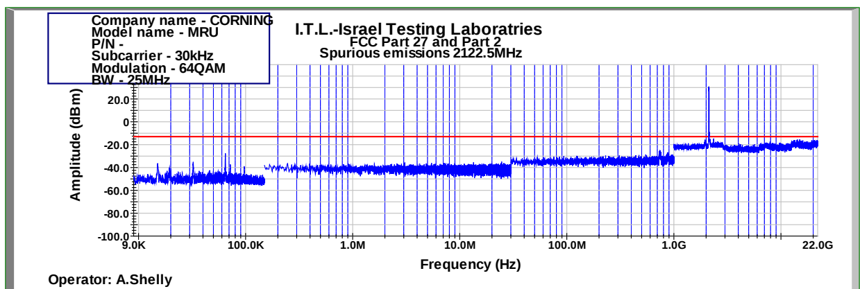
Figure 903: Spurious Emissions at Antenna Terminal 64QAM 25MHz B.W.; 2122.5MHz, 30kHz
