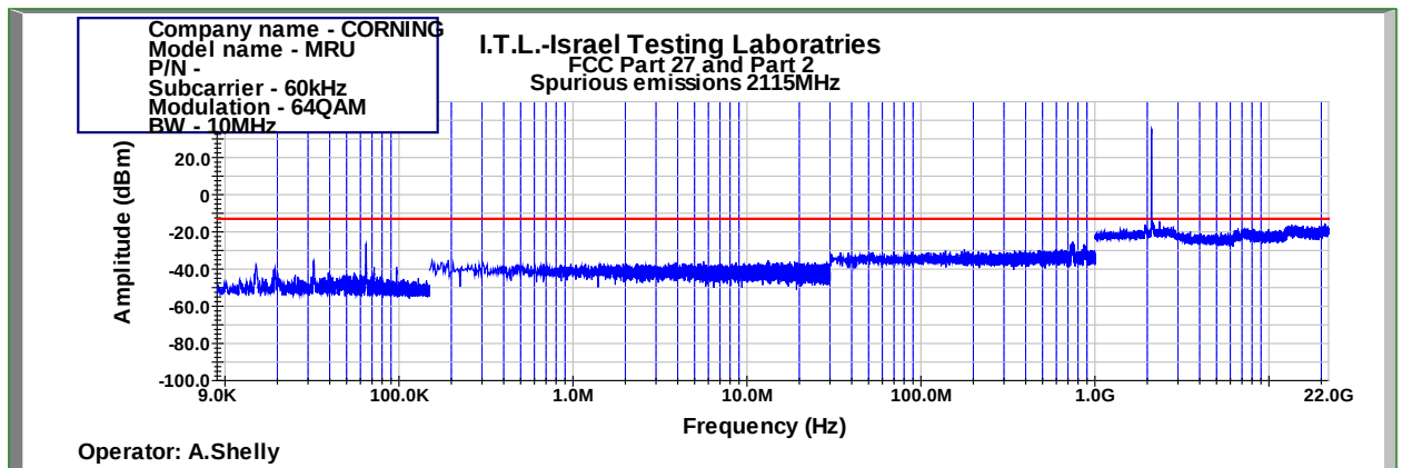
Figure 879: Spurious Emissions at Antenna Terminal 64QAM 10MHz B.W.; 2115.0MHz, 60kHz
