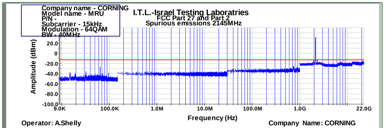
Figure 910: Spurious Emissions at Antenna Terminal 64QAM 40MHz B.W.; 2145.0MHz, 15kHz
