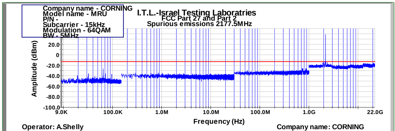
Figure 869: Spurious Emissions at Antenna Terminal 64QAM 5MHz B.W.; 2177.5MHz, 15kHz
