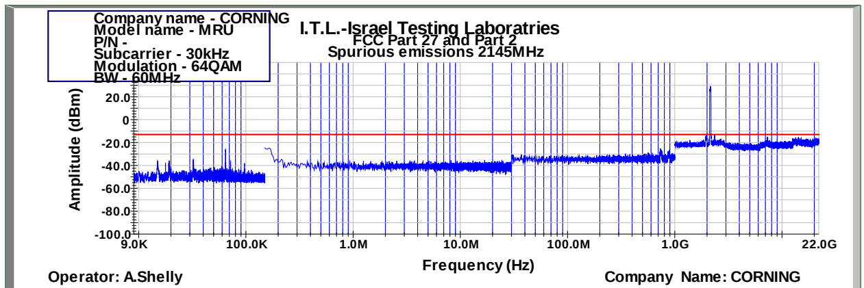
Figure 928: Spurious Emissions at Antenna Terminal 64QAM 60MHz B.W.; 2145.0MHz, 30kHz
