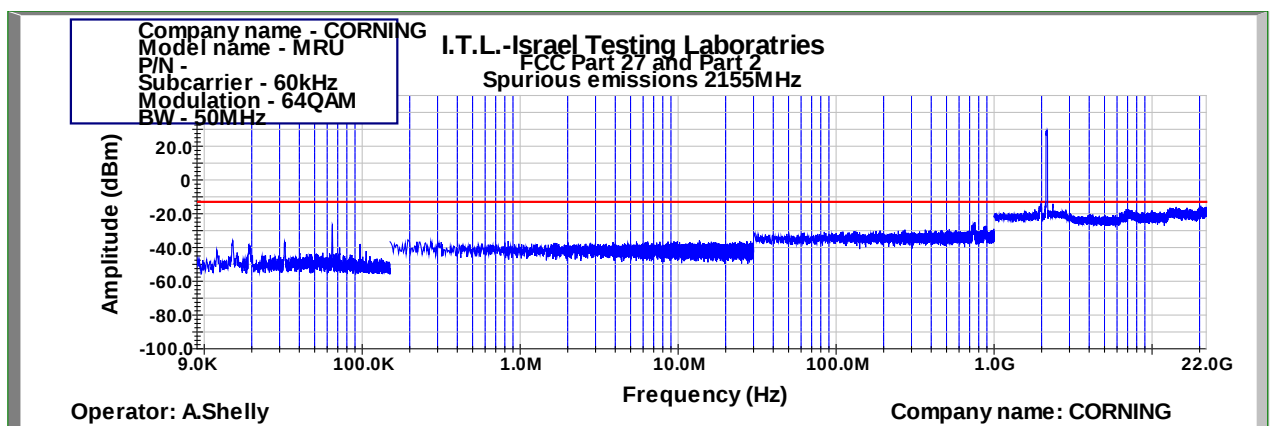
Figure 926: Spurious Emissions at Antenna Terminal 64QAM 50MHz B.W.; 2155.0MHz, 60kHz
