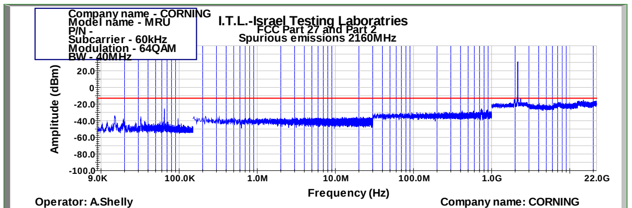
Figure 917: Spurious Emissions at Antenna Terminal 64QAM 40MHz B.W.; 2160.0MHz, 60kHz
