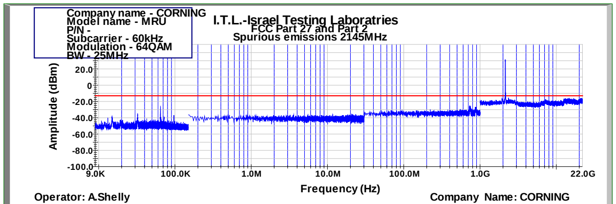
Figure 907: Spurious Emissions at Antenna Terminal 64QAM 25MHz B.W.; 2145.0MHz, 60kHz
