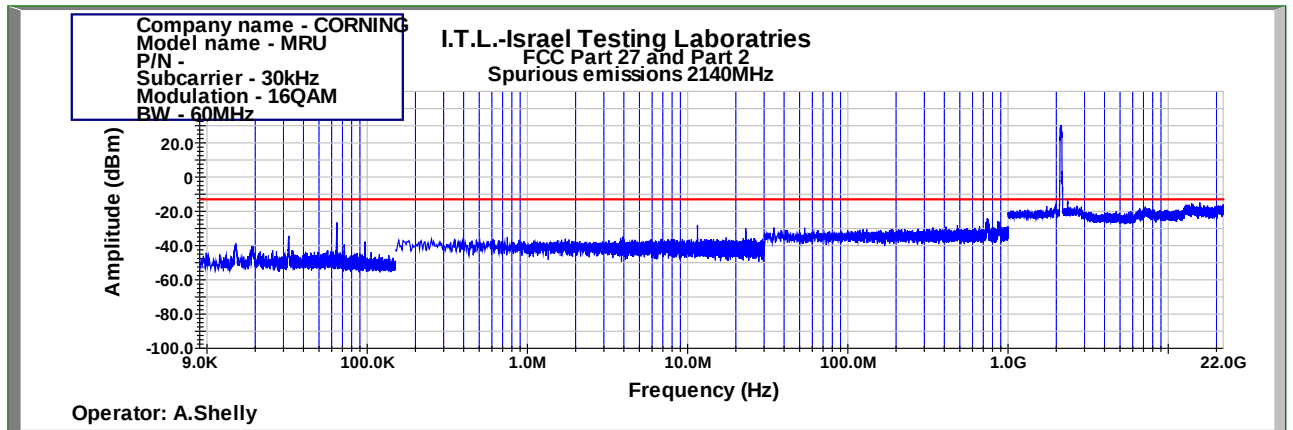
Figure 861: Spurious Emissions at Antenna Terminal 16QAM 60MHz B.W.; 2140.0MHz, 30kHz
