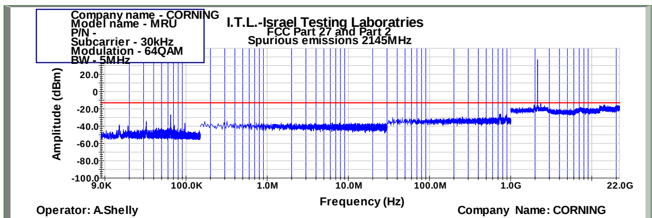
Figure 871: Spurious Emissions at Antenna Terminal 64QAM 5MHz B.W.; 2145.0MHz, 30kHz
