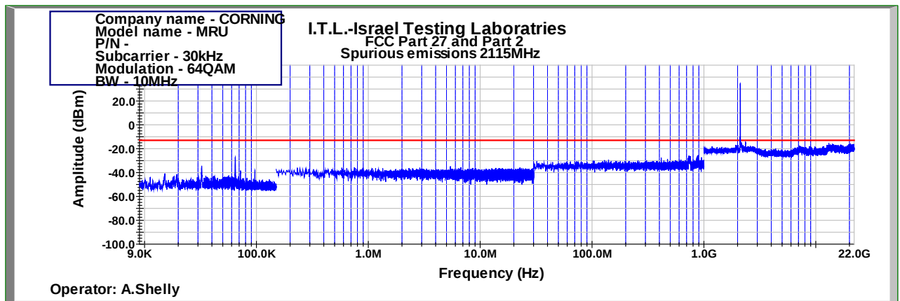
Figure 876: Spurious Emissions at Antenna Terminal 64QAM 10MHz B.W.; 2115.0MHz, 30kHz
