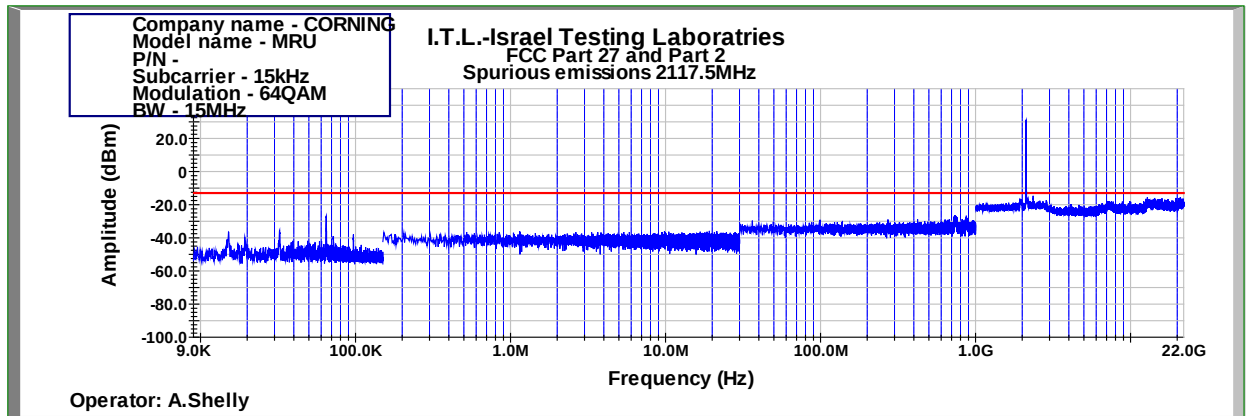
Figure 882: Spurious Emissions at Antenna Terminal 64QAM 15MHz B.W.; 2117.5MHz, 15kHz
