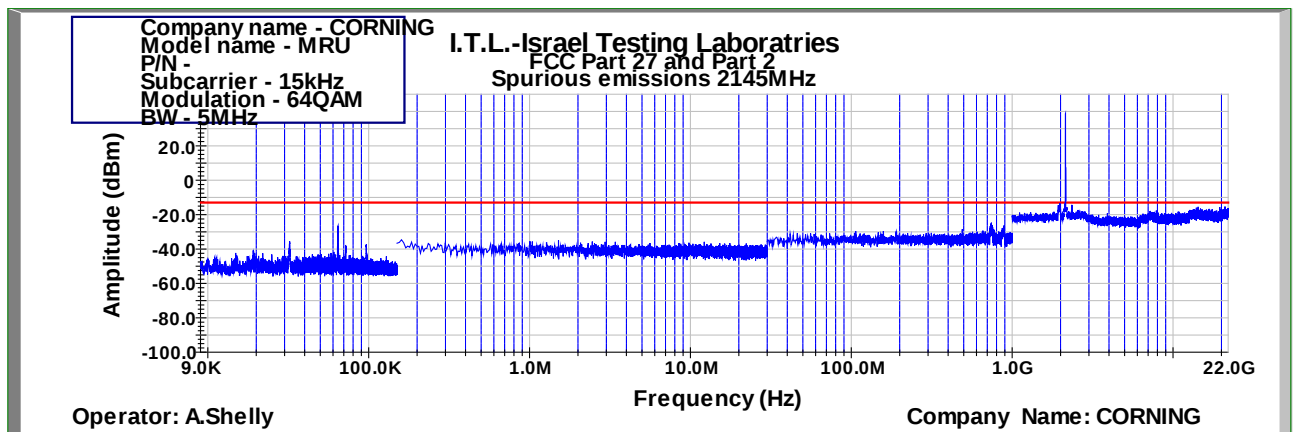
Figure 868: Spurious Emissions at Antenna Terminal 64QAM 5MHz B.W.; 2145.0MHz, 15kHz
