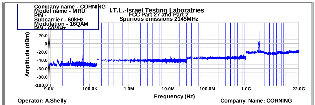
Figure 865: Spurious Emissions at Antenna Terminal 16QAM 60MHz B.W.; 2145.0MHz, 60kHz
