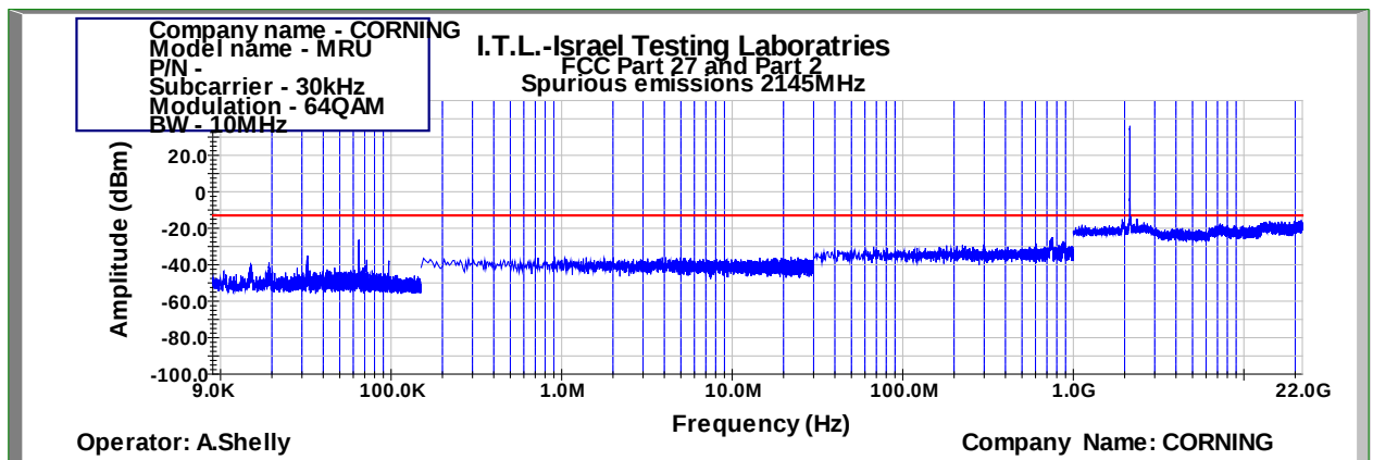
Figure 877: Spurious Emissions at Antenna Terminal 64QAM 10MHz B.W.; 2145.0MHz, 30kHz
