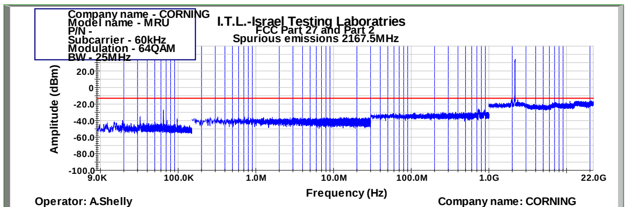
Figure 908: Spurious Emissions at Antenna Terminal 64QAM 25MHz B.W.; 2167.5MHz, 60kHz
