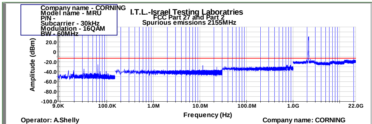
Figure 863: Spurious Emissions at Antenna Terminal 16QAM 60MHz B.W.; 2155.0MHz, 30kHz
