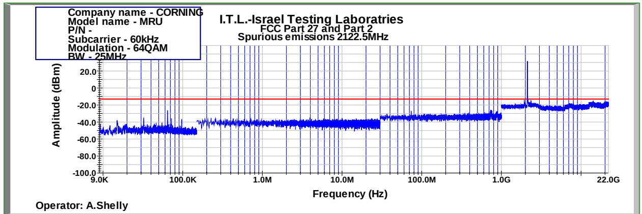
Figure 906: Spurious Emissions at Antenna Terminal 64QAM 25MHz B.W.; 2122.5MHz, 60kHz
