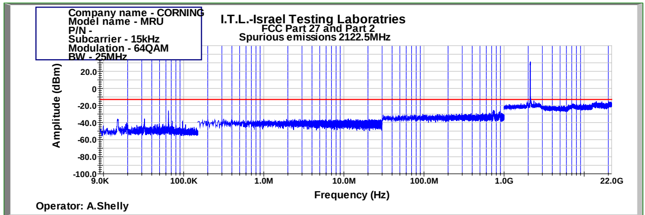
Figure 900: Spurious Emissions at Antenna Terminal 64QAM 25MHz B.W.; 2122.5MHz, 15kHz
