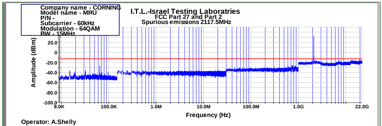
Figure 888: Spurious Emissions at Antenna Terminal 64QAM 15MHz B.W.; 2117.5MHz, 60kHz
