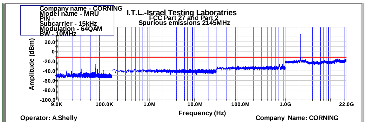
Figure 874: Spurious Emissions at Antenna Terminal 64QAM 10MHz B.W.; 2145.0MHz, 15kHz
