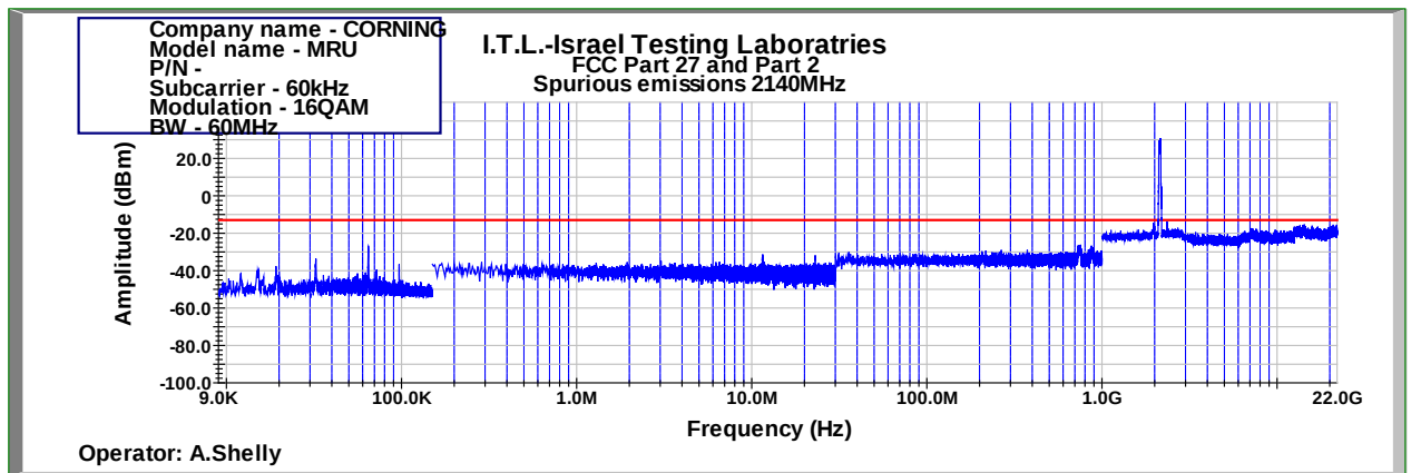
Figure 864: Spurious Emissions at Antenna Terminal 16QAM 60MHz B.W.; 2140.0MHz, 60kHz
