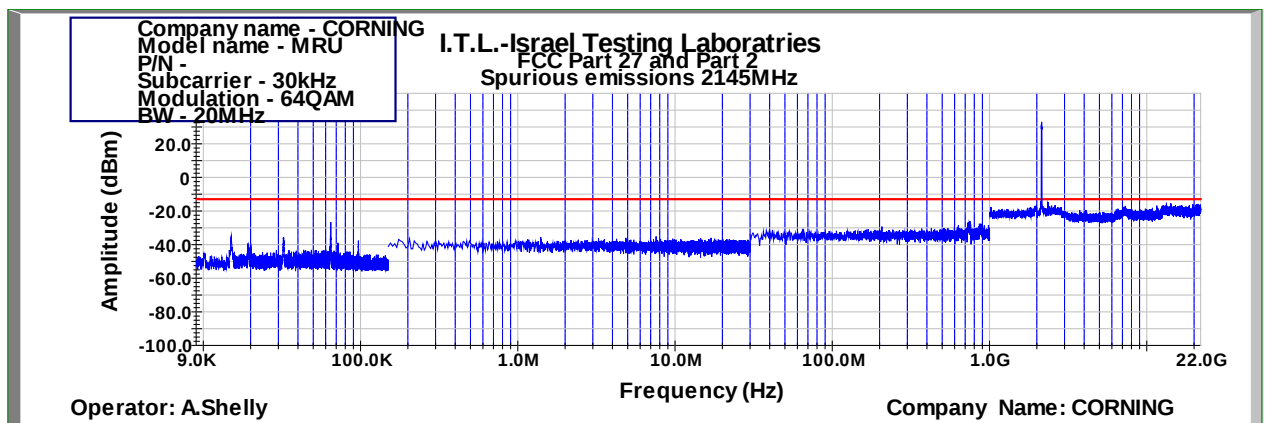
Figure 895: Spurious Emissions at Antenna Terminal 64QAM 20MHz B.W.; 2145.0MHz, 30kHz
