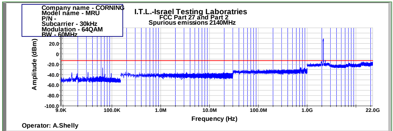
Figure 927: Spurious Emissions at Antenna Terminal 64QAM 60MHz B.W.; 2140.0MHz, 30kHz
