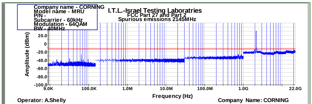
Figure 916: Spurious Emissions at Antenna Terminal 64QAM 40MHz B.W.; 2145.0MHz, 60kHz
