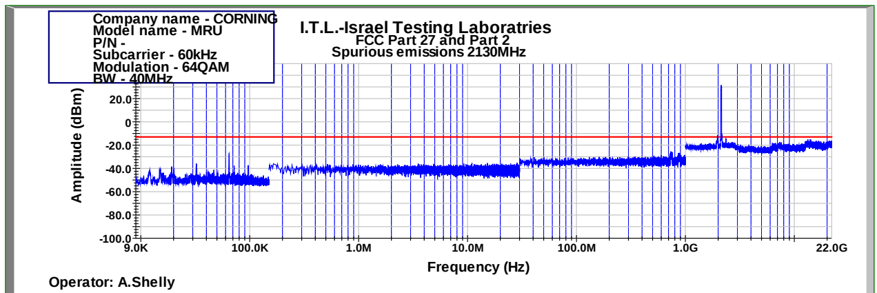
Figure 915: Spurious Emissions at Antenna Terminal 64QAM 40MHz B.W.; 2130.0MHz, 60kHz
