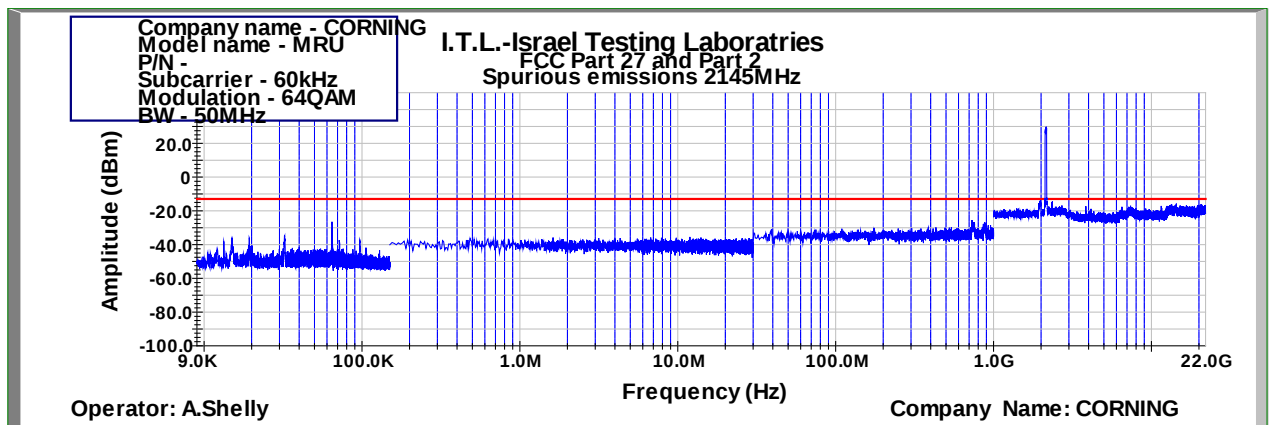
Figure 925: Spurious Emissions at Antenna Terminal 64QAM 50MHz B.W.; 2145.0MHz, 60kHz
