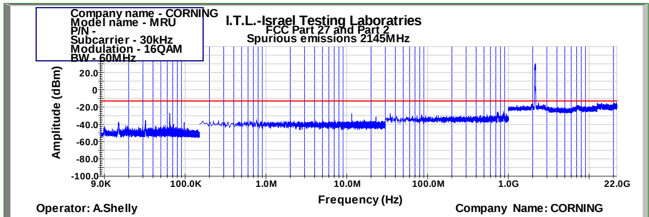
Figure 862: Spurious Emissions at Antenna Terminal 16QAM 60MHz B.W.; 2145.0MHz, 30kHz
