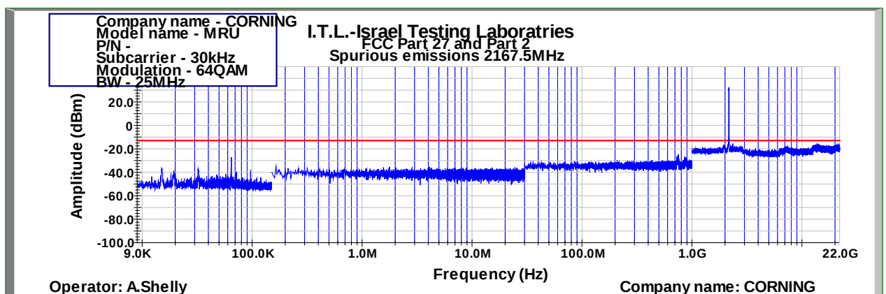
Figure 905: Spurious Emissions at Antenna Terminal 64QAM 25MHz B.W.; 2167.5MHz, 30kHz
