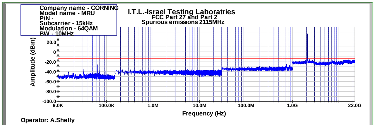
Figure 873: Spurious Emissions at Antenna Terminal 64QAM 10MHz B.W.; 2115.0MHz, 15kHz
