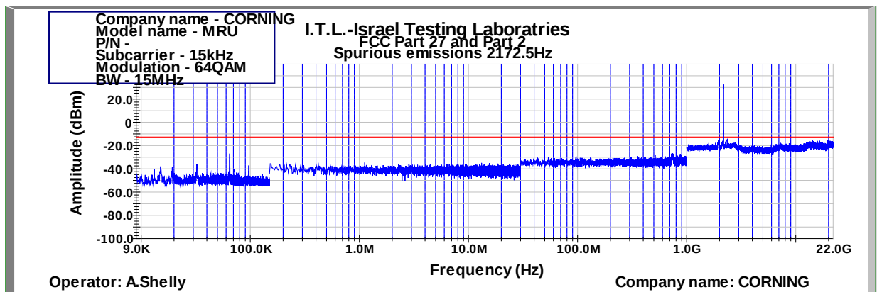
Figure 884: Spurious Emissions at Antenna Terminal 64QAM 15MHz B.W.; 2172.5MHz, 15kHz
