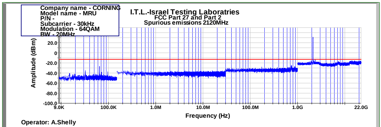
Figure 894: Spurious Emissions at Antenna Terminal 64QAM 20MHz B.W.; 2120.0MHz, 30kHz
