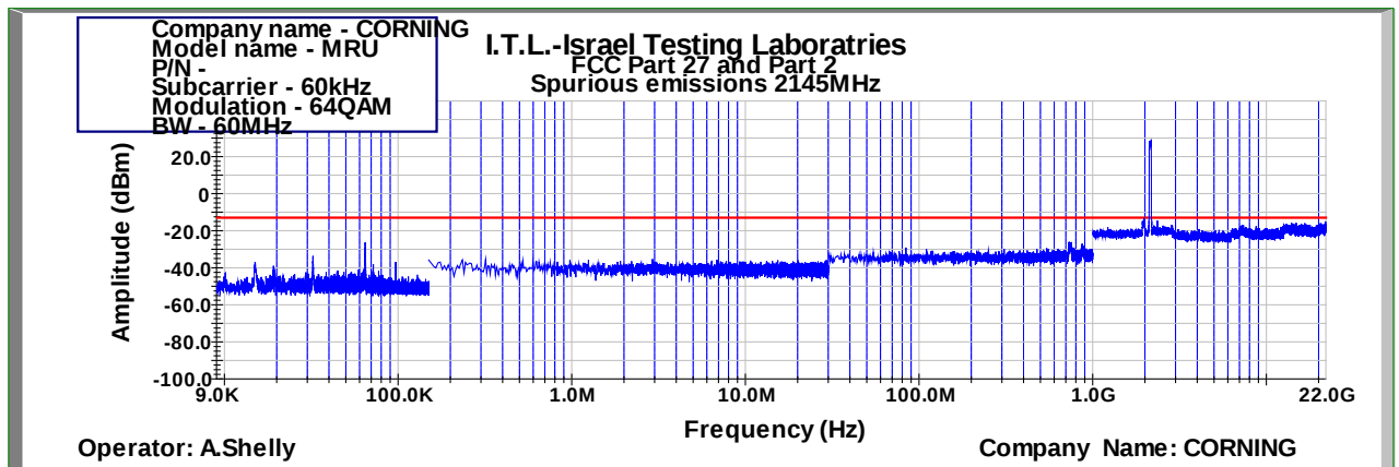
Figure 931: Spurious Emissions at Antenna Terminal 64QAM 60MHz B.W.; 2145.0MHz, 60kHz
