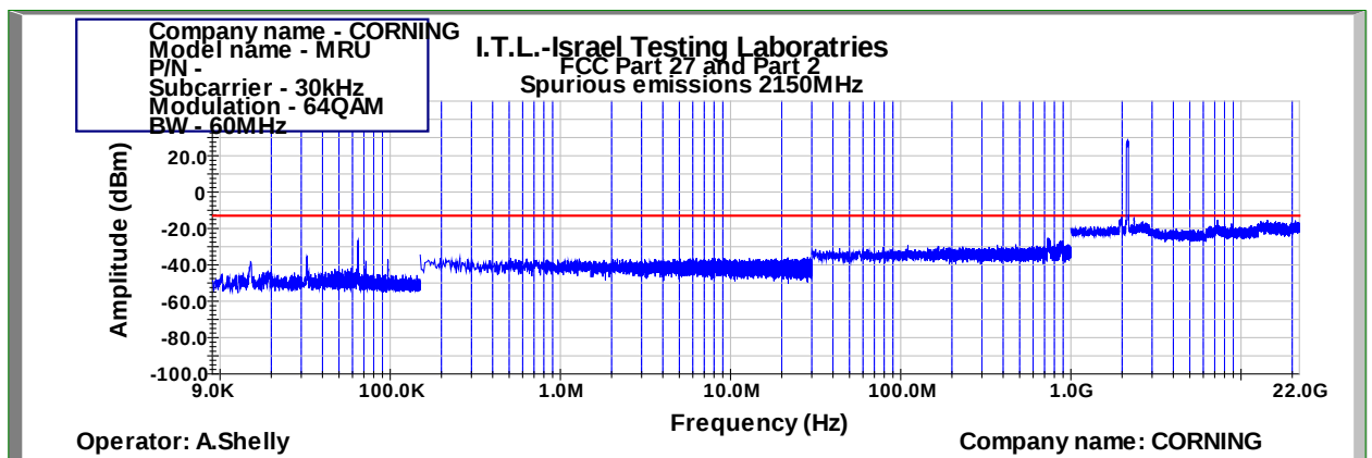
Figure 929: Spurious Emissions at Antenna Terminal 64QAM 60MHz B.W.; 2150.0MHz, 30kHz
