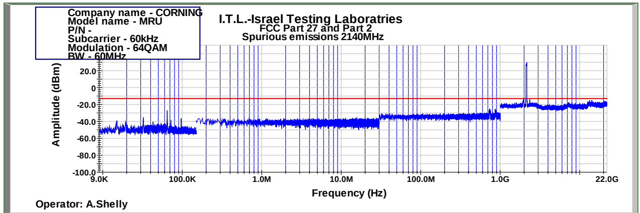
Figure 930: Spurious Emissions at Antenna Terminal 64QAM 60MHz B.W.; 2140.0MHz, 60kHz
