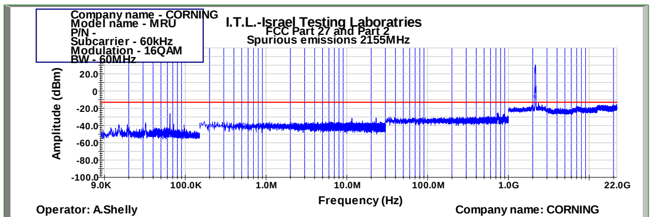
Figure 866: Spurious Emissions at Antenna Terminal 16QAM 60MHz B.W.; 2155.0MHz, 60kHz
