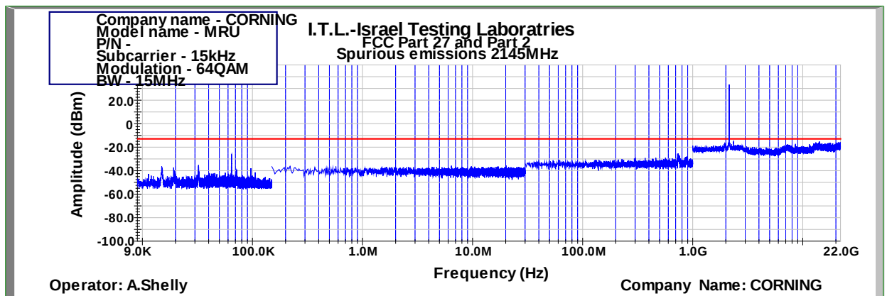
Figure 883: Spurious Emissions at Antenna Terminal 64QAM 15MHz B.W.; 2145.0MHz, 15kHz
