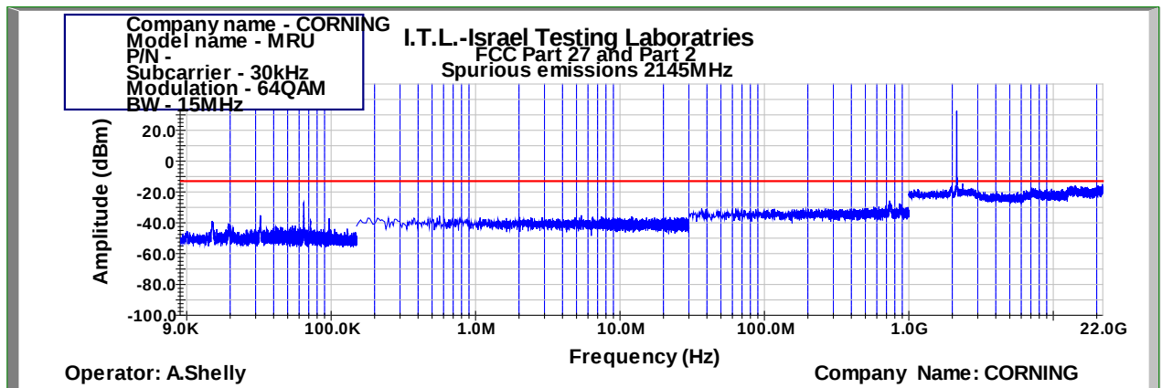
Figure 886: Spurious Emissions at Antenna Terminal 64QAM 15MHz B.W.; 2145.0MHz, 30kHz
