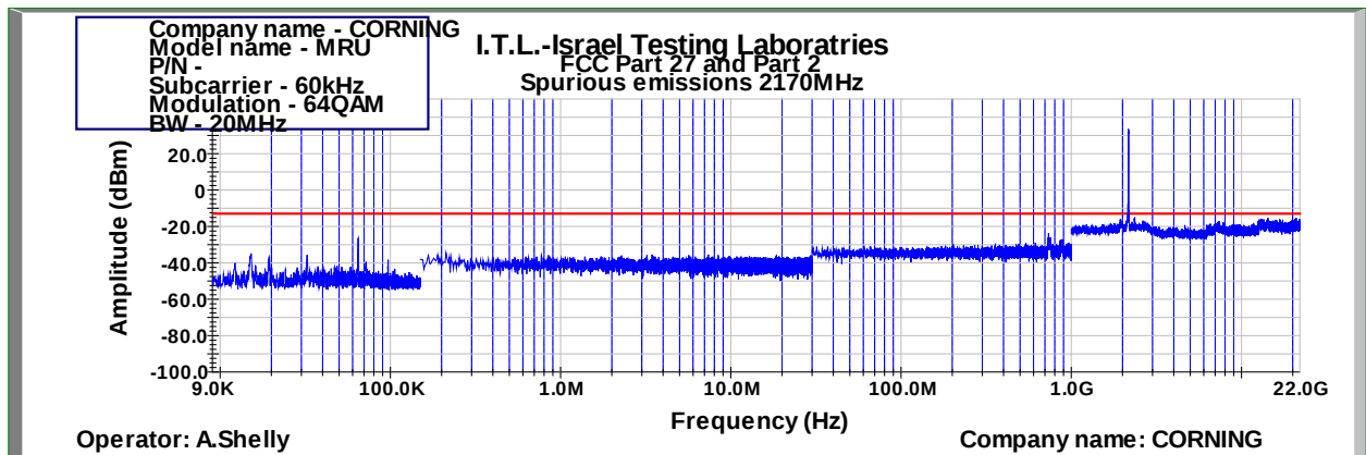
Figure 899: Spurious Emissions at Antenna Terminal 64QAM 20MHz B.W.; 2170.0MHz, 60kHz
