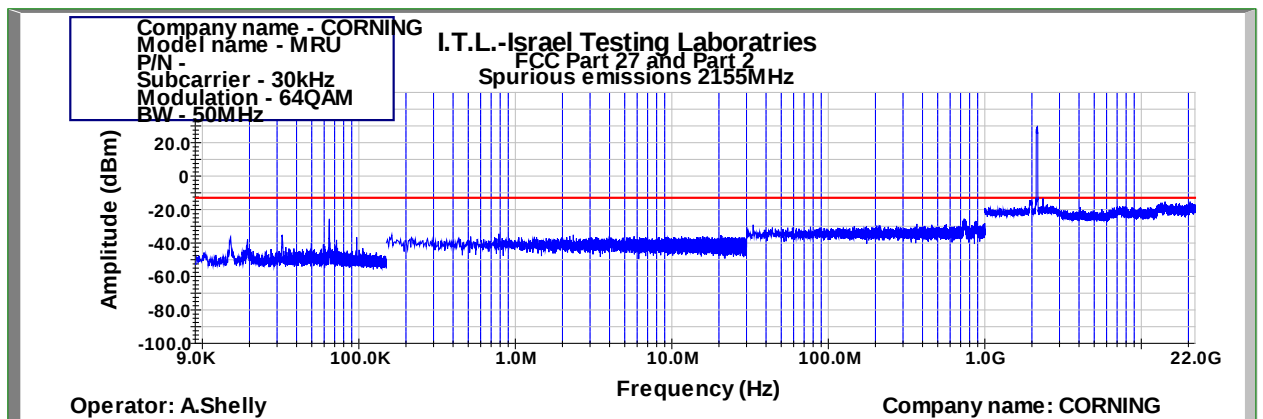
Figure 923: Spurious Emissions at Antenna Terminal 64QAM 50MHz B.W.; 2155.0MHz, 30kHz
