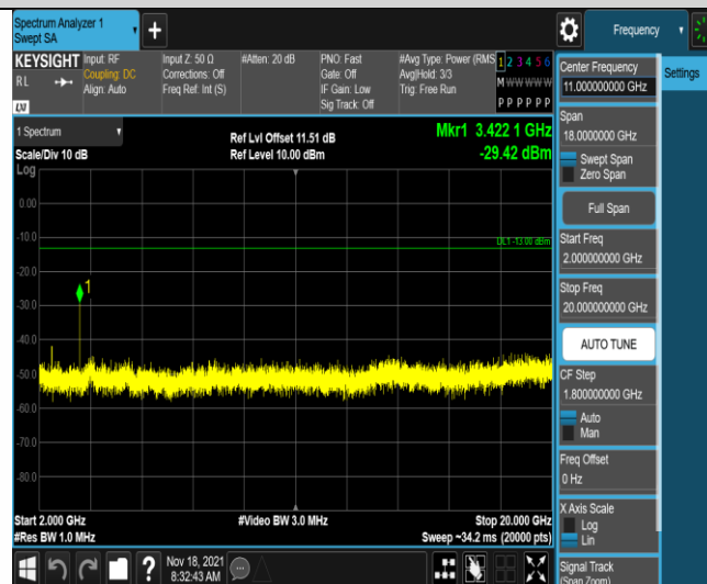
Band4-15MHz-QPSK-20025-1RB#0-Range3:2000~20000MHz
