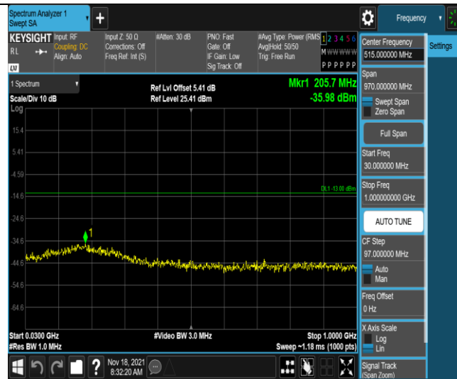
Band4-15MHz-QPSK-20025-1RB#0-Range1:30~1000MHz
