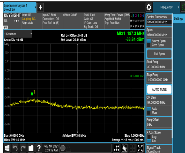
Band4-20MHz-QPSK-20300-1RB#0-Range1:30~1000MHz
