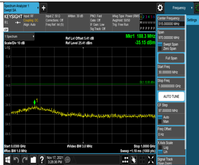
Band4-10MHz-QPSK-20175-1RB#0-Range1:30~1000MHz
