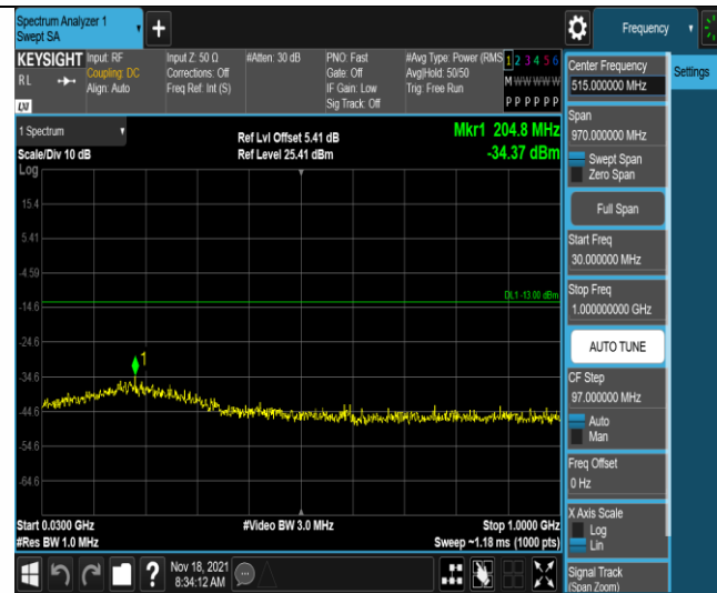
Band4-15MHz-16QAM-20175-1RB#0-Range1:30~1000MHz
