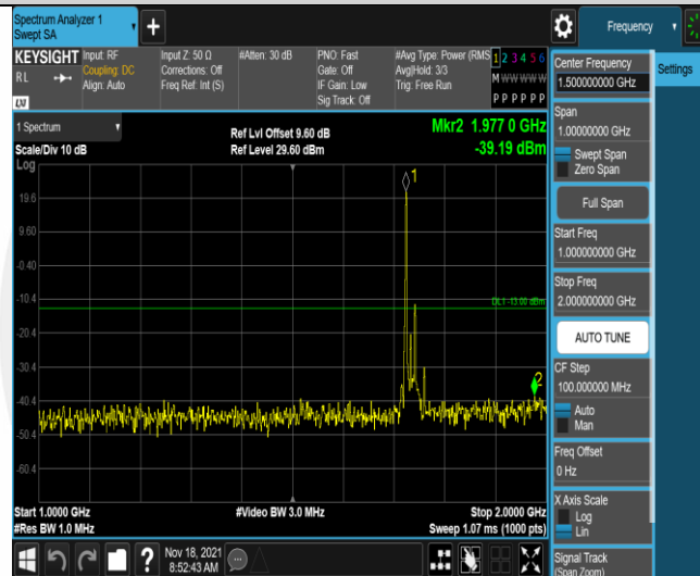
Band4-20MHz-16QAM-20175-1RB#0-Range2:1000~2000MHz
