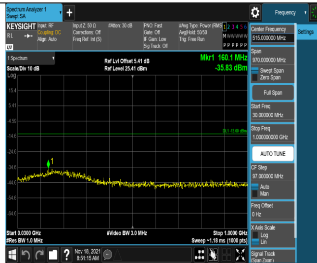
Band4-20MHz-16QAM-20050-1RB#0-Range1:30~1000MHz
