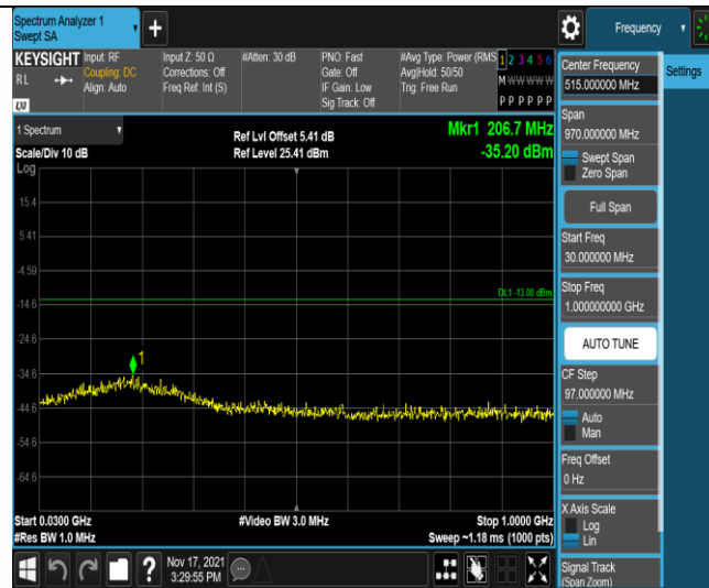
Band4-10MHz-QPSK-20350-1RB#0-Range1:30~1000MHz
