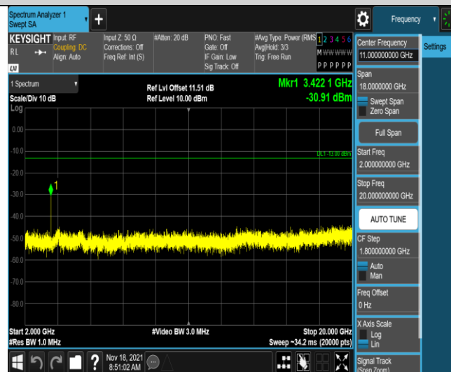
Band4-20MHz-QPSK-20050-1RB#0-Range3:2000~20000MHz
