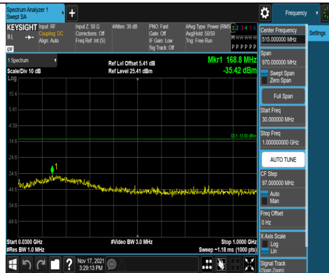
Band4-10MHz-16QAM-20175-1RB#0-Range1:30~1000MHz
