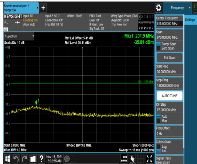
Band4-15MHz-16QAM-20025-1RB#0-Range1:30~1000MHz
