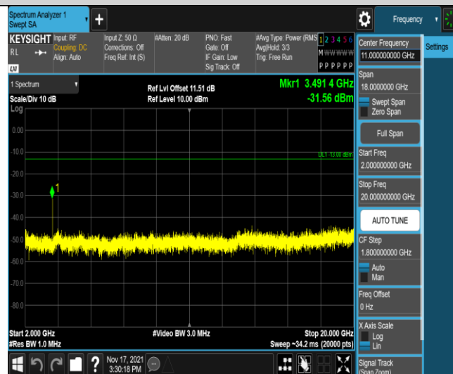
Band4-10MHz-QPSK-20350-1RB#0-Range3:2000~20000MHz
