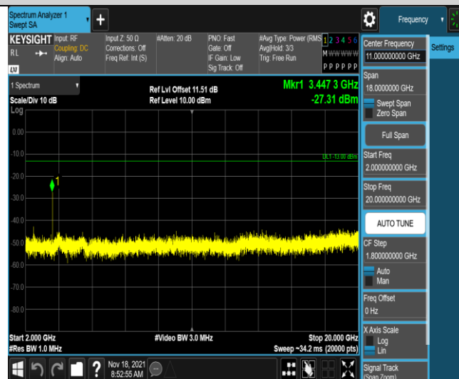
Band4-20MHz-16QAM-20175-1RB#0-Range3:2000~20000MHz
