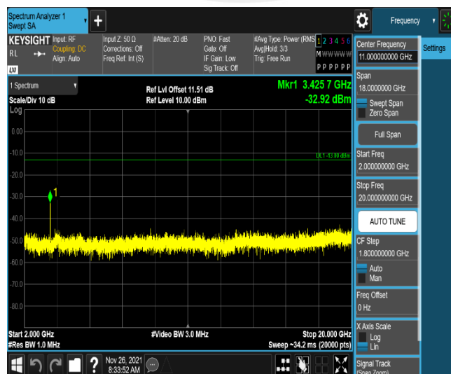
Band4-10MHz-16QAM-20175-1RB#0-Range3:2000~20000MHz
