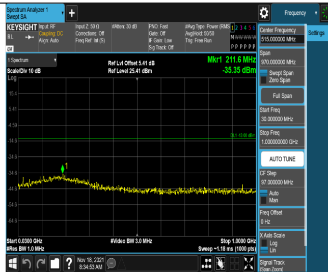
Band4-15MHz-QPSK-20325-1RB#0-Range1:30~1000MHz
