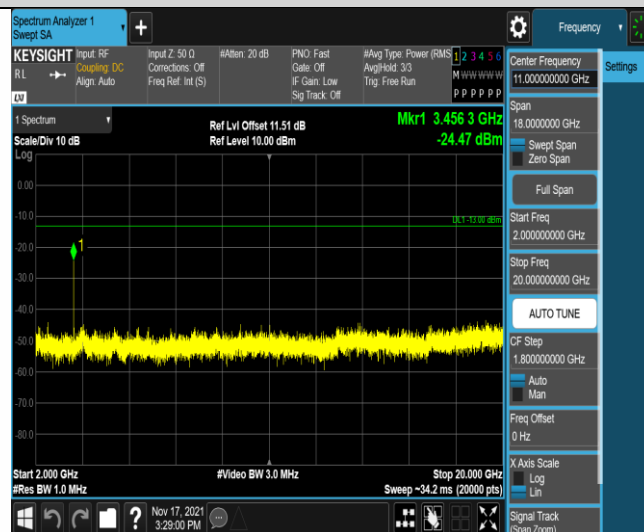
Band4-10MHz-QPSK-20175-1RB#0-Range3:2000~20000MHz
