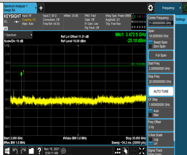
Band4-20MHz-16QAM-20300-1RB#0-Range3:2000~20000MHz
