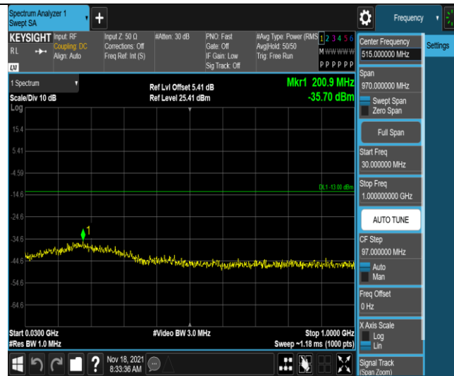
Band4-15MHz-QPSK-20175-1RB#0-Range1:30~1000MHz
