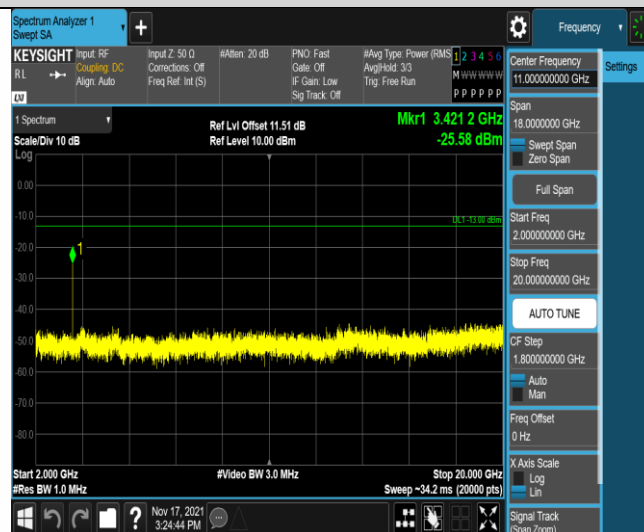
Band4-10MHz-QPSK-20000-1RB#0-Range3:2000~20000MHz
