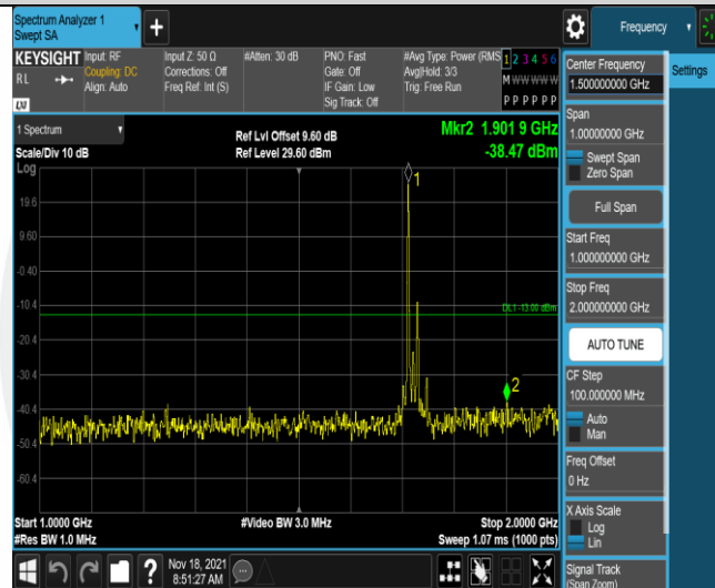
Band4-20MHz-16QAM-20050-1RB#0-Range2:1000~2000MHz
