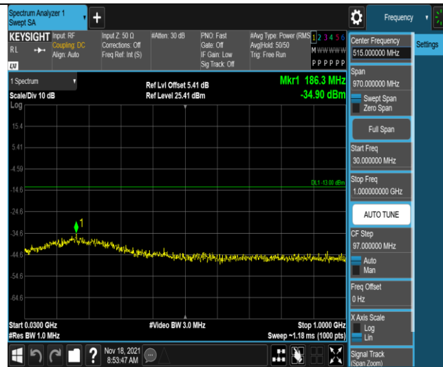
Band4-20MHz-16QAM-20300-1RB#0-Range1:30~1000MHz
