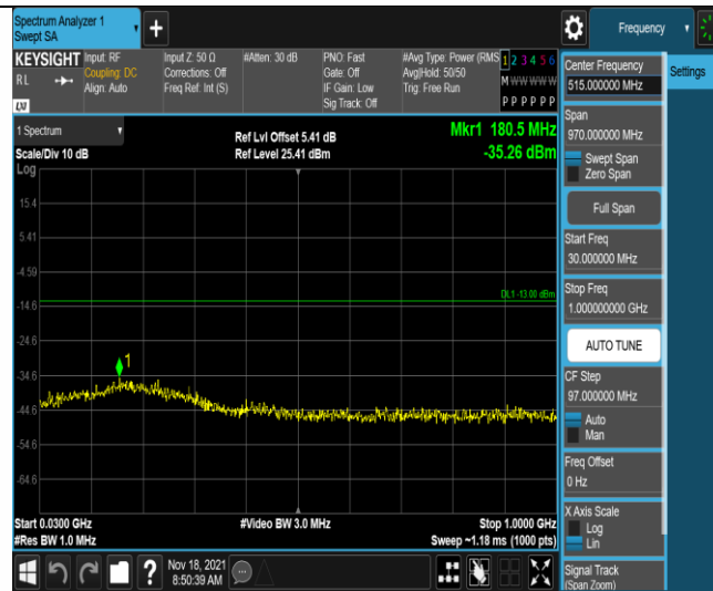
Band4-20MHz-QPSK-20050-1RB#0-Range1:30~1000MHz
