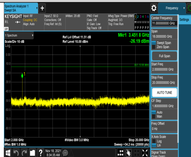
Band4-15MHz-16QAM-20175-1RB#0-Range3:2000~20000MHz
