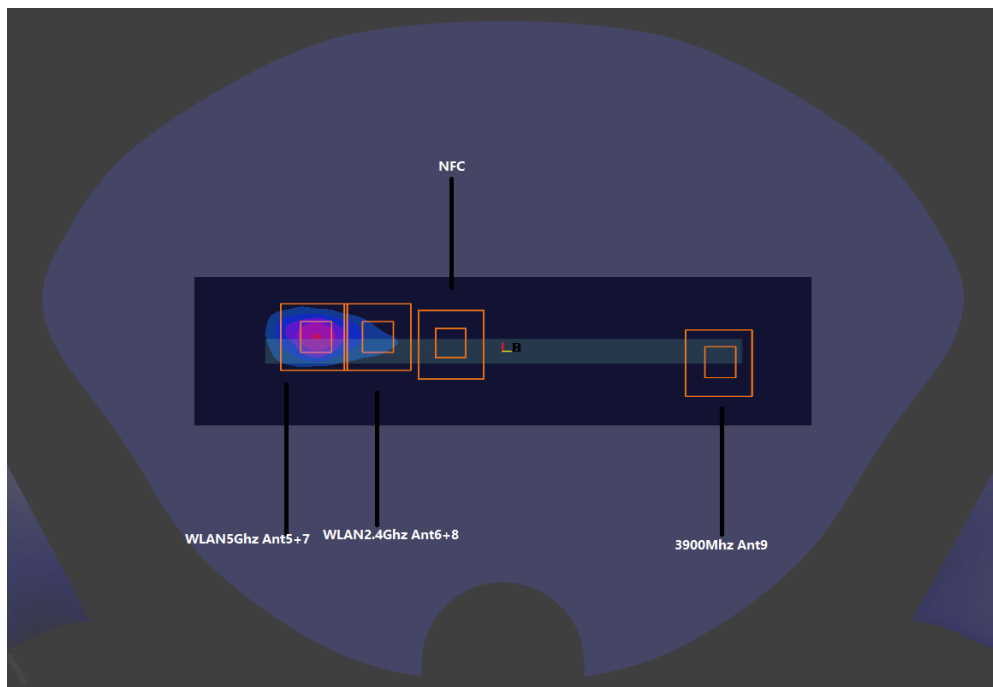
WWAN+ WLAN+ NFC _Right Side (0mm) for Extremity
