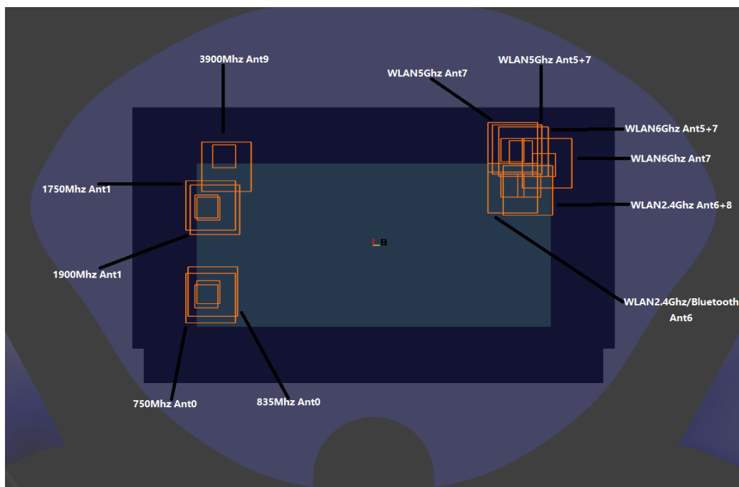
WWAN+ WLAN+ Bluetooth _Back (5mm) for Body-worn
