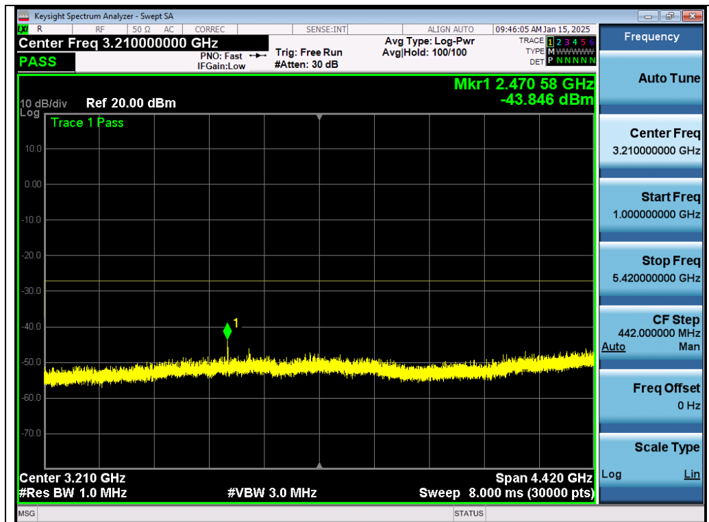
Test_Graph_802.11ac80_Chain B_5610_MCS0_Frequency Band 2
