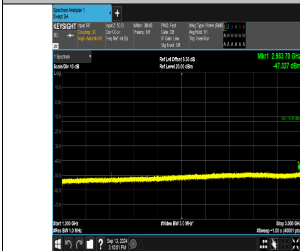
Band17_5MHz_16QAM_23790_1RB#0_1000~3000_1000~3000
