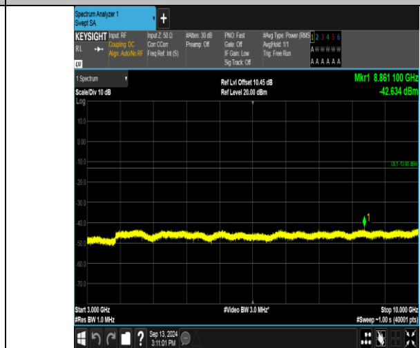
Band17_5MHz_16QAM_23790_1RB#0_3000~10000_3000~10000
