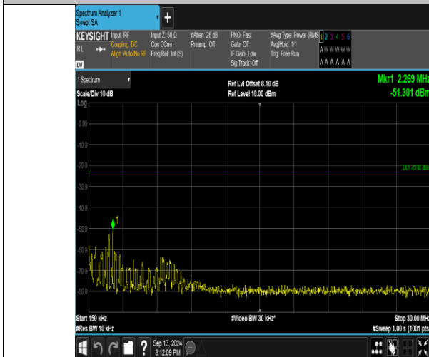
Band17_5MHz_16QAM_23790_1RB#24_0.15~30_0.15~30
