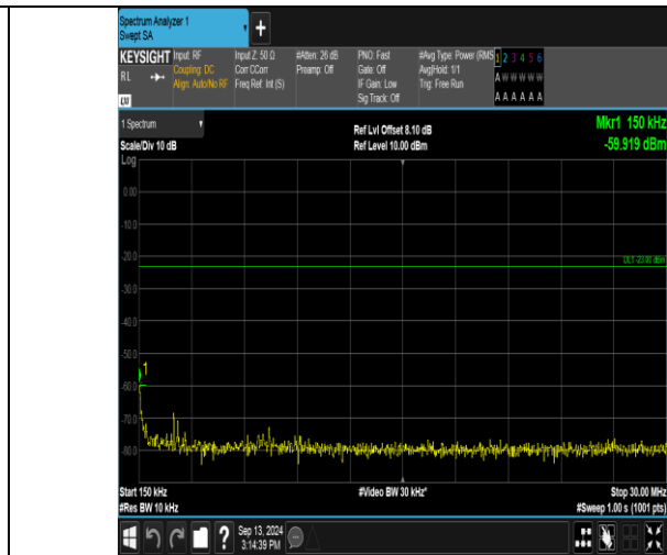
Band17_5MHz_QPSK_23825_1RB#0_0.15-30_0.15-30
