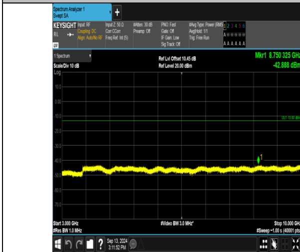
Band17_5MHz_QPSK_23790_1RB#24_3000~10000_3000~10000
