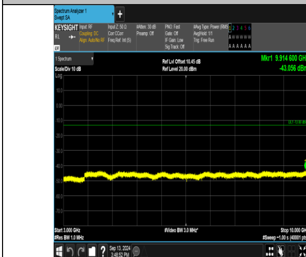
Band17_10MHz_QPSK_23780_1RB#0_3000~10000_3000~10000
