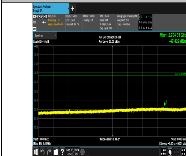
Band17_5MHz_16QAM_23790_25RB#0_1000~3000_1000~3000
