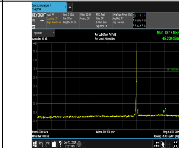
Band17_5MHz_16QAM_23790_1RB#24_30~1000_30~1000
