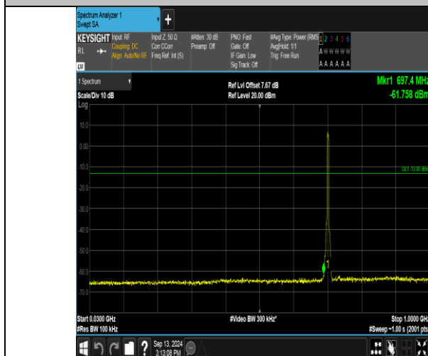
Band17_5MHz_QPSK_23790_25RB#0_30~1000_30~1000
