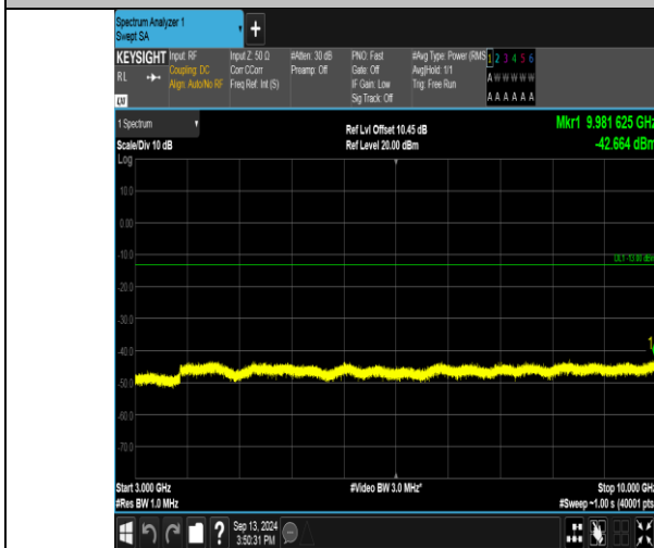
Band17_10MHz_QPSK_23780_1RB#49_3000~10000_3000~10000
