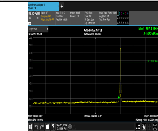
Band17_5MHz_16QAM_23790_25RB#0_30~1000_30~1000
