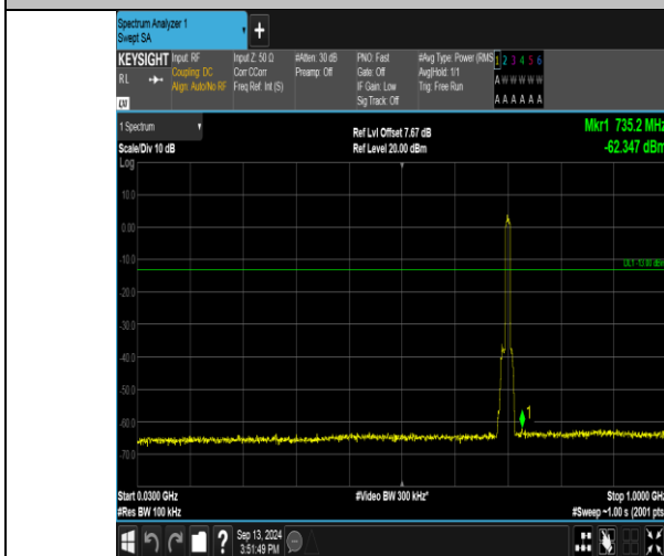
Band17_10MHz_QPSK_23780_50RB#0_30~1000_30~1000
