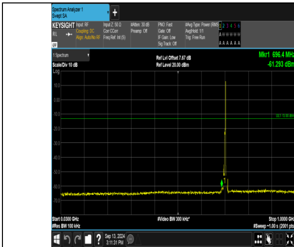
Band17_5MHz_QPSK_23790_1RB#24_30~1000_30~1000
