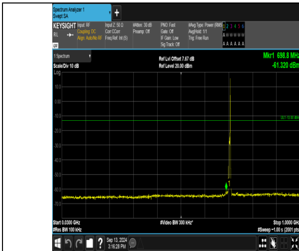
Band17_5MHz_QPSK_23825_1RB#24_30~1000_30~1000
