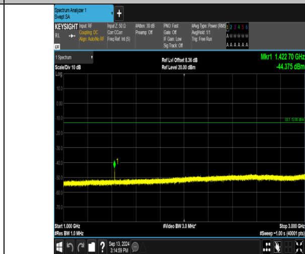
Band17_5MHz_QPSK_23825_1RB#0_1000-3000_1000-3000
