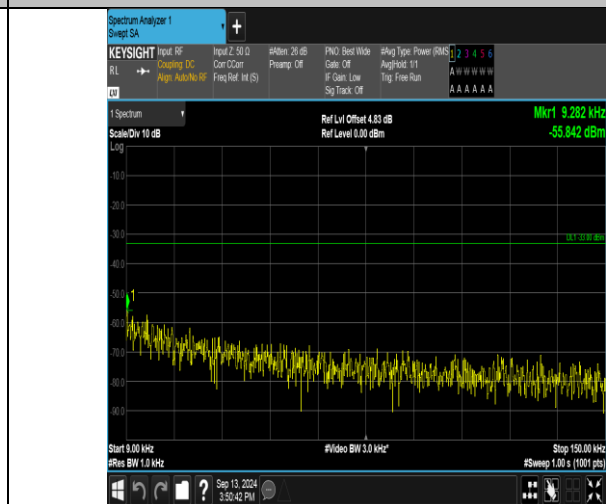
Band17_10MHz_16QAM_23780_1RB#49_0.009~0.15_0.009~0.15
