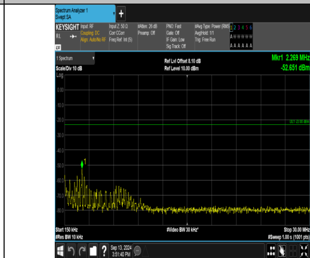
Band17_10MHz_QPSK_23780_50RB#0_0.15~30_0.15~30
