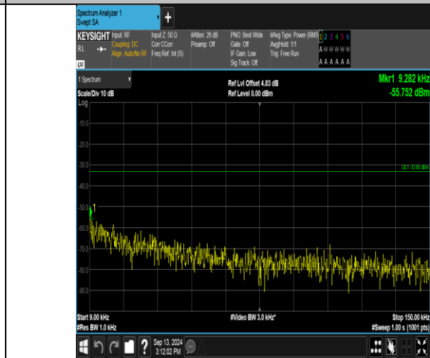
Band17_5MHz_16QAM_23790_1RB#24_0.009~0.15_0.009~0.15
