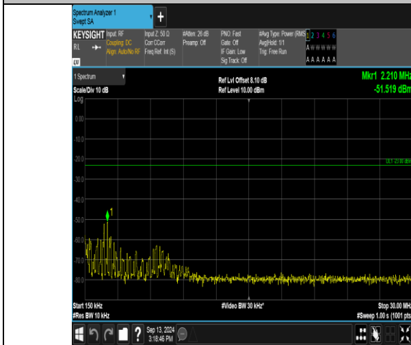
Band17_5MHz_16QAM_23825_25RB#0_0.15~30_0.15~30
