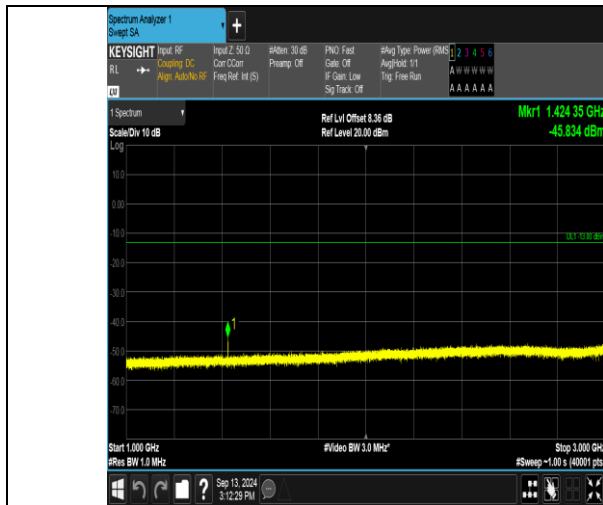
Band17_5MHz_16QAM_23790_1RB#24_1000~3000_1000~3000
