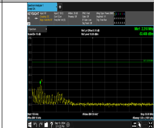
Band17_5MHz_QPSK_23790_1RB#24_0.15~30_0.15~30
