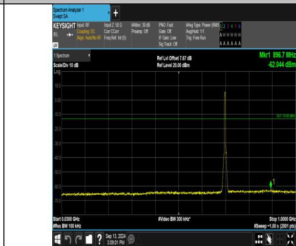
Band17_5MHz_16QAM_23755_25RB#0_30~1000_30~1000
