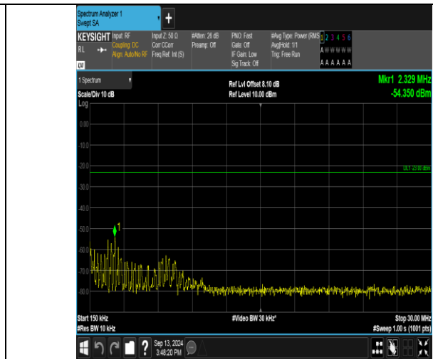
Band17_10MHz_QPSK_23780_1RB#0_0.15~30_0.15~30
