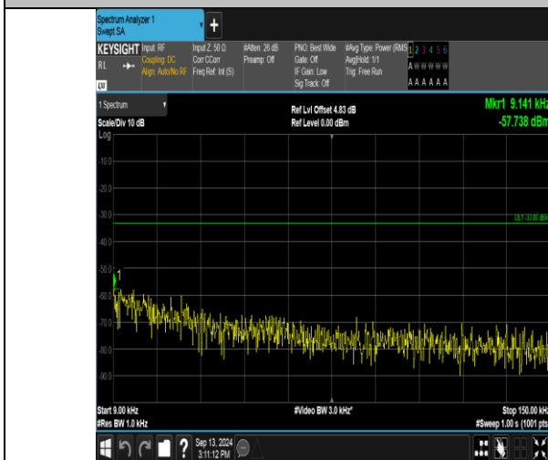
Band17_5MHz_QPSK_23790_1RB#24_0.009~0.15_0.009~0.15
