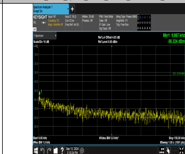
Band17_5MHz_16QAM_23790_1RB#0_0.009~0.15_0.009~0.15
