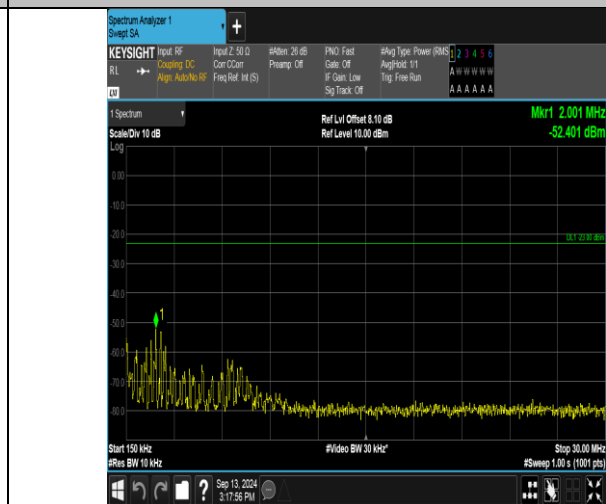
Band17_5MHz_QPSK_23825_25RB#0_0.15~30_0.15~30
