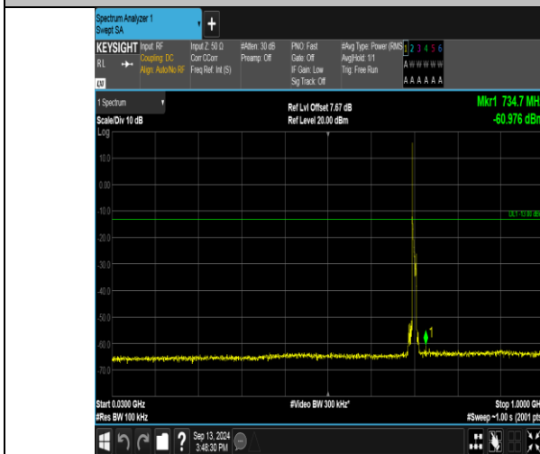
Band17_10MHz_QPSK_23780_1RB#0_30~1000_30~1000
