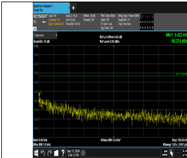
Band17_10MHz_QPSK_23780_1RB#0_0.009~0.15_0.009~0.15
