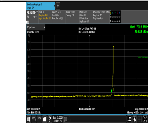
Band17_5MHz_16QAM_23825_25RB#0_30~1000_30~1000
