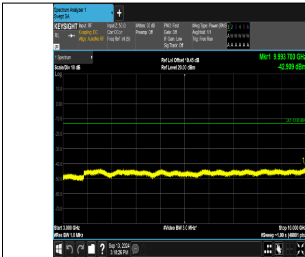
Band17_5MHz_QPSK_23825_25RB#0_3000~10000_3000~10000
