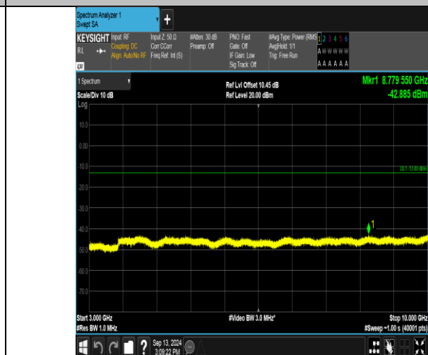
Band17_5MHz_16QAM_23755_25RB#0_3000~10000_3000~10000
