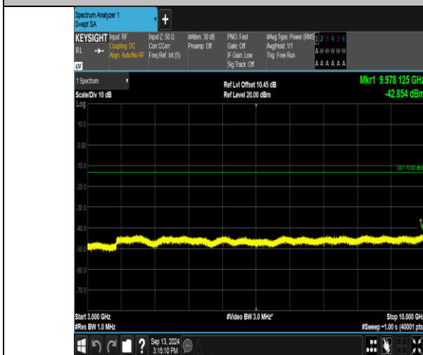
Band17_5MHz_QPSK_23825_1RB#0_3000-10000_3000-10000
