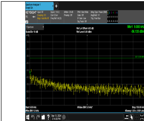
Band17_5MHz_QPSK_23825_1RB#0_0.009-0.15_0.009-0.15
