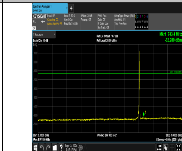
Band17_5MHz_16QAM_23825_1RB#24_30~1000_30~1000
