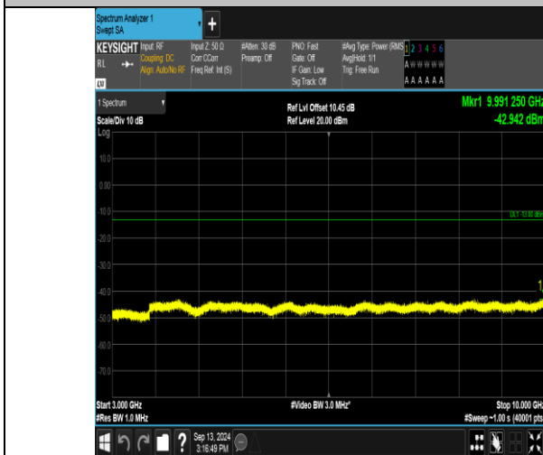
Band17_5MHz_QPSK_23825_1RB#24_3000~10000_3000~10000
