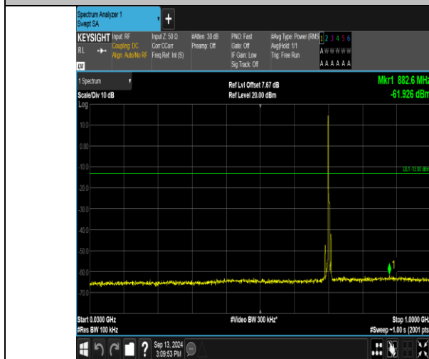
Band17_5MHz_QPSK_23790_1RB#0_30~1000_30~1000
