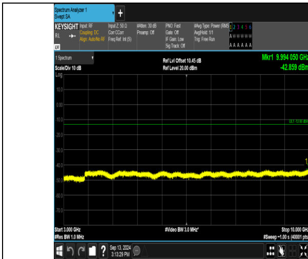
Band17_5MHz_QPSK_23790_25RB#0_3000~10000_3000~10000
