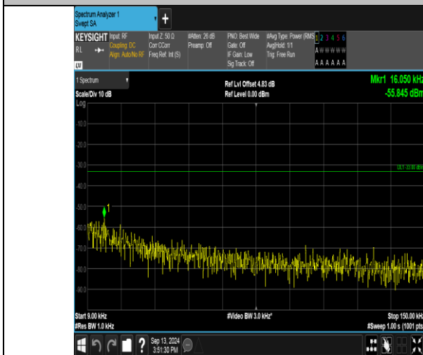
Band17_10MHz_QPSK_23780_50RB#0_0.009~0.15_0.009~0.15
