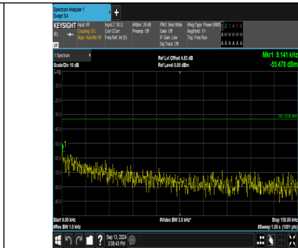
Band17_5MHz_16QAM_23755_25RB#0_0.009~0.15_0.009~0.15
