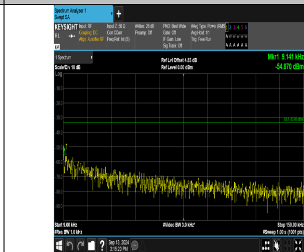
Band17_5MHz_16QAM_23825_1RB#0_0.009-0.15_0.009-0.15
