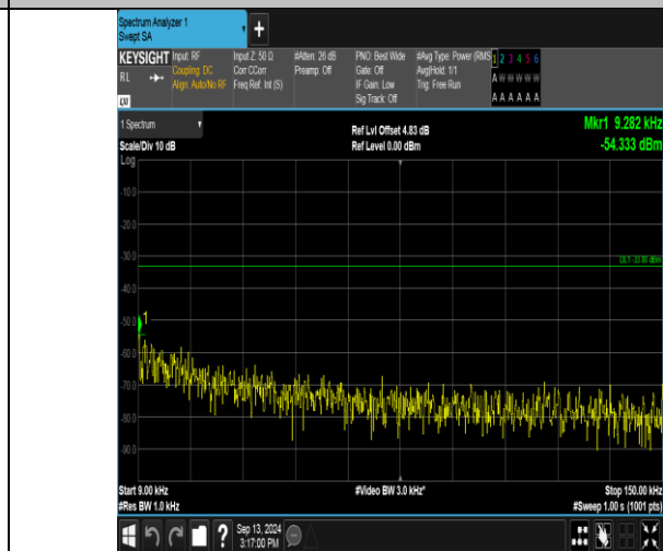
Band17_5MHz_16QAM_23825_1RB#24_0.009~0.15_0.009~0.15
