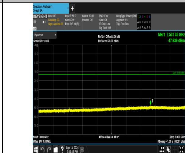
Band17_5MHz_QPSK_23790_25RB#0_1000~3000_1000~3000
