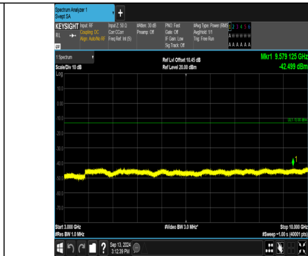
Band17_5MHz_16QAM_23790_1RB#24_3000~10000_3000~10000
