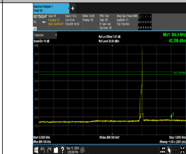
Band17_10MHz_16QAM_23780_1RB#49_30~1000_30~1000
