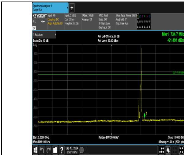
Band17_10MHz_QPSK_23780_1RB#49_30~1000_30~1000
