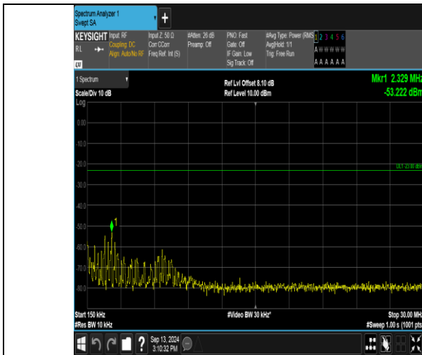
Band17_5MHz_16QAM_23790_1RB#0_0.15~30_0.15~30
