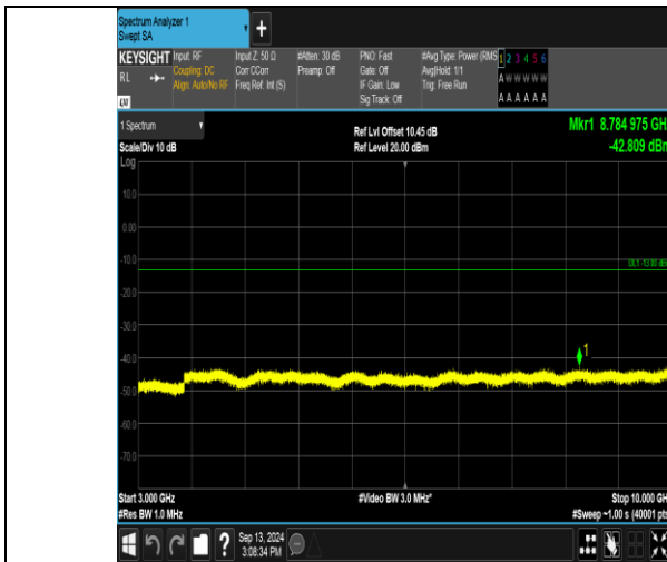
Band17_5MHz_QPSK_23755_25RB#0_3000~10000_3000~10000
