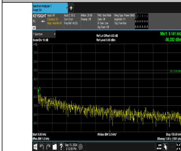
Band17_5MHz_QPSK_23790_25RB#0_0.009~0.15_0.009~0.15
