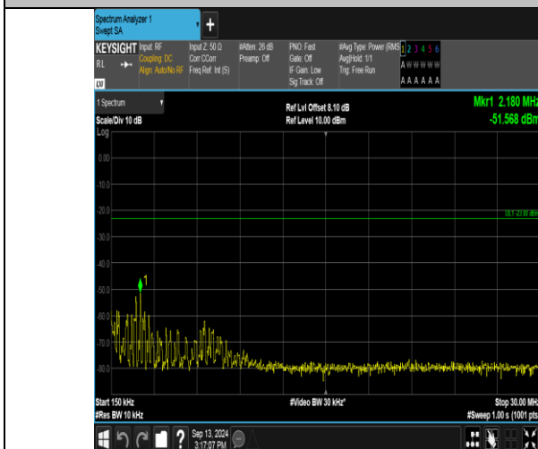
Band17_5MHz_16QAM_23825_1RB#24_0.15~30_0.15~30
