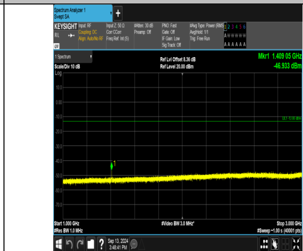
Band17_10MHz_QPSK_23780_1RB#0_1000~3000_1000~3000
