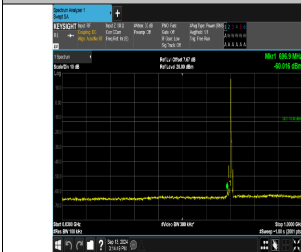
Band17_5MHz_QPSK_23825_1RB#0_30-1000_30-1000
