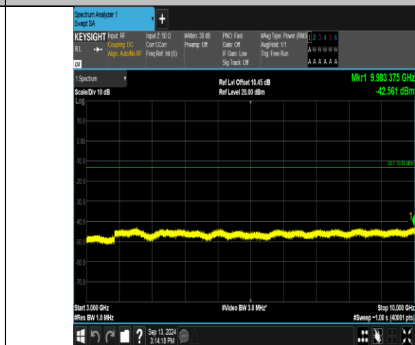
Band17_5MHz_16QAM_23790_25RB#0_3000~10000_3000~10000
