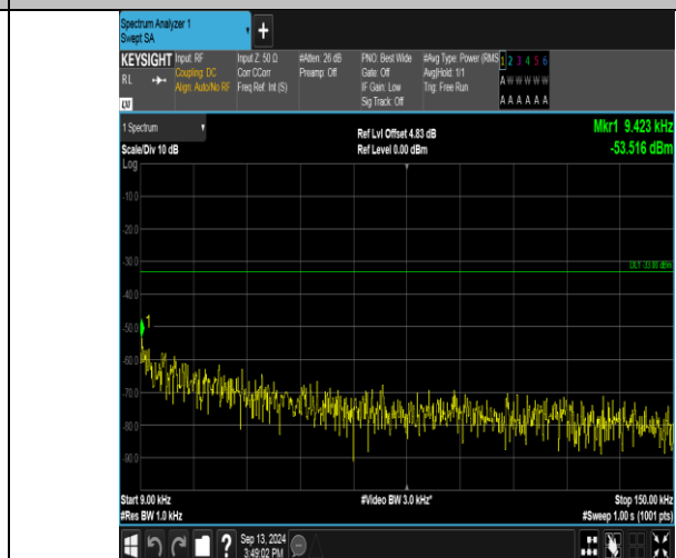
Band17_10MHz_16QAM_23780_1RB#0_0.009~0.15_0.009~0.15
