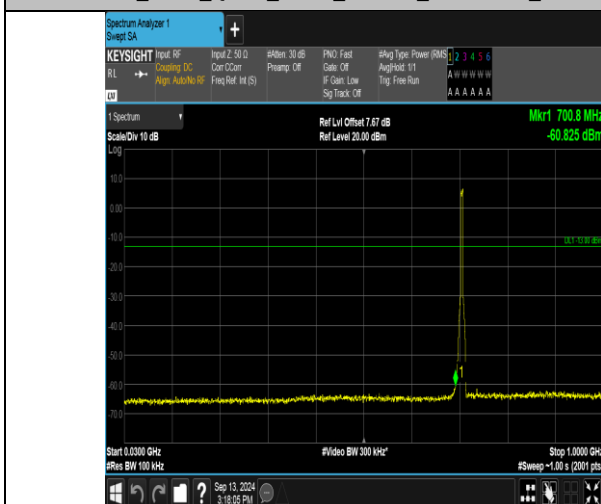
Band17_5MHz_QPSK_23825_25RB#0_30~1000_30~1000
