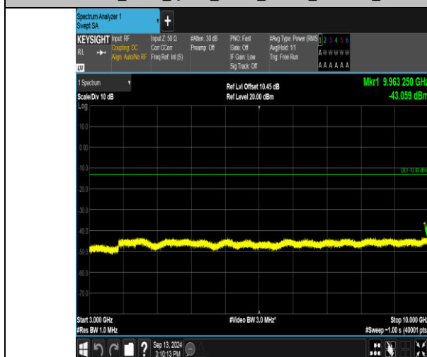
Band17_5MHz_QPSK_23790_1RB#0_3000~10000_3000~10000
