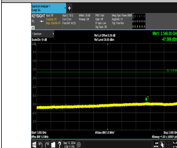
Band17_5MHz_16QAM_23755_25RB#0_1000~3000_1000~3000
