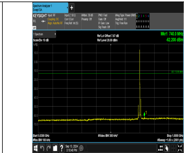
Band17_5MHz_16QAM_23790_1RB#0_30~1000_30~1000
