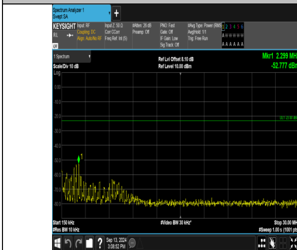
Band17_5MHz_16QAM_23755_25RB#0_0.15~30_0.15~30
