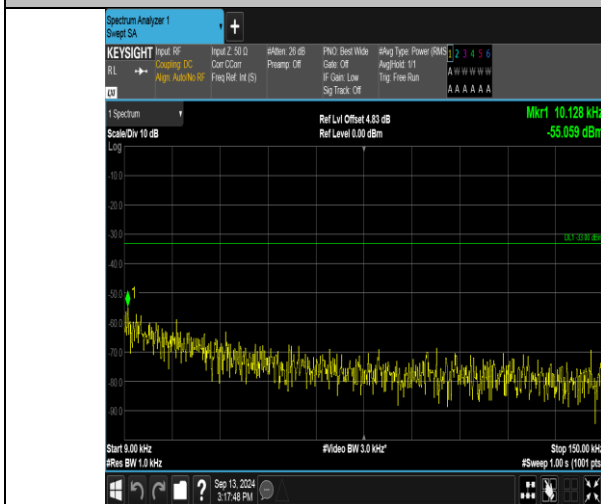
Band17_5MHz_QPSK_23825_25RB#0_0.009~0.15_0.009~0.15
