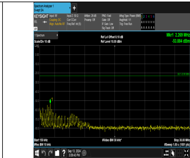
Band17_5MHz_QPSK_23790_1RB#0_0.15~30_0.15~30
