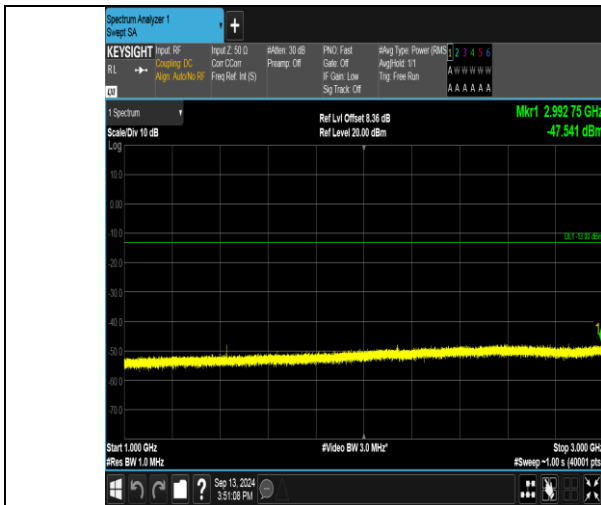
Band17_10MHz_16QAM_23780_1RB#49_1000~3000_1000~3000
