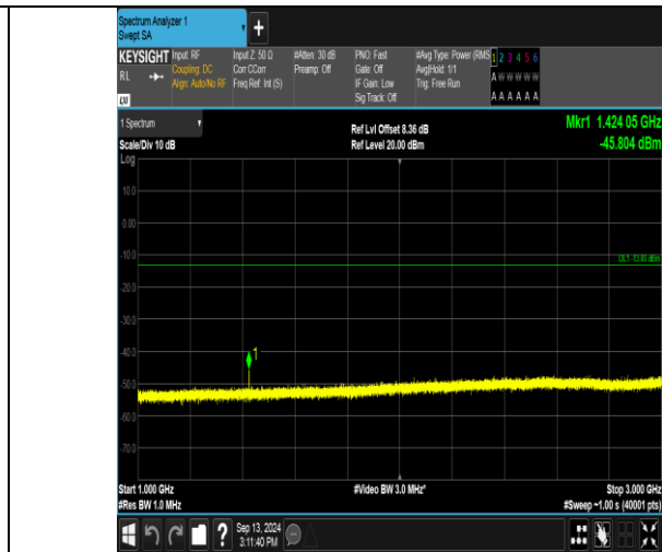
Band17_5MHz_QPSK_23790_1RB#24_1000~3000_1000~3000
