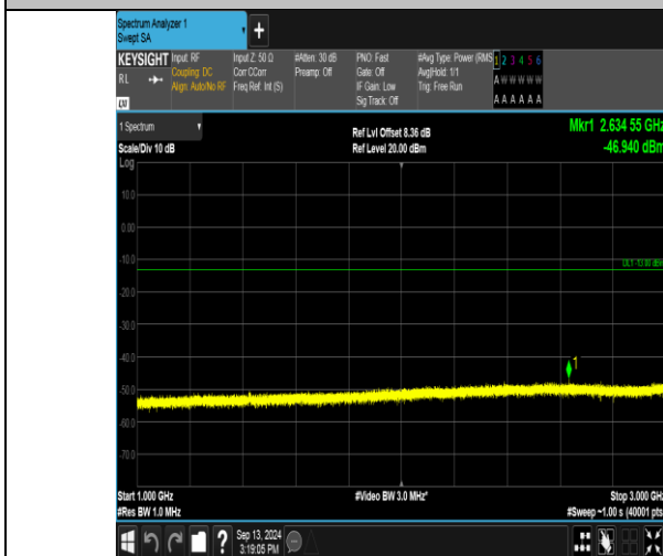
Band17_5MHz_16QAM_23825_25RB#0_1000~3000_1000~3000
