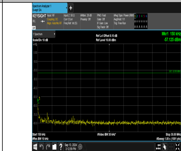
Band17_5MHz_QPSK_23790_25RB#0_0.15~30_0.15~30
