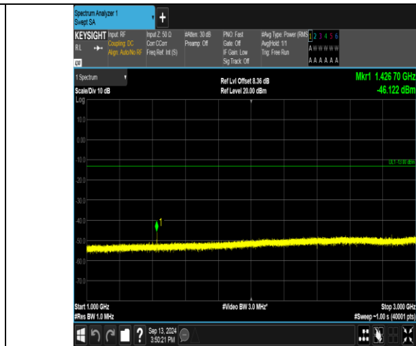
Band17_10MHz_QPSK_23780_1RB#49_1000~3000_1000~3000
