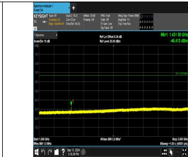
Band17_5MHz_QPSK_23825_1RB#24_1000~3000_1000~3000
