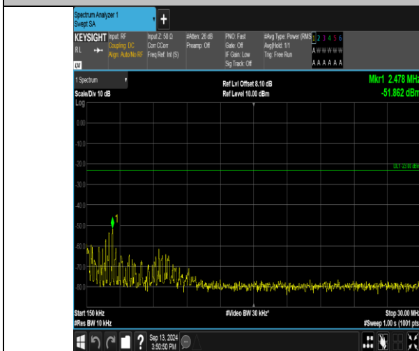
Band17_10MHz_16QAM_23780_1RB#49_0.15~30_0.15~30
