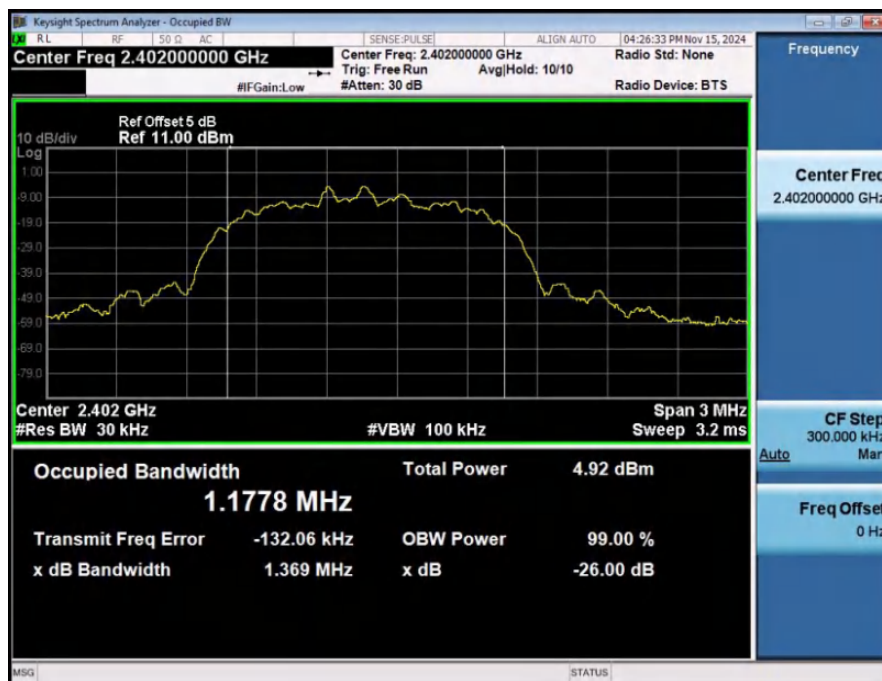
99%_Occupied_Bandwidth_NVNT_ANT1_3-DH5_2402_00
