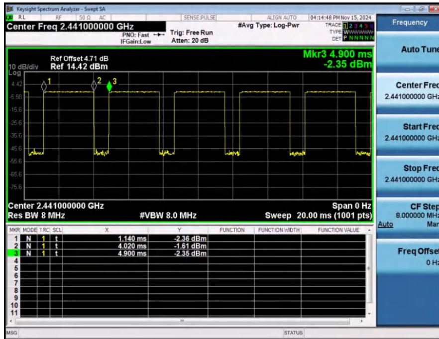
Duty_Cycle_NVNT_ANT1_2-DH5_2441
