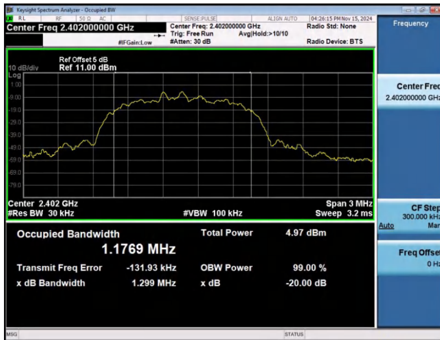
-20dB_Bandwidth_NVNT_ANT1_3-DH5_2402_00
