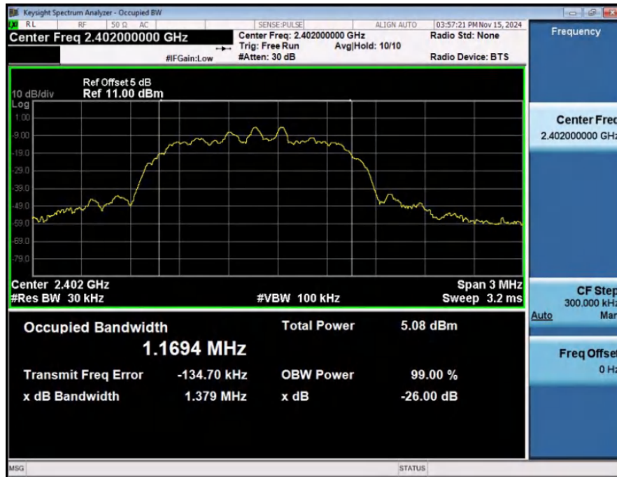
99%_Occupied_Bandwidth_NVNT_ANT1_2-DH5_2402_00
