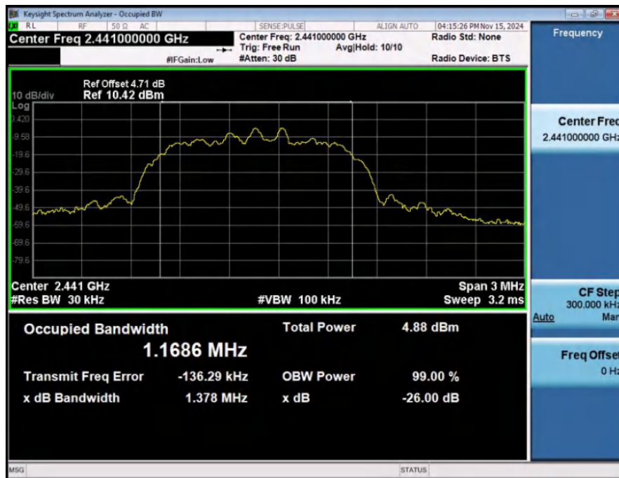
99%_Occupied_Bandwidth_NVNT_ANT1_2-DH5_2441_00
