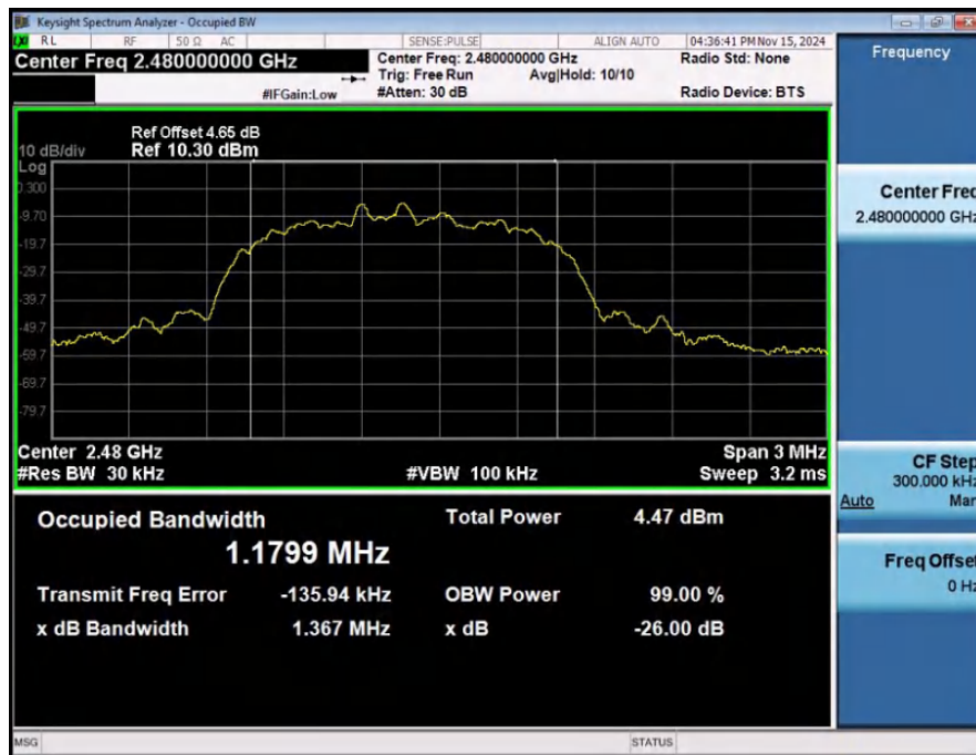
99%_Occupied_Bandwidth_NVNT_ANT1_3-DH5_2480_00
