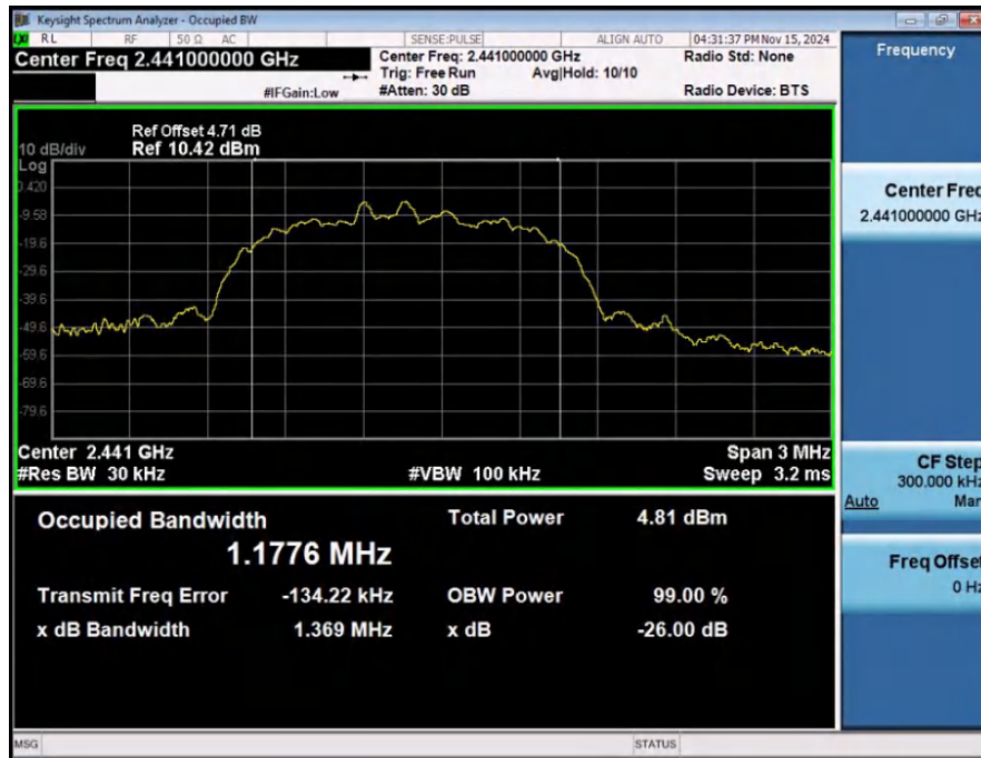
99%_Occupied_Bandwidth_NVNT_ANT1_3-DH5_2441_00
