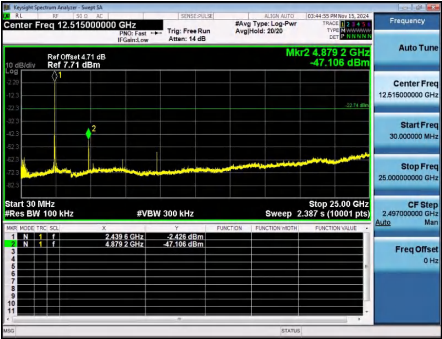
2_Spurious_Emissions_NVNT_ANT1_1-DH5_2441_00
