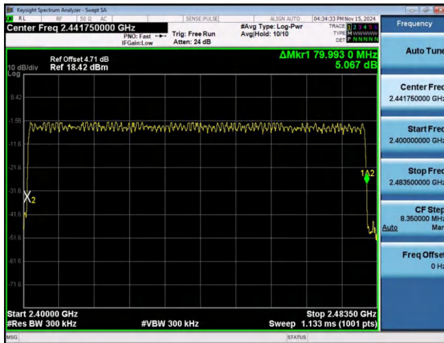
Number_of_Hopping_Channel_(Hopping)_NVNT_ANT1_3-DH5_Hopping
