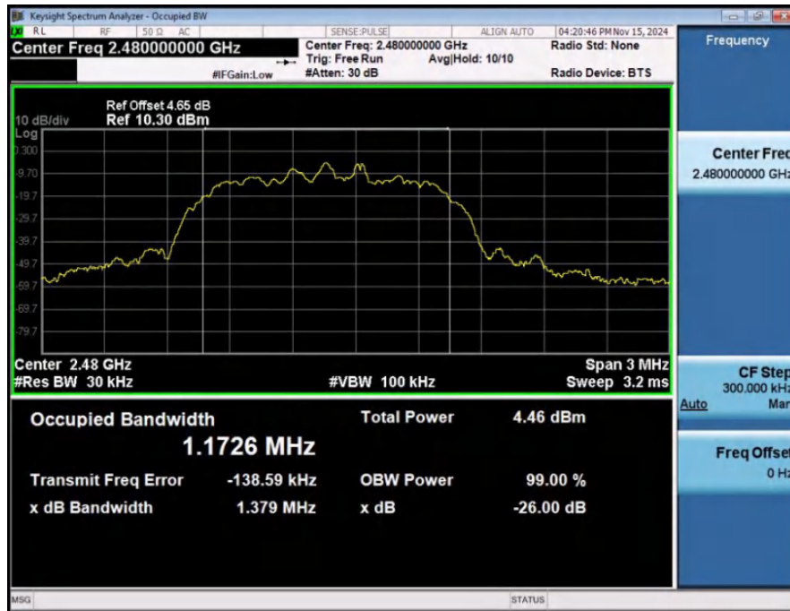
99%_Occupied_Bandwidth_NVNT_ANT1_2-DH5_2480_00
