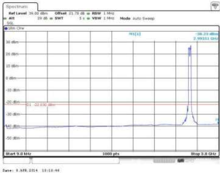
Figure 173 Spurious Emissions (9kHz – 3GHz) – 16QAM (2583.0/2603.0 MHz) (20MHz Channel BW)
