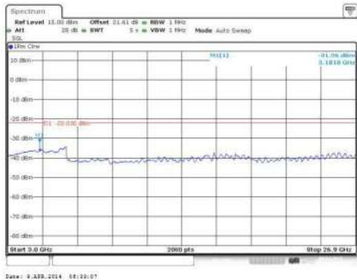
Figure 214 Spurious Emissions (3GHz – 26.900GHz) – 64QAM (2583.0/2603.0 MHz) (20MHz Channel BW)
