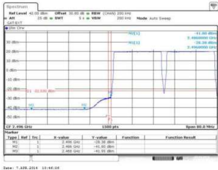
Figure 215 Spurious Emissions (Lower Band Edge) – QPSK (2506.0/2526.0 MHz) (20MHz Channel BW)
