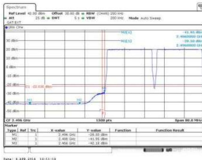
Figure 167 Spurious Emissions (Lower Band Edge) – QPSK (2506.0/2526.0 MHz) (20MHz Channel BW)
