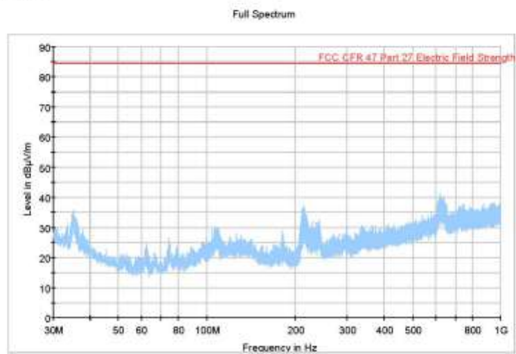
Figure 237 Radiated Emission 30 MHz – 1 GHz (2506 MHz) (20MHz Channel BW)
