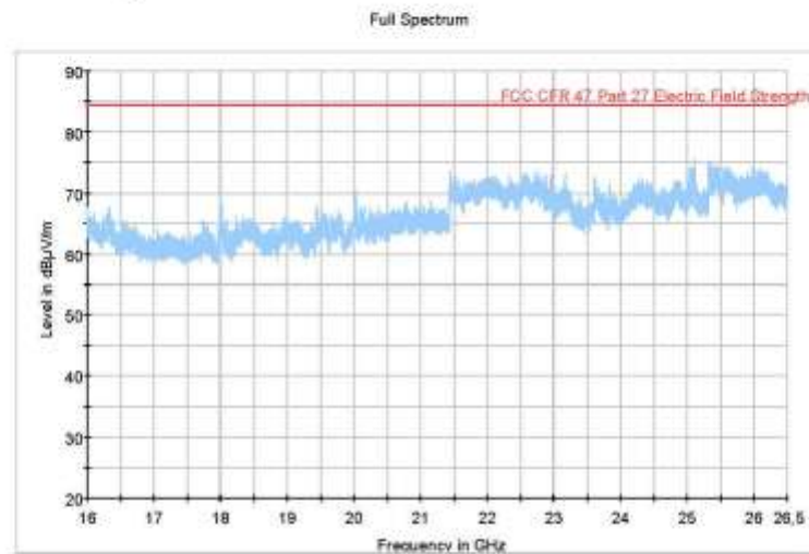
Figure 236 Radiated Emission 16 GHz – 26.5 GHz (2680 MHz) (20MHz Channel BW)
