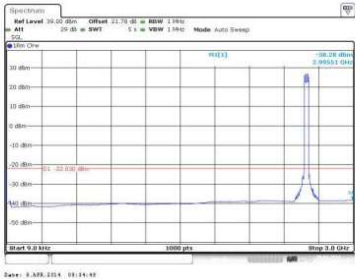
Figure 213 Spurious Emissions (9kHz – 3GHz) – 64QAM (2583.0/2603.0 MHz) (20MHz Channel BW)
