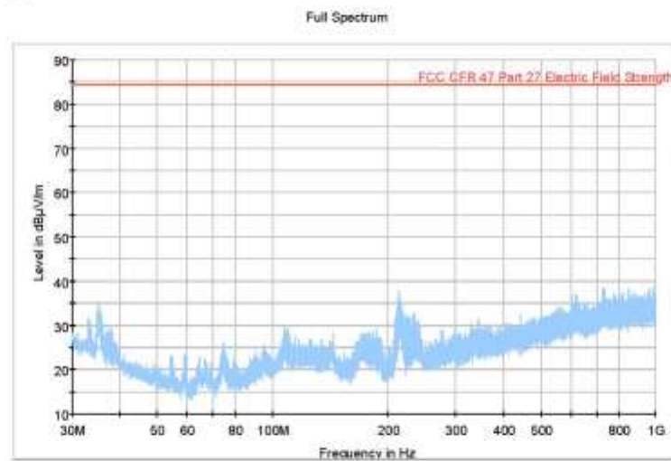
Figure 228 Radiated Emission 30 MHz – 1 GHz (2506 MHz) (20MHz Channel BW)
