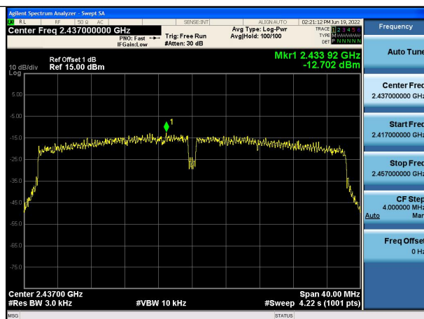
Test Mode:802.11n HT40 2437MHz Chain0
