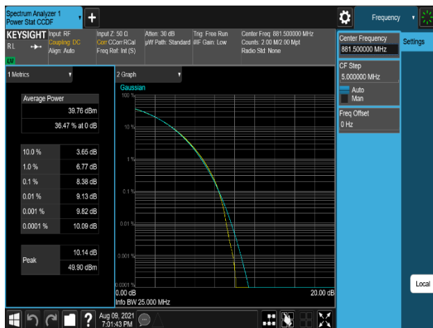
Plot 7-293. Peak To Average Power Ratio Plot (DSS_B5_10M+10M+5M_3C_64QAM - Port 3)
