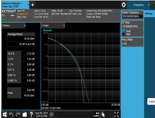
Plot 7-285. Peak To Average Power Radio Plot (DSS_B5_10M+5M_2C_64QAM - Low Channel, Port 3)
