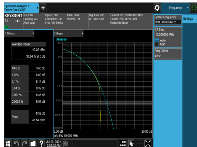
Plot 7-271. Peak To Average Power Radio Plot (LTE_B5_10M_1C_256QAM - High Channel, Port 0)
