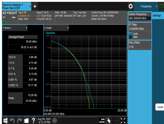
Plot 7-291. Peak To Average Power Ratio Plot (DSS_B5_10M+10M+5M_3C_QPSK - Port 3)
