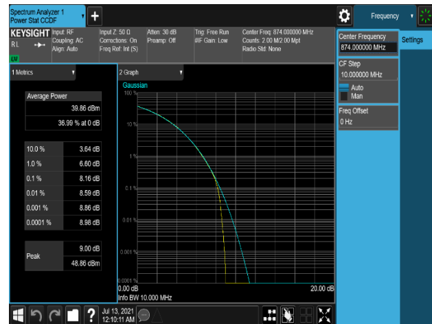
Plot 7-269. Peak To Average Power Radio Plot (LTE_B5_10M_1C_256QAM - Low Channel, Port 0)
