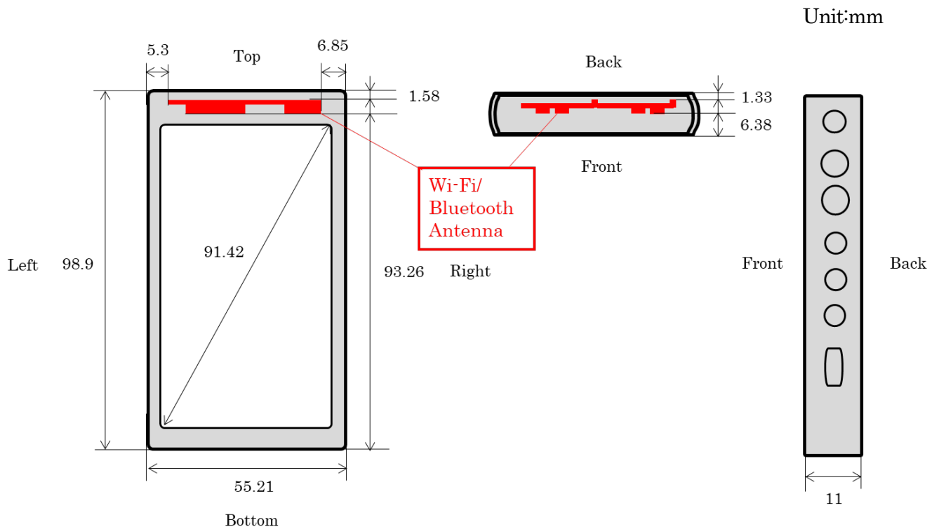
Figure D-4 Antenna Dimensions and Separation Distances
