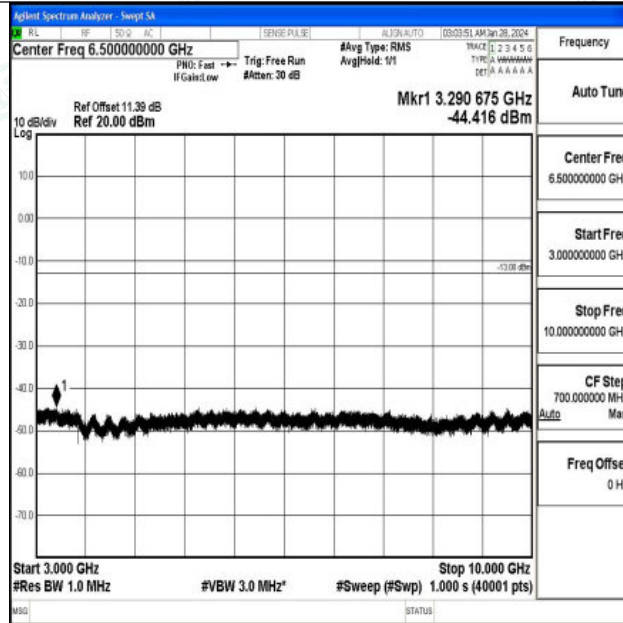
Band5_10MHz_QPSK_20525_1RB#0_3000~10000_3000~10000
