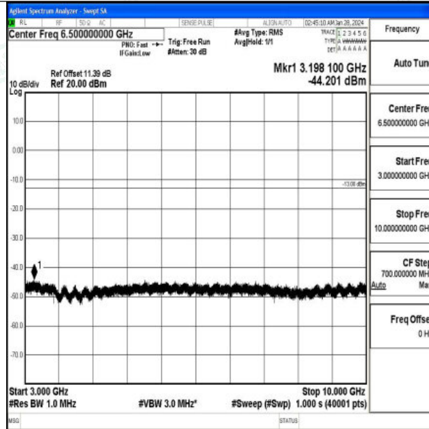
Band5_5MHz_QPSK_20625_1RB#0_3000~10000_3000~10000
