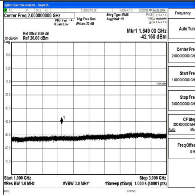
Band5_10MHz_16QAM_20450_1RB#0_1000~3000_1000~3000
