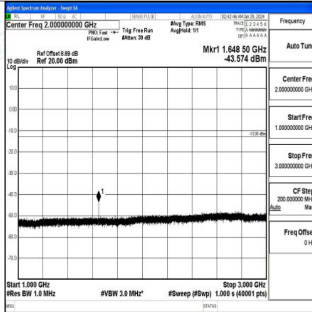
Band5_5MHz_16QAM_20425_1RB#0_1000~3000_1000~3000
