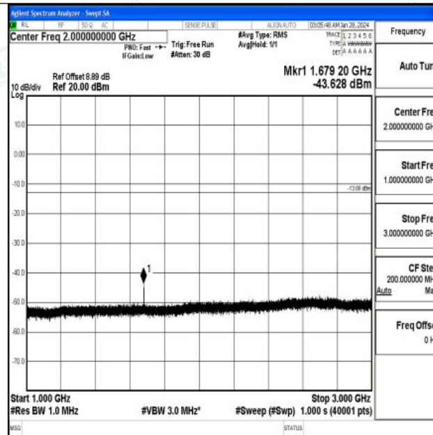
Band5_10MHz_16QAM_20600_1RB#0_1000~3000_1000~3000
