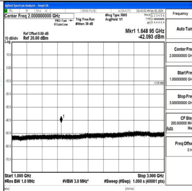
Band5_5MHz_QPSK_20425_1RB#0_1000~3000_1000~3000
