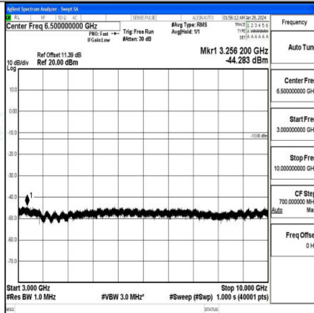
Band5_1.4MHz_16QAM_20525_1RB#0_3000~10000_3000~10000
