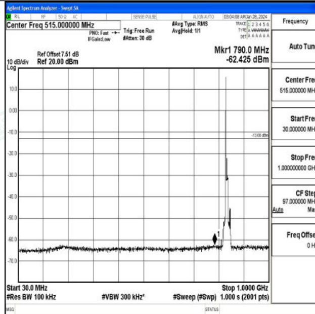
Band5_10MHz_16QAM_20525_1RB#0_30~1000_30~1000
