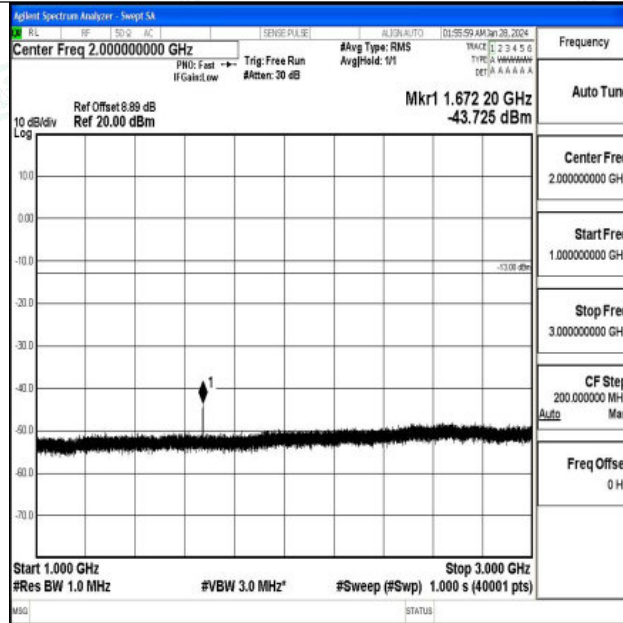
Band5_1.4MHz_16QAM_20525_1RB#0_1000~3000_1000~3000
