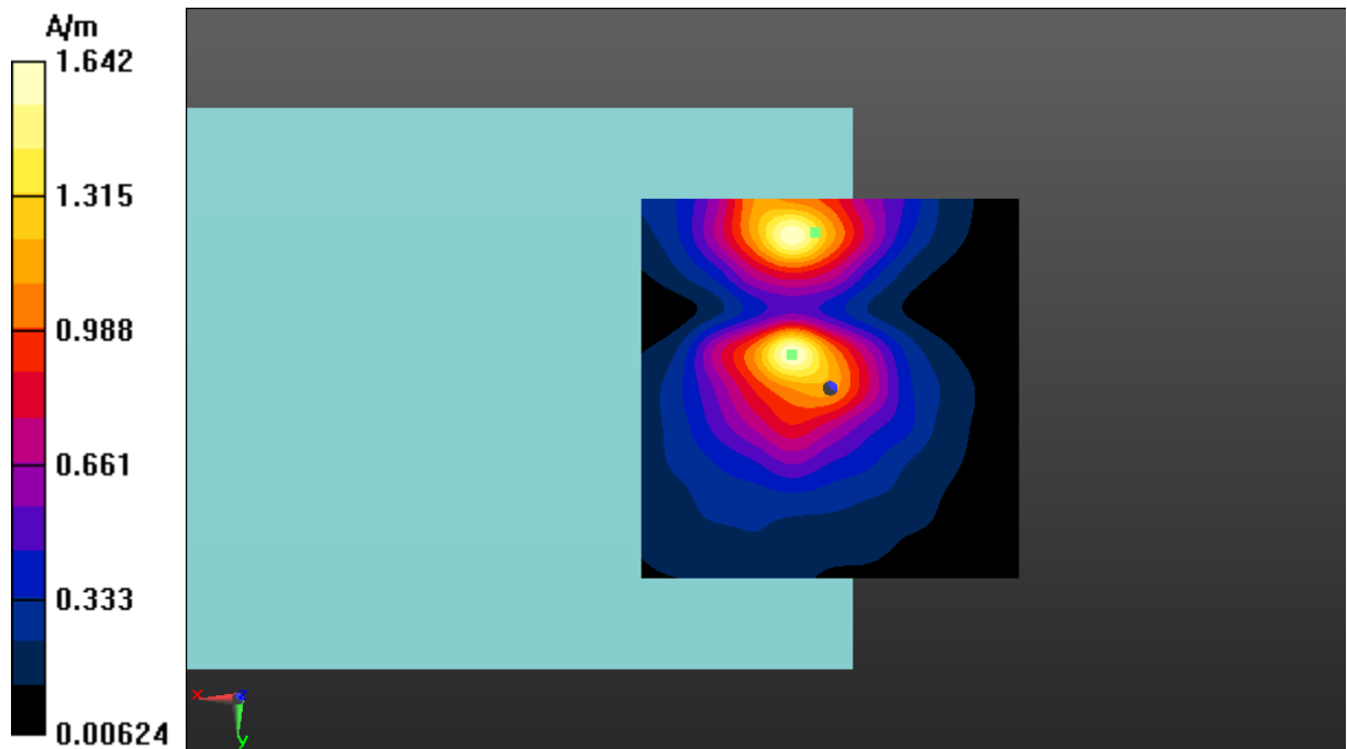
Fig A.41 T-Coil LTE-Band 41-Y
