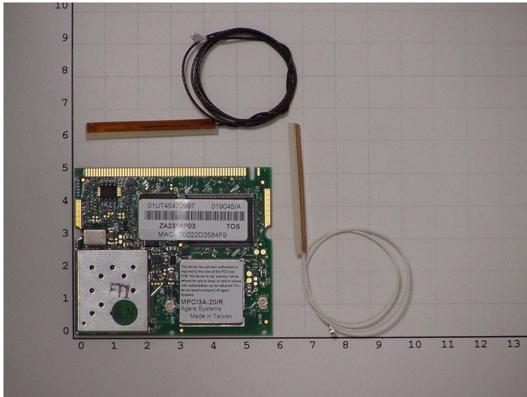
Front view Module with Stick on Antenna
