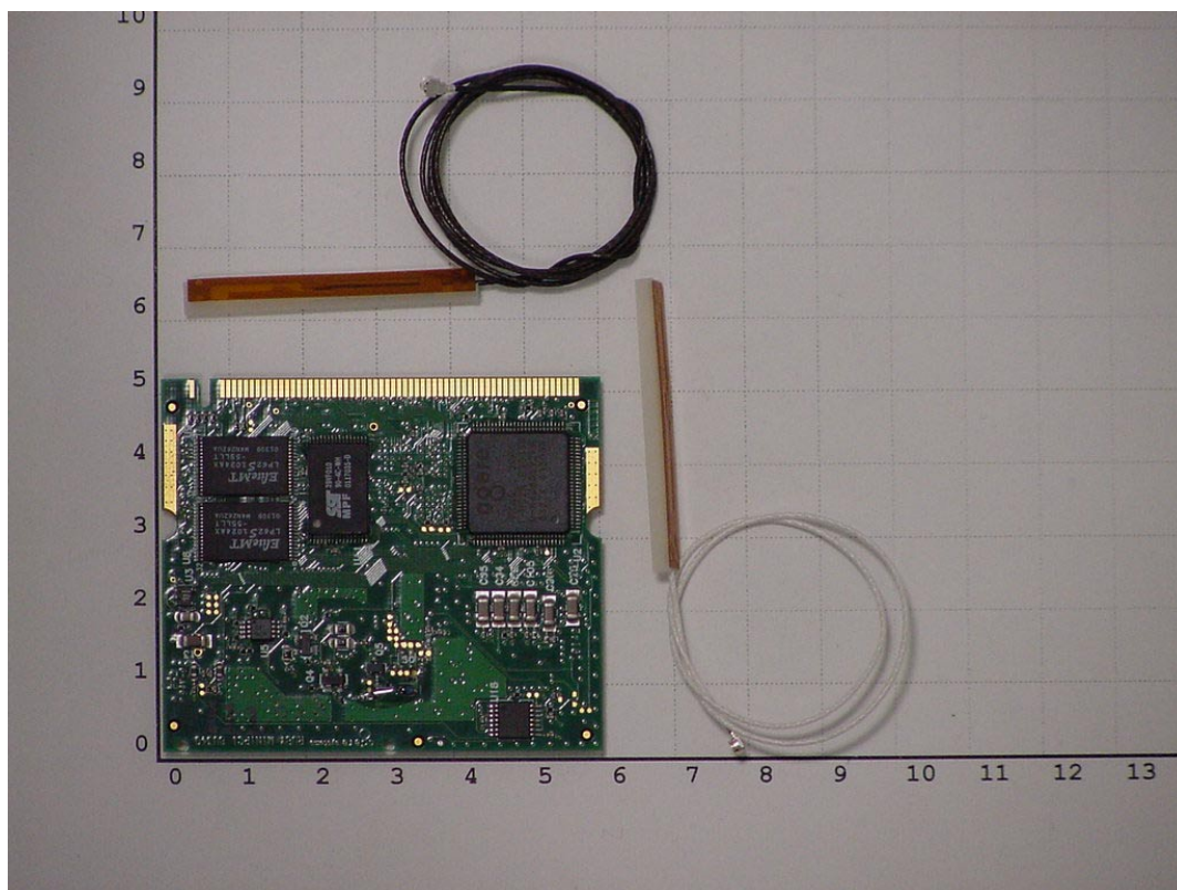
Rear view Module with Stick on Antenna
