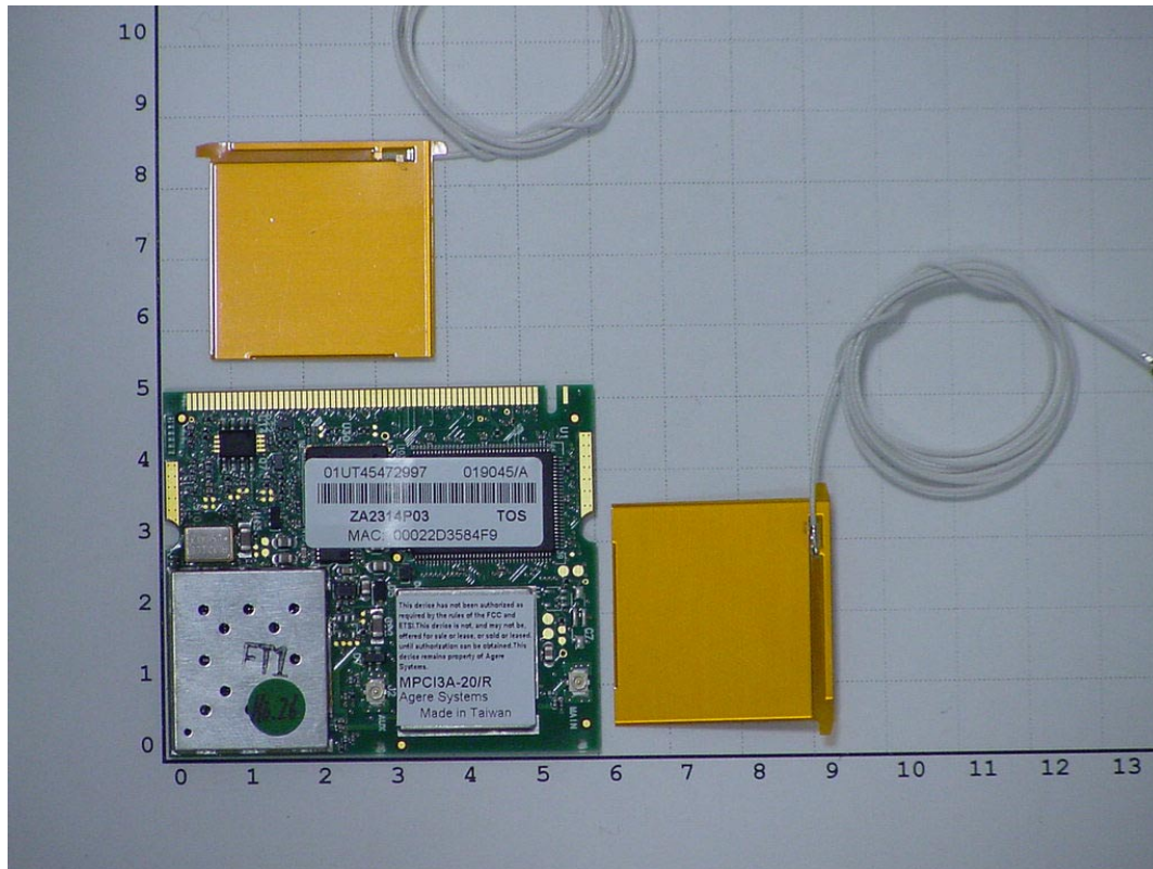
Front view Module with Film Antenna
