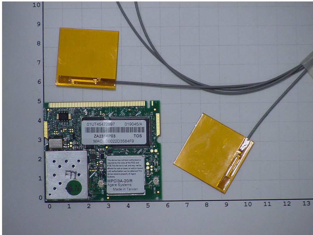
Front view Module with Dual Film Antenna
