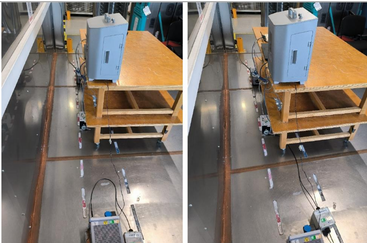
Photo of AC Power Line Conducted Emissions
