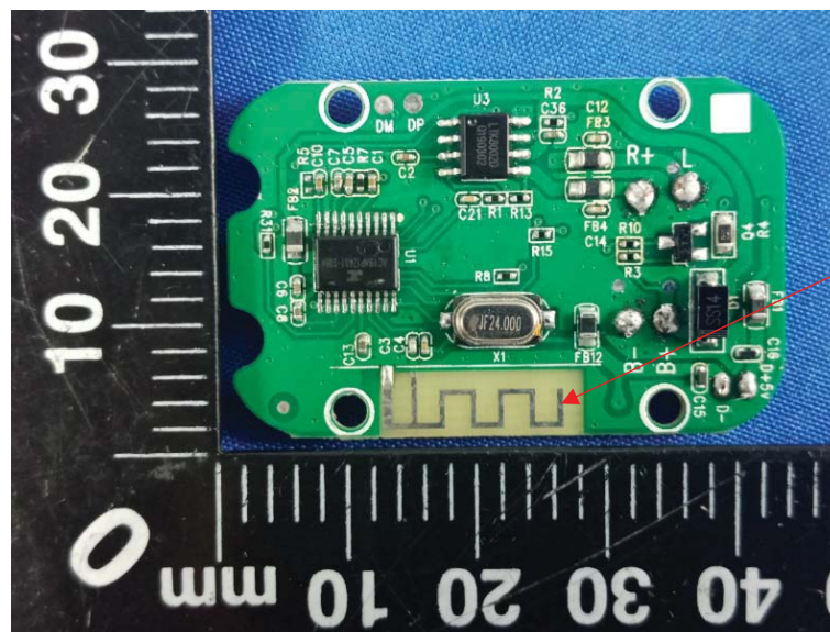
BT Antenna
