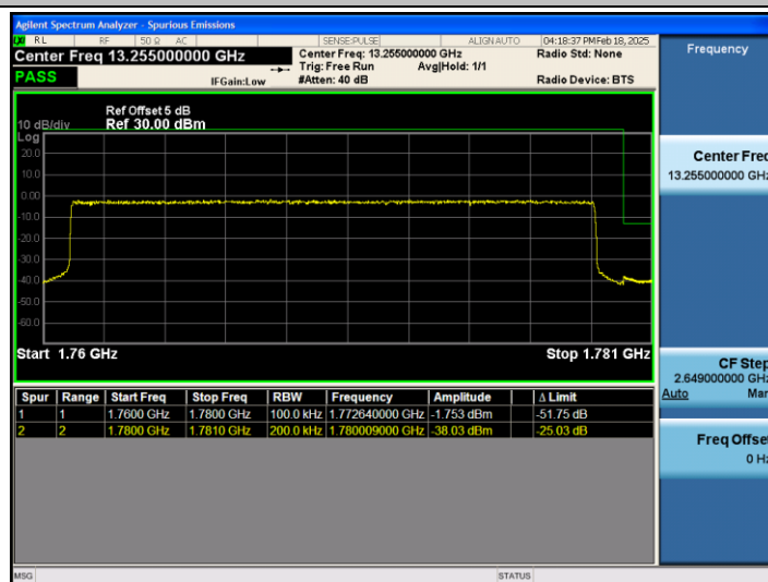
Band66_20MHz_QPSK_132572_100RB#0
