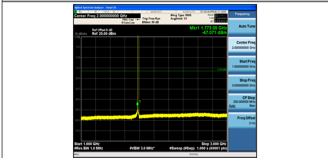
Band66_1.4MHz_QPSK_132665_1RB#0_1000~3000_1000~3000
