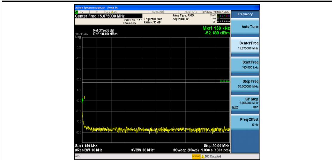
Band66_5MHz_QPSK_132647_1RB#0_0.15~30_0.15~30
