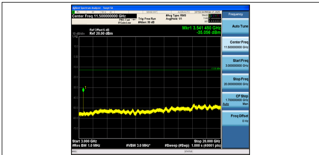
Band66_10MHz_QPSK_132622_1RB#0_3000~131022_3000~131022
