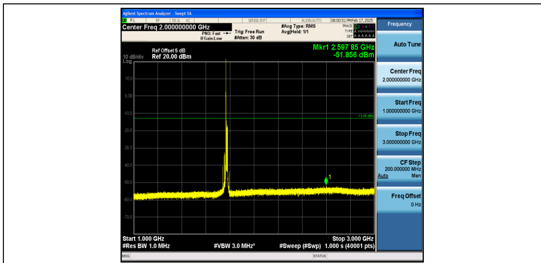
Band66_15MHz_QPSK_132597_1RB#0_1000~3000_1000~3000
