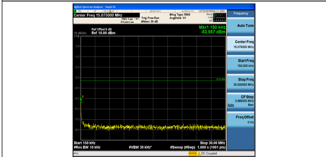
Band66_10MHz_16QAM_132622_1RB#0_0.15~30_0.15~30
