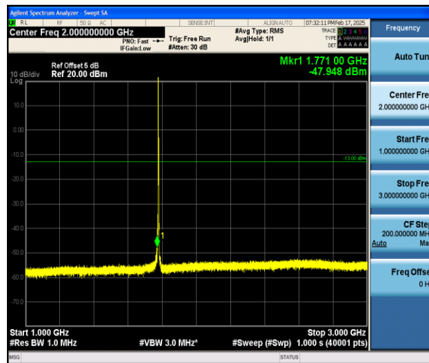
Band66_3MHz_QPSK_132657_1RB#0_1000~3000_1000~3000
