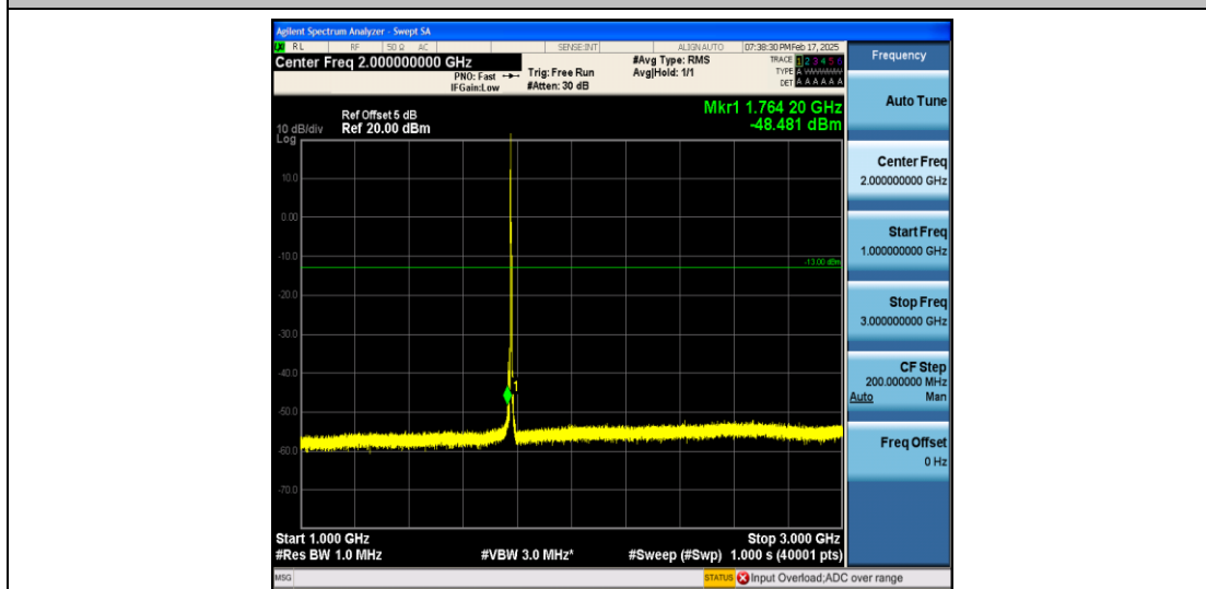
Band66_5MHz_QPSK_132647_1RB#0_1000~3000_1000~3000
