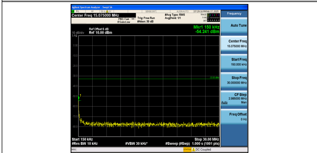
Band66_1.4MHz_16QAM_132665_1RB#0_0.15~30_0.15~30
