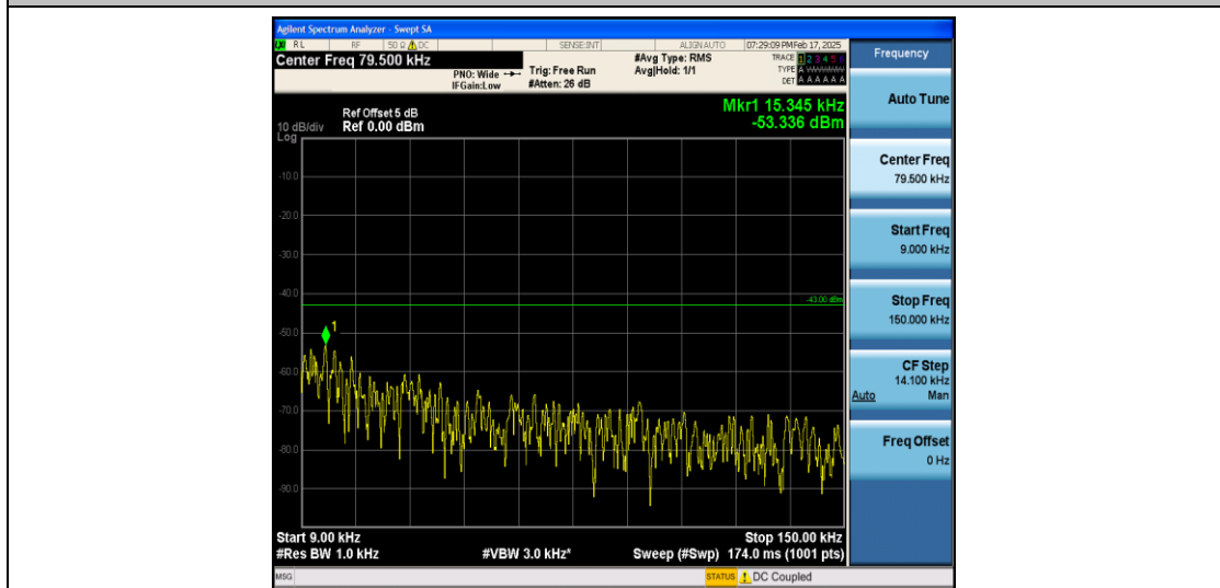
Band66_1.4MHz_16QAM_132665_1RB#0_0.009~0.15_0.009~0.15
