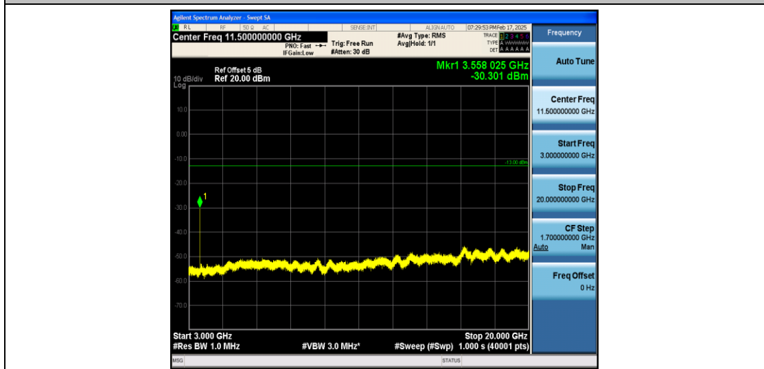
Band66_1.4MHz_16QAM_132665_1RB#0_3000~131022_3000~131022
