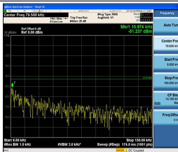
Band66_3MHz_16QAM_132657_1RB#0_0.009~0.15_0.009~0.15
