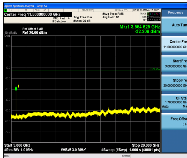
Band66_3MHz_QPSK_132657_1RB#0_3000~131022_3000~131022
