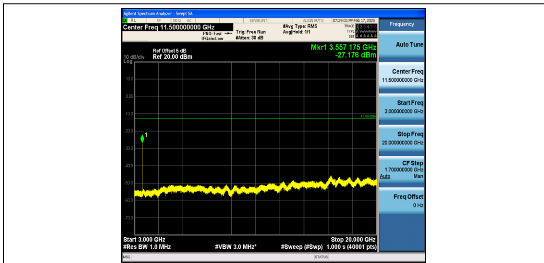
Band66_1.4MHz_QPSK_132665_1RB#0_3000~131022_3000~131022
