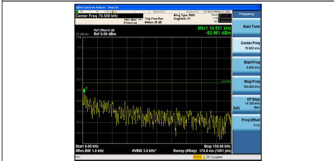
Band66_5MHz_QPSK_132647_1RB#0_0.009~0.15_0.009~0.15
