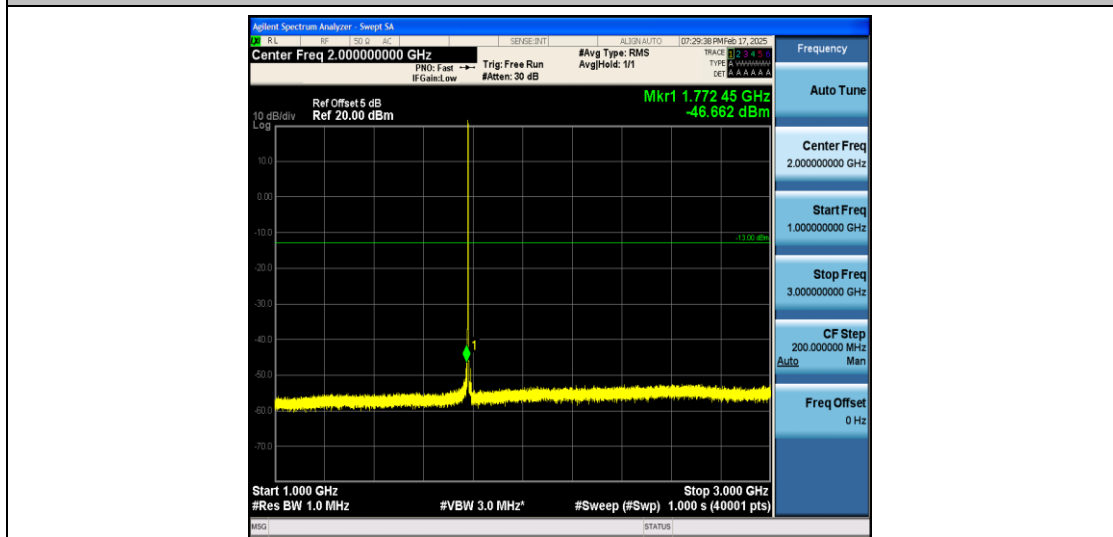
Band66_1.4MHz_16QAM_132665_1RB#0_1000~3000_1000~3000
