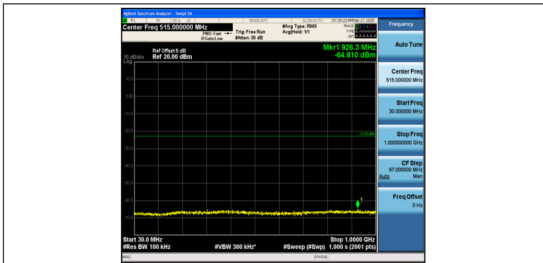
Band66_1.4MHz_16QAM_132665_1RB#0_30~1000_30~1000
