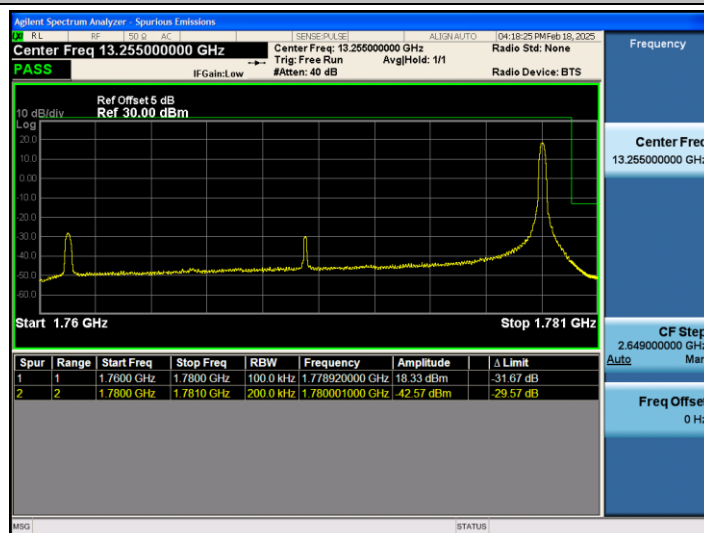
Band66_20MHz_16QAM_132572_1RB#99
