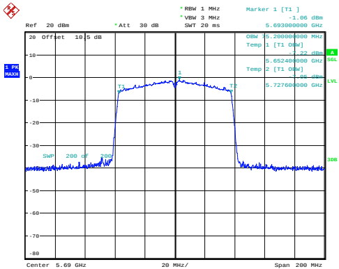
ac80_5690MHz_Chain 0 75.200MHz
