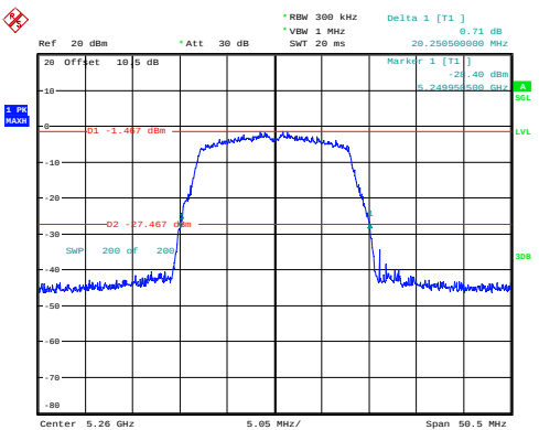
a_5260MHz_Chain 0 20.251MHz
