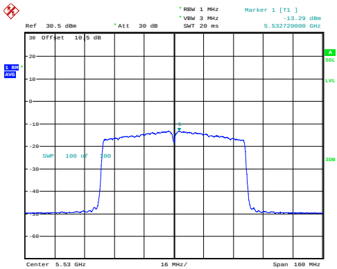
ac80_5530MHz_Chain 0 -13.29dBm/MHz
