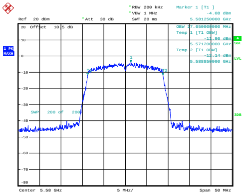
n20_5580MHz_Chain 0 17.650MHz
