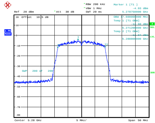
n20_5280MHz_Chain 0 17.600MHz
