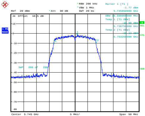
a_5745MHz_Chain 0 16.500MHz
