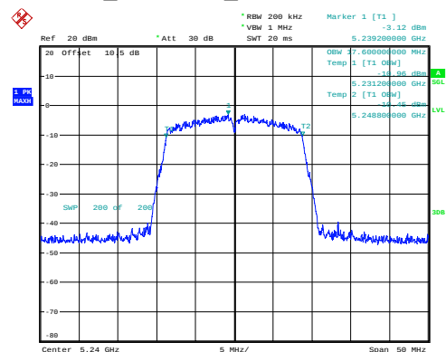
n20_5240MHz_Chain 0 17.600MHz
