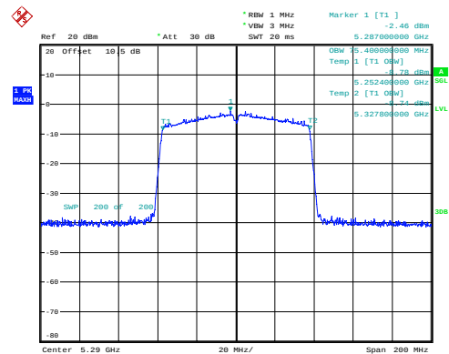
ac80_5290MHz_Chain 0 75.400MHz
