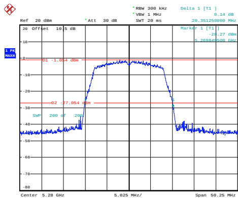
a_5280MHz_Chain 0 20.351MHz
