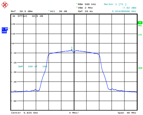
a_5825MHz_Chain 0 -7.62dBm/MHz
