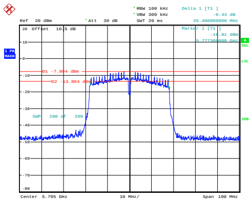
n40_5795MHz_Chain 0 35.400MHz
