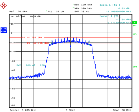
n20_5785MHz_Chain 0 15.400MHz
