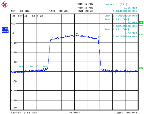
ac80_5610MHz_Chain 0 75.400MHz
