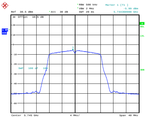
a_5745MHz_Chain 0 -5.99dBm/MHz
