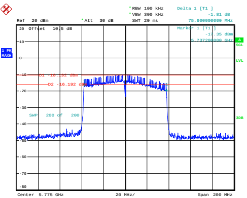
ac80_5775MHz_Chain 0 75.600MHz
