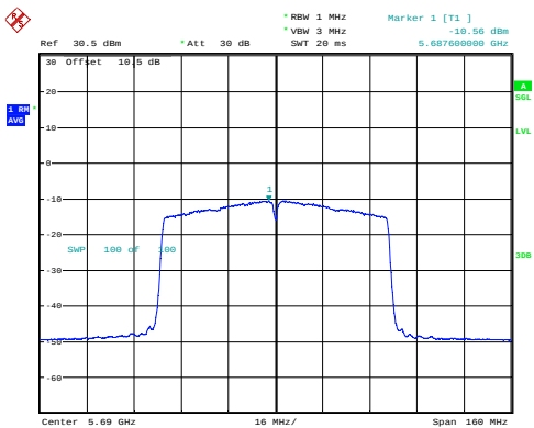
ac80_5690MHz_Chain 0 -10.56dBm/MHz
