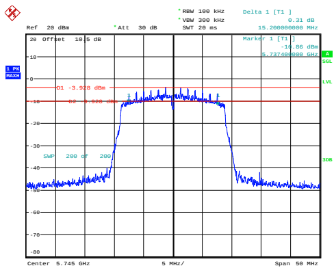
n20_5745MHz_Chain 0 15.200MHz
