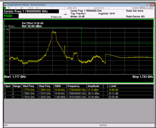
Band66-1.4MHz-QPSK-132665-6RB#0
