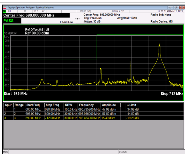
Band12-10MHz-64QAM-23130-1RB#0
