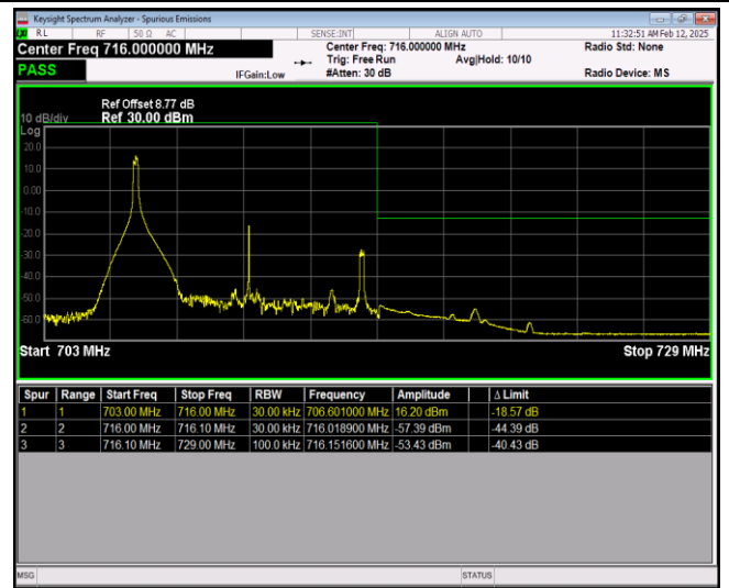
Band12-10MHz-16QAM-23130-50RB#0
