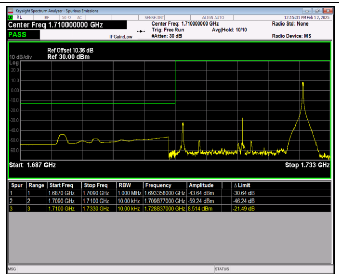
Band66-20MHz-64QAM-132572-1RB#0
