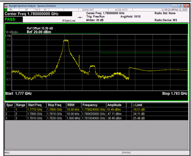
Band66-1.4MHz-64QAM-132665-6RB#0
