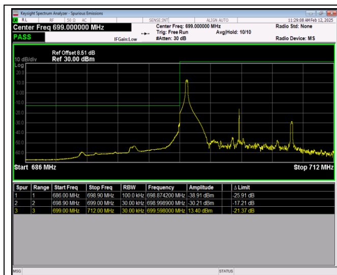
Band12-10MHz-64QAM-23060-50RB#0
