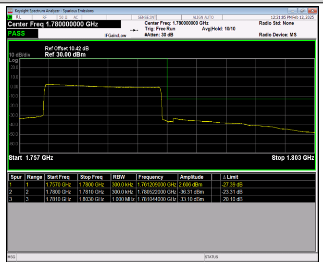
Band66-20MHz-64QAM-132572-100RB#0
