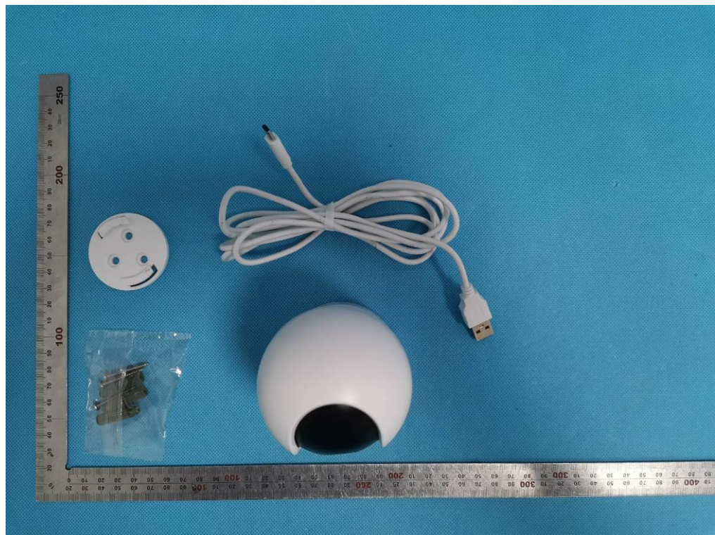
Model: C516 All view of EUT
