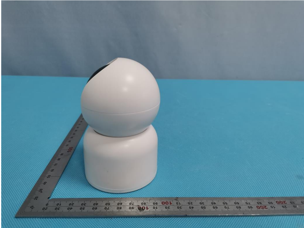
Model: C528 All view of EUT
