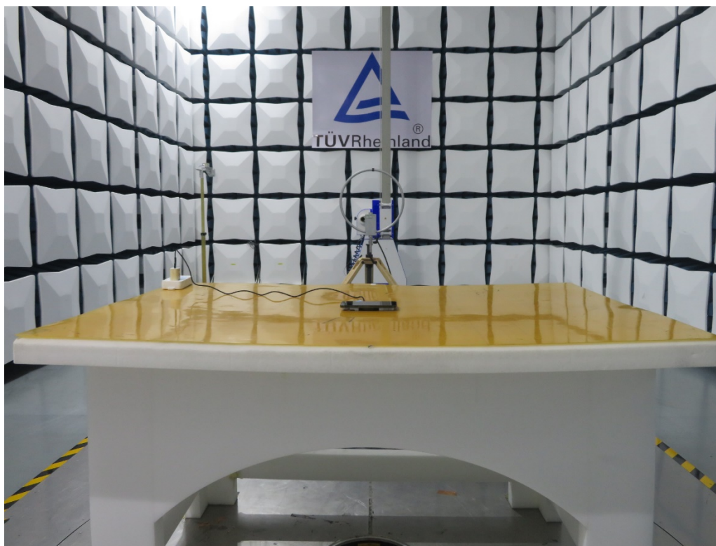
Photograph 1: Set-up for Radiated Spurious Emission, Below 30MHz
