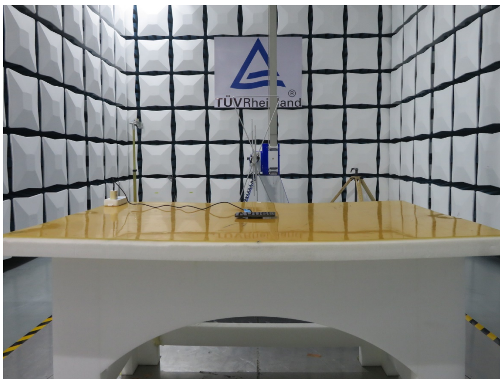
Photograph 2: Set-up for Radiated Spurious Emission, Above 30MHz
