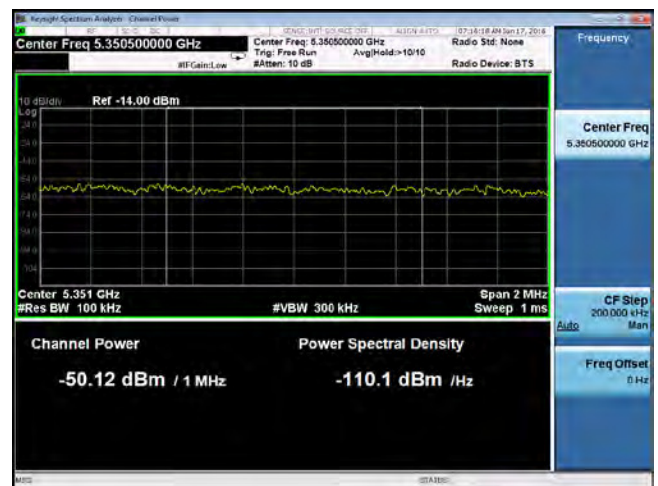
Band Edge-802.11n20 5320 MHz (Limit: -27dBm/MHz eirp)
