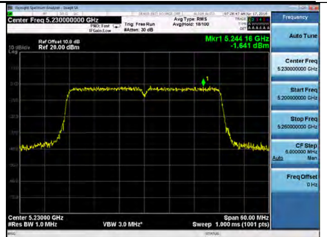
PSD-802.11n-40M 5230MHz
