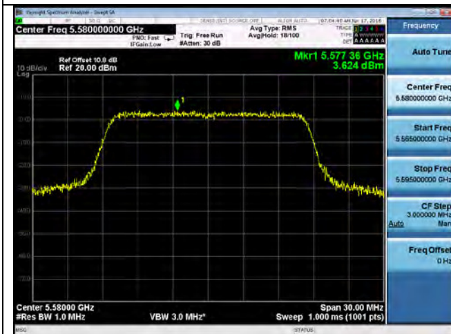
PSD-802.11a 5580MHz
