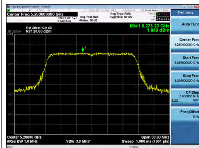
PSD-802.11a 5280MHz
