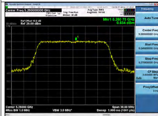
PSD-802.11a 5260MHz
