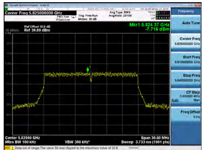
PSD-802.11n-20M 5825MHz
