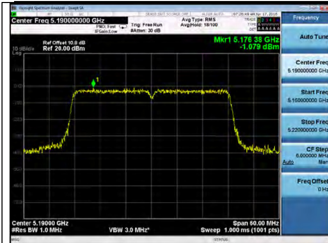
PSD-802.11n-40M 5190MHz
