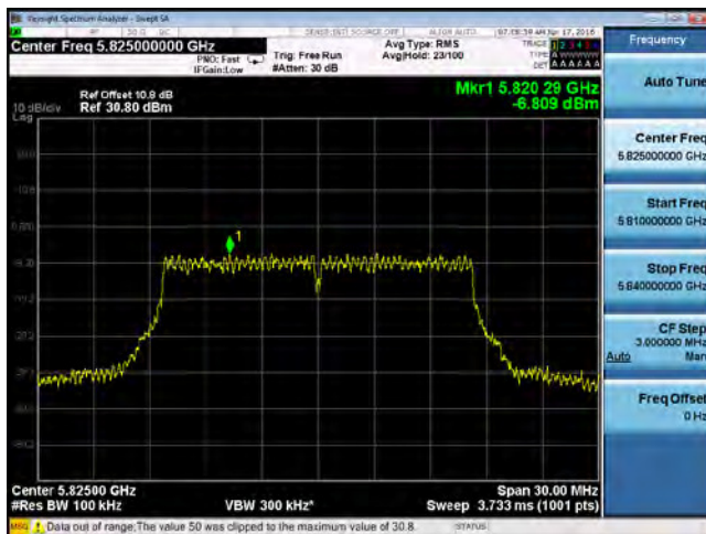
PSD-802.11a 5825MHz
