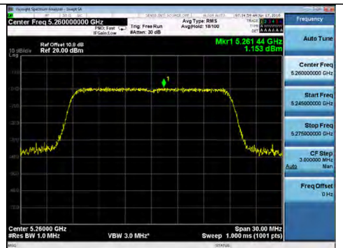
PSD-802.11n-20M 5260MHz
