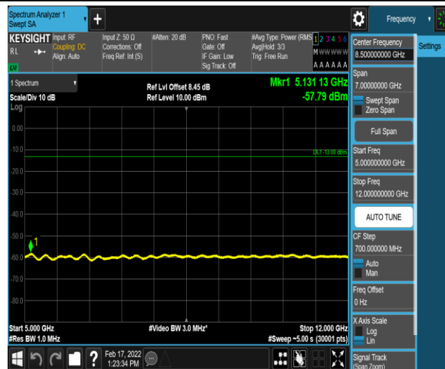
Band26-15MHz-16QAM-26865-1-0-Low-5000-12000--57.79-PASS
