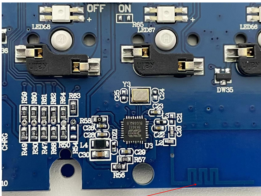
PCB ANTENNA
