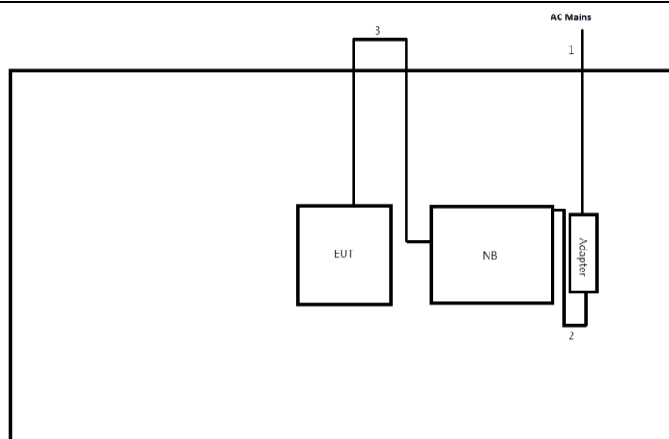
Test Setup Diagram - Radiated Test (Mode 1)
