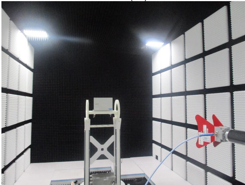
18 - 40 GHz REAR TEST PHOTO (3m)
