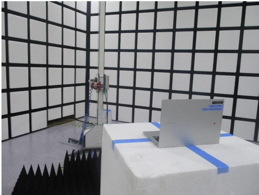
1 - 18 GHz REAR TEST PHOTO
