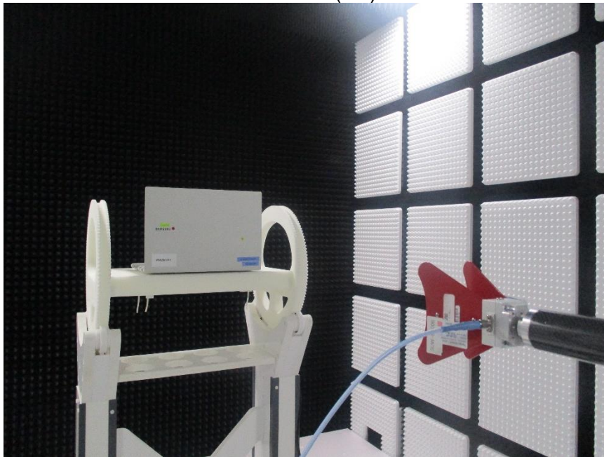
18 - 40 GHz FRONT TEST PHOTO (1m)
