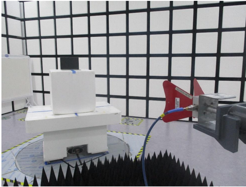
1 - 18 GHz FRONT TEST PHOTO
