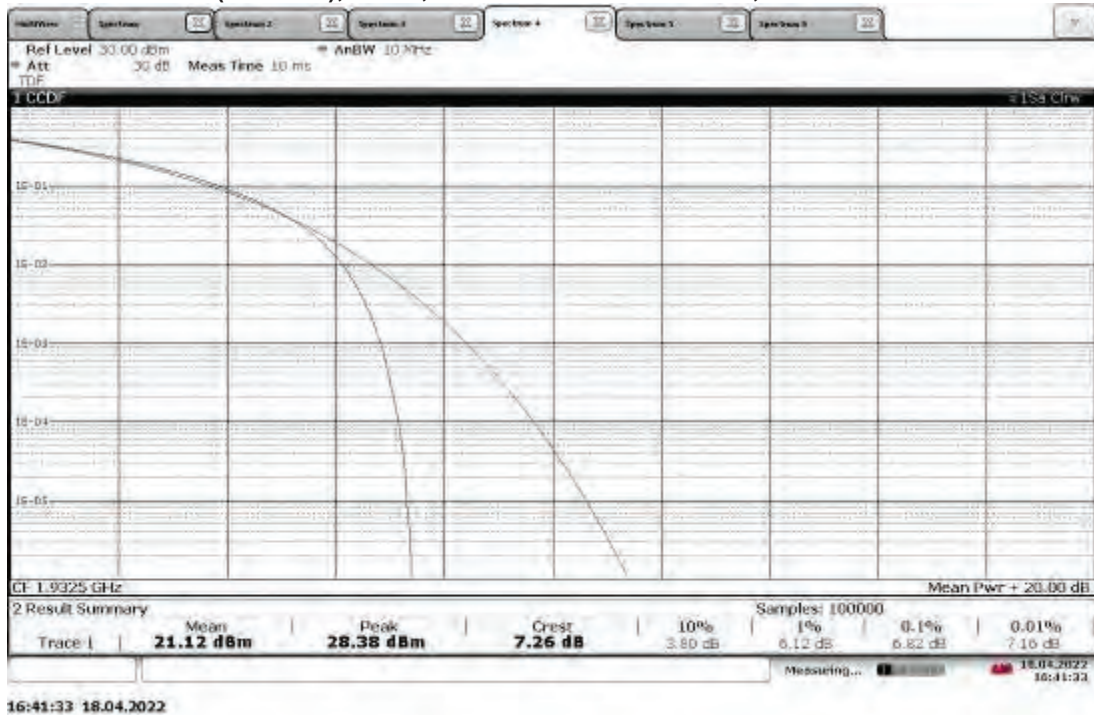
TM1.1-QPSK_5 MHz Bandwidth (4G LTE) Slot 0 (Band 25), ANT1, Low Channel 1932.5 MHz, PAPR = 7.26 dB
