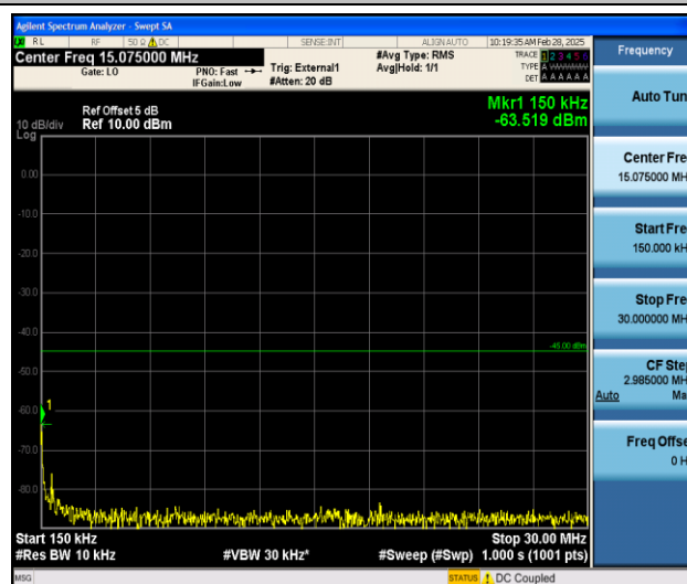
Band41_5MHz_16QAM_41565_1RB#0_0.15~30_0.15~30
