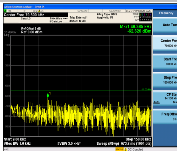
Band41_10MHz_QPSK_41540_1RB#0_0.009~0.15_0.009~0.15
