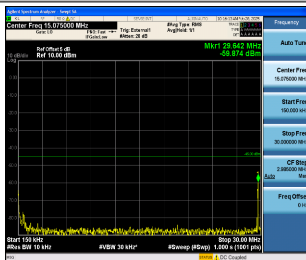
Band41_5MHz_QPSK_40620_1RB#0_0.15~30_0.15~30
