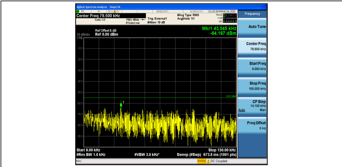
Band41_10MHz_16QAM_40620_1RB#0_0.009~0.15_0.009~0.15
