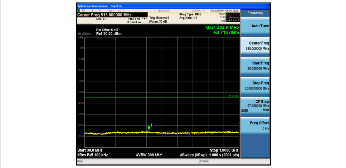
Band41_10MHz_16QAM_40620_1RB#0_30~1000_30~1000
