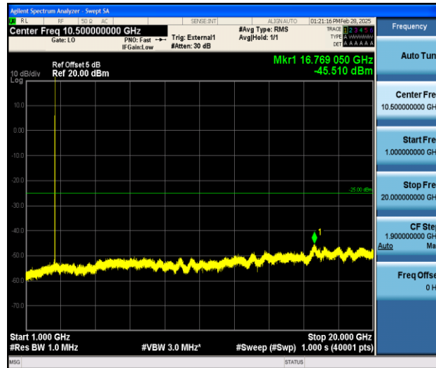
Band41_10MHz_16QAM_40620_1RB#0_1000~20000_1000~20000
