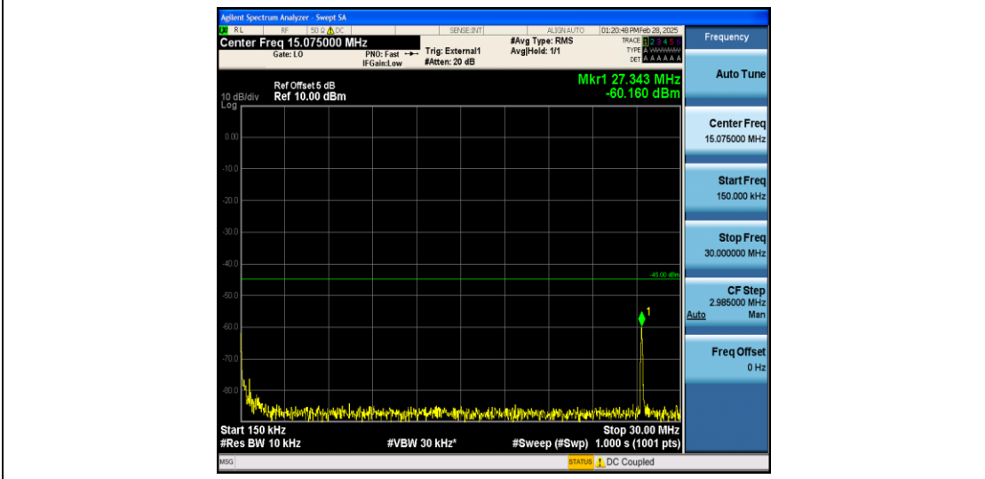
Band41_10MHz_16QAM_40620_1RB#0_0.15~30_0.15~30
