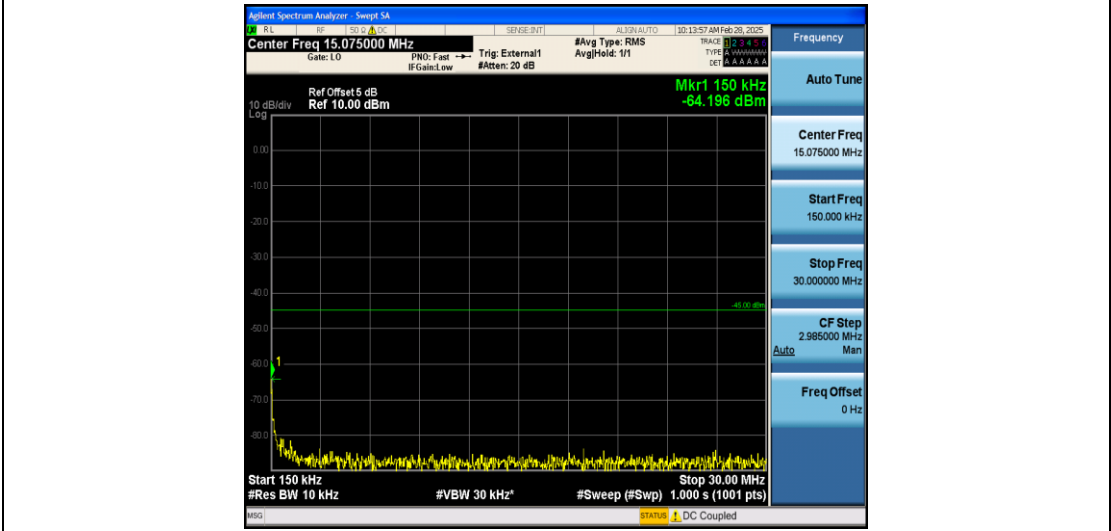
Band41_5MHz_QPSK_39675_1RB#0_0.15~30_0.15~30
