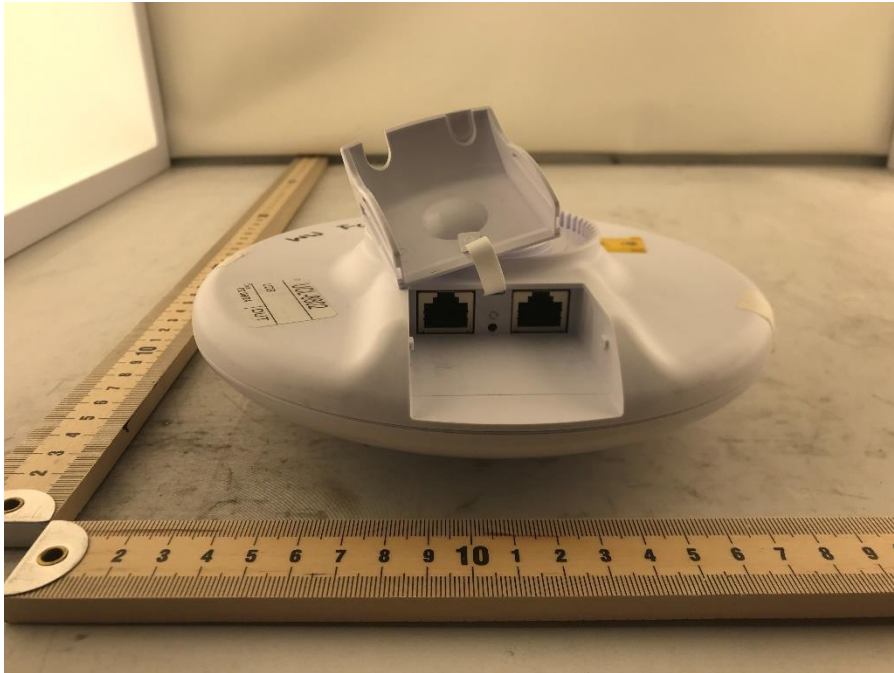
Photograph 11: Bottom Port View of DUT
