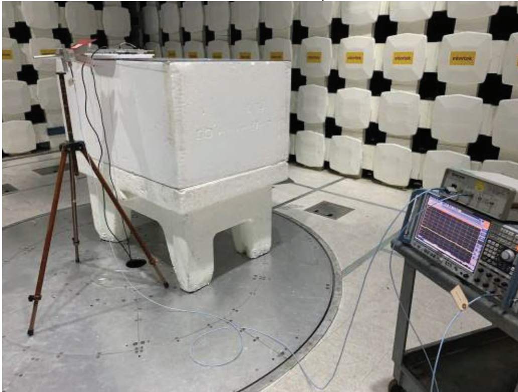
13-18 GHz Test Setup
