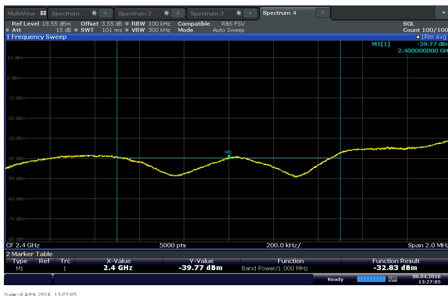
Bluetooth LE Low Channel (2402 MHz). Limit is -22.53dBm. Margin is -10.3dB. (The highest level of the desired power in the 100 kHz bandwidth within the band is 7.47dBm)
